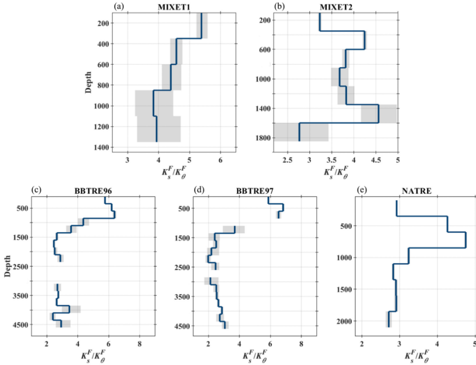
Fig. 16. Vertical profiles of depth-bin mean K_{\theta S}^F / K_{\theta S}^F based on salt finger patches for the five projects. The dark blue curves are the mean K_{\theta S}^F / K_{\theta S}^F , and the gray shadings are 95% bootstrapped confidence intervals. To exclude the influence of extreme values, we only consider patches with \Gamma_{\theta}^F between its upper and lower quartiles for each depth bin. The depth-bin size is 250 m; and depth bins with number of patches smaller than 10 are excluded.
