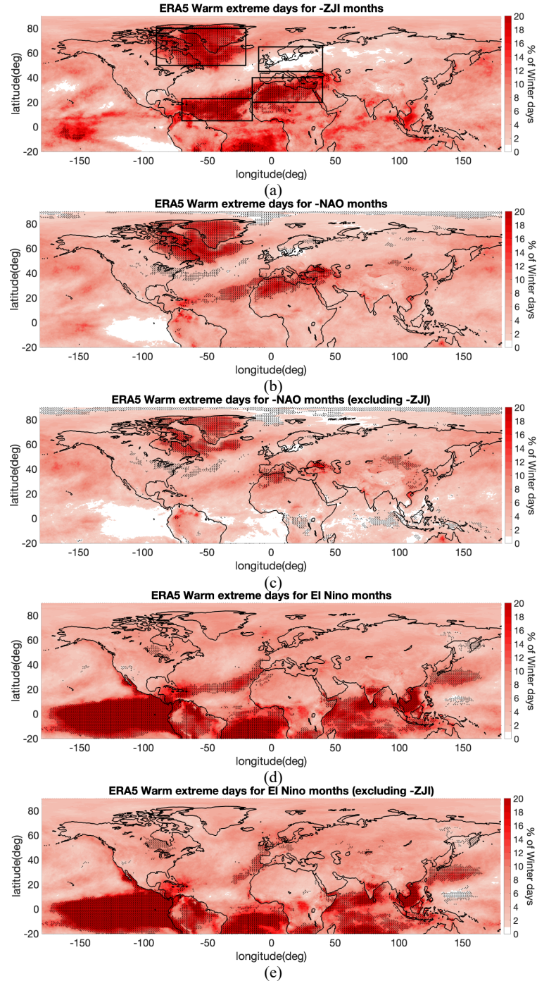
Figure 1. The distribution of the percentage of warm extreme days for (a) merged jet winter months (b) negative-NAO -NAO winter months (c) negative-NAO -NAO winter months excluding merged jet months (d) El Nino winter months (e) El Nino winter months excluding merged jet months. The regions stippled in black (+) represents regions significant at 99% using Monte Carlo simulation.
