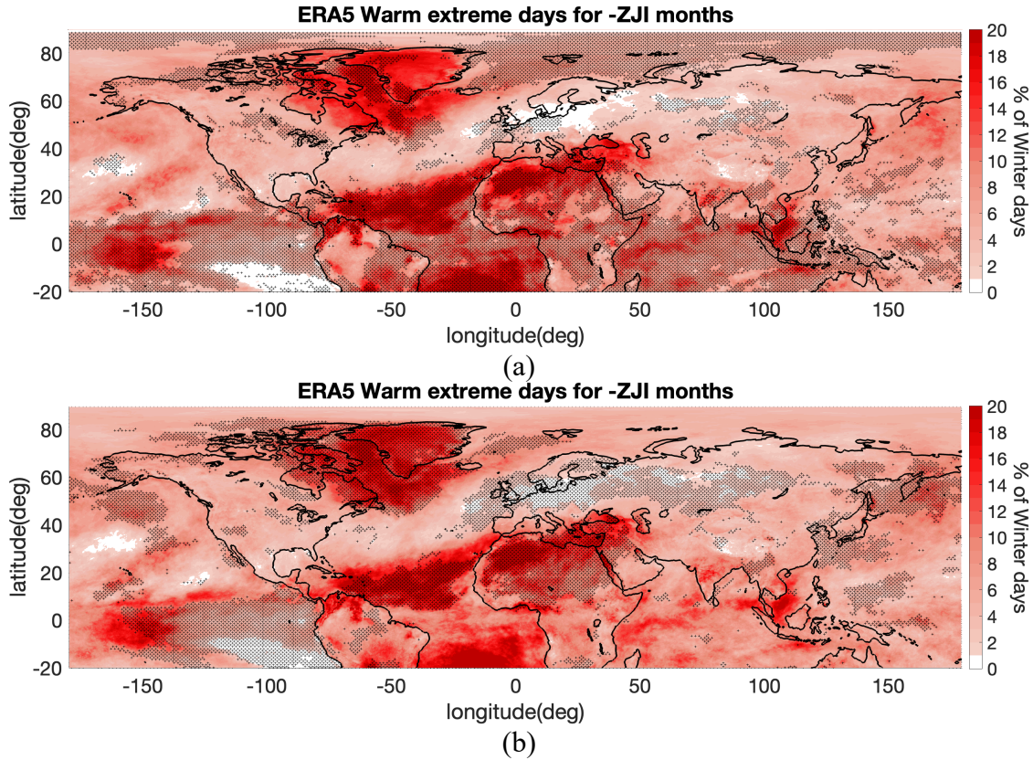
Figure 2. The distribution of the percentage of warm extreme days for merged jet winter months (same as Fig. 1a) but the regions stippled in black (+) represents regions significant at 99% using bootstrapping w.r.t. (a) -NAO months (excluding -ZJI) and (b) El Niño months (excluding -ZJI)
