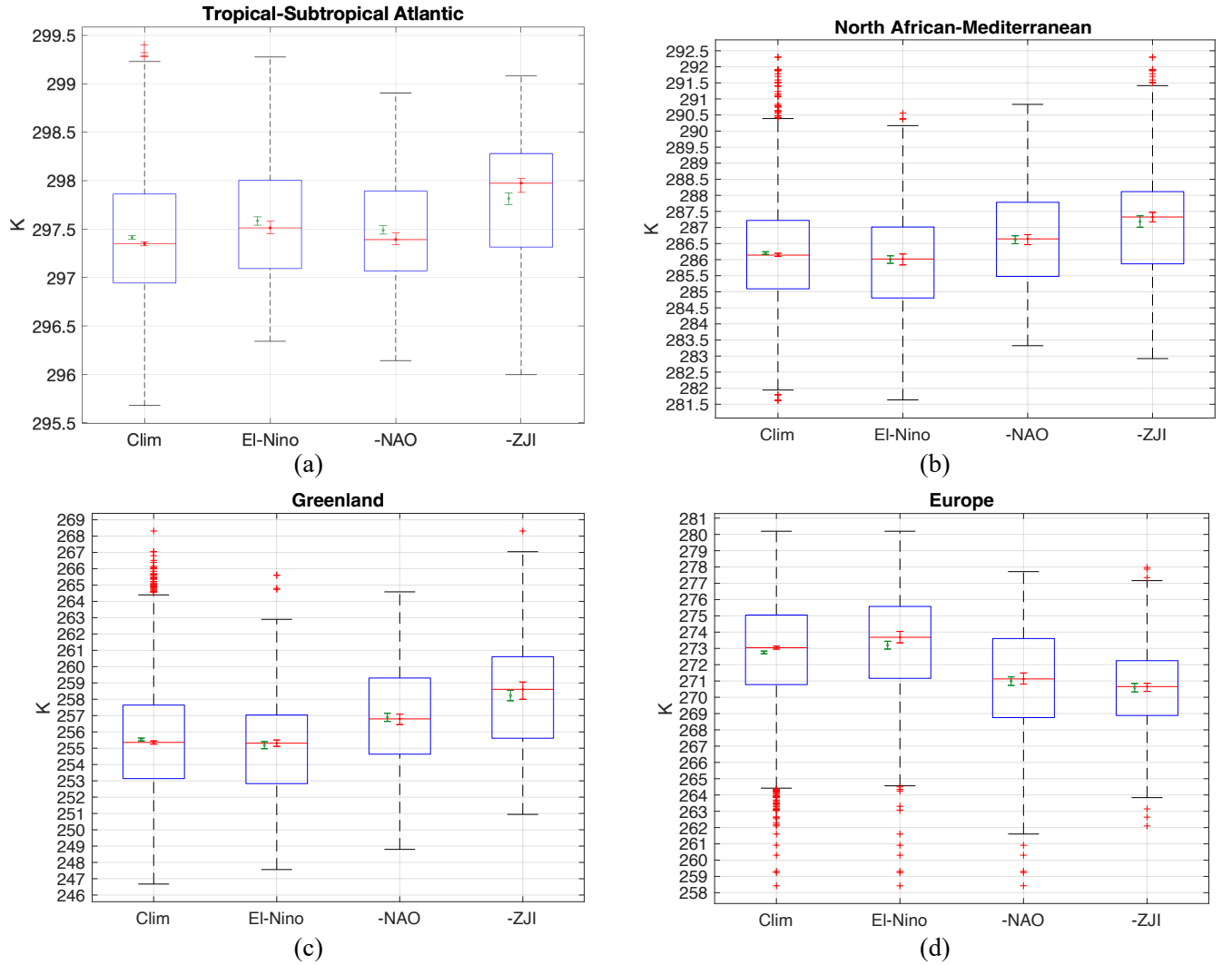
Figure 3. Box plot of daily average surface temperatures for DJF Climatology (1960-2020), El Nino months (excluding -ZJI), negative-NAO -NAO months (excluding -ZJI) and merged jet months(-ZJI) over (a) the tropical-subtropical Atlantic within the region of [5°N-23°N,70°W-15°W],(b) the North African-Mediterranean [20°N-40°N,15°W-40°E],(c)the Greenland region [50°N-80°N,90°W-20°W],(d)Europe [45°N-65°N,10°W-40°E]. These regions are marked in boxes in Fig.1a. In each box plot, the red line represents the median along with its 95% confidence interval , while the lower and upper edges of the box represent the 25th and 75th percentiles, respectively. The whiskers stretch to the furthest data points that are not deemed outliers, which are values that are more than 1.5 times the interquartile range away from the bottom or top of the box, and any outliers are depicted individually with a red (+) marker symbol. The value marked in green (+) on left half of each box represents the average-mean value along with its 95% confidence interval .
