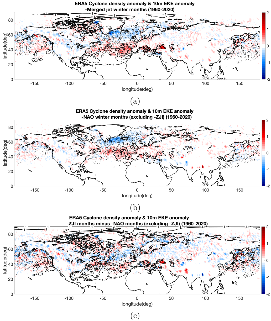
Figure 10. The cyclone density (number of cyclones per month per grid point) monthly anomaly composite during (a) merged jet winter (b) negative-NAO -NAO winter months excluding merged jet months (c) the difference of cyclone density monthly anomaly between (a) and (b). The surface eddy-kinetic energy ( m^2 s^{-2} ) anomaly is shown in contours. The positive and negative values are shown in solid and dashed lines respectively.
