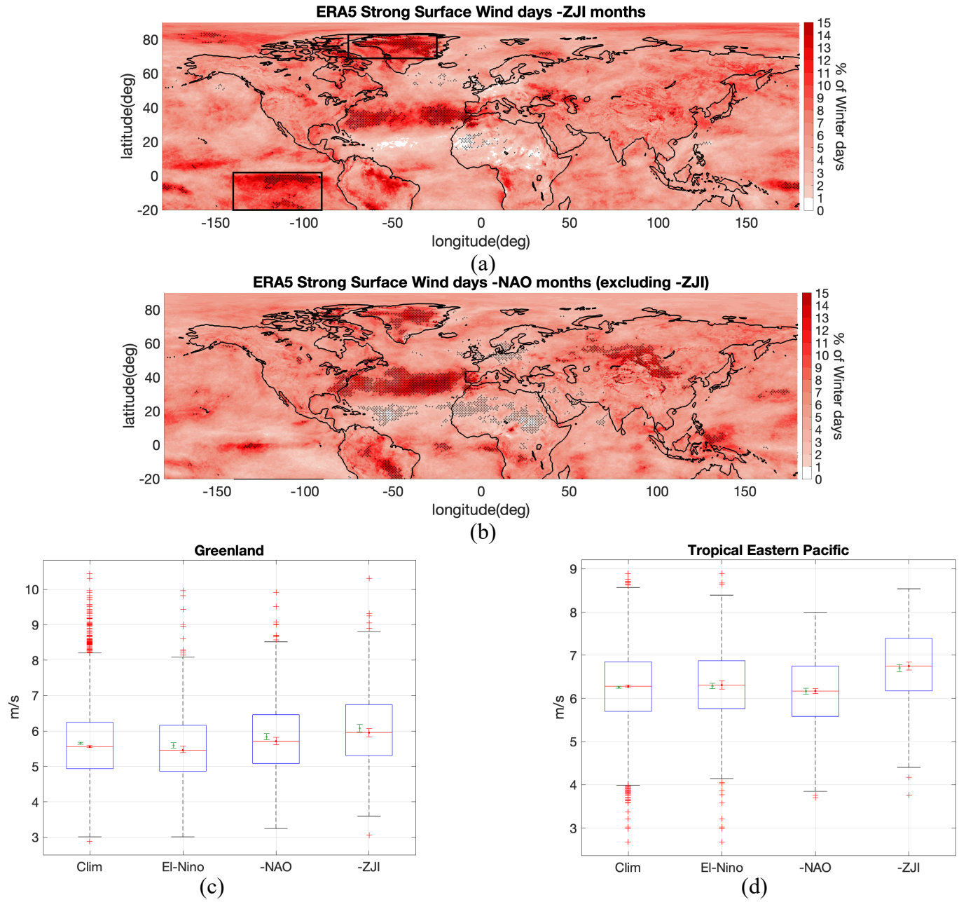
Figure 6. The distribution of the percentage of strong surface wind days for (a) merged jet winter months (b) negative NAO winter months excluding merged jet months, the regions stippled in black (+) represents regions significant at 99% using Monte Carlo simulation. Box plot, similar to Fig.3, of daily wind averaged over (c) Greenland [69°N-83°N, 75°W-25°W] (d) tropical eastern-pacific [20°S-2°N, 140°W-90°W]. These regions are marked in boxes in Fig.6a
