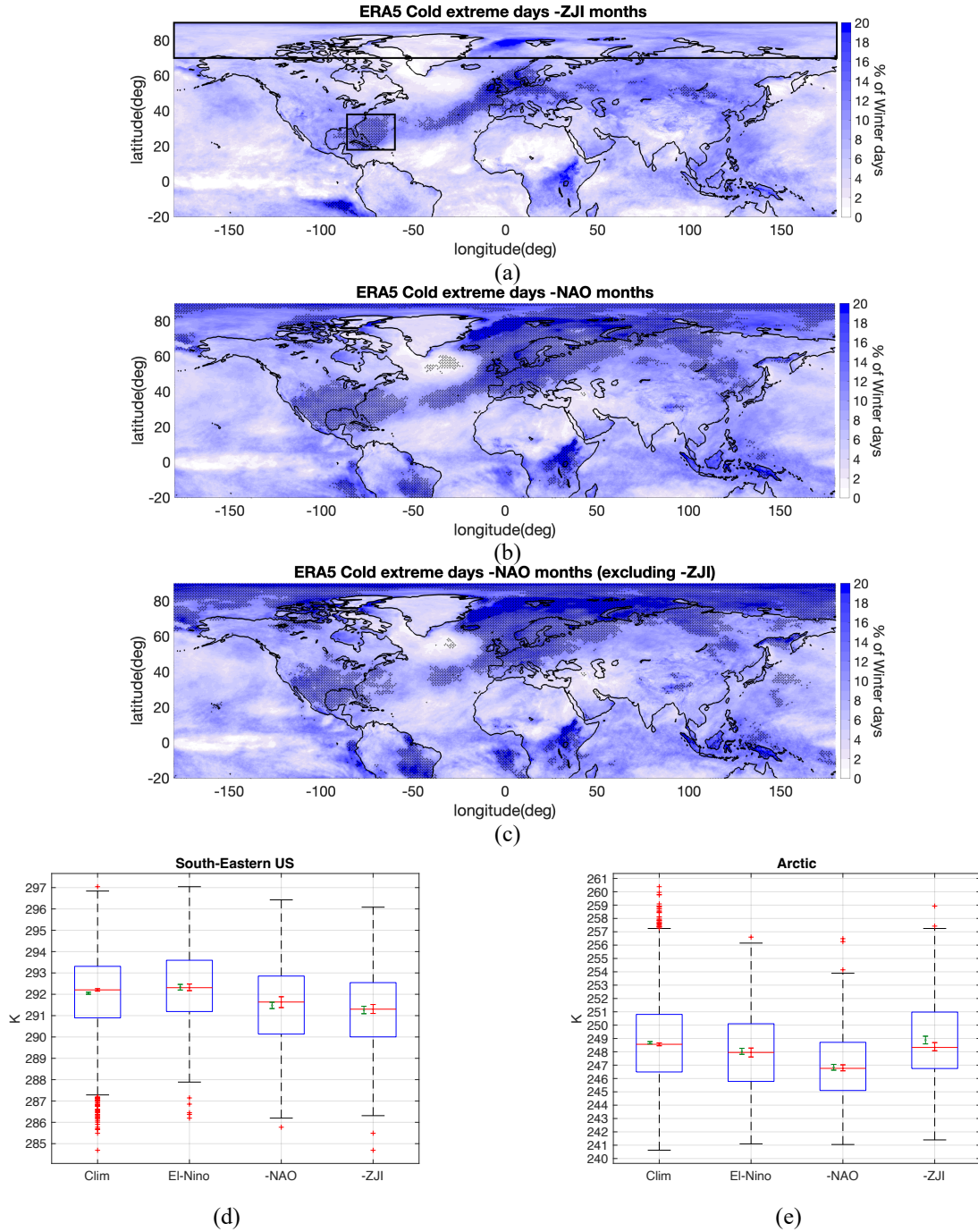
Figure 4. The distribution of the percentage of cold extreme days for (a) merged jet winter months (b) negative-NAO -NAO winter months (c) negative-NAO -NAO winter months excluding merged jet months. The regions stippled in black (+) represent regions significant at 99% using Monte Carlo simulation. Box plot of daily average surface temperature similar to Fig.3 over (d) south-east US coast [18°N-38°N,86°W-60°W] and (e)Arctics [70°N-90°N,180°W-180°E].These regions are marked in boxes in Fig.4a
