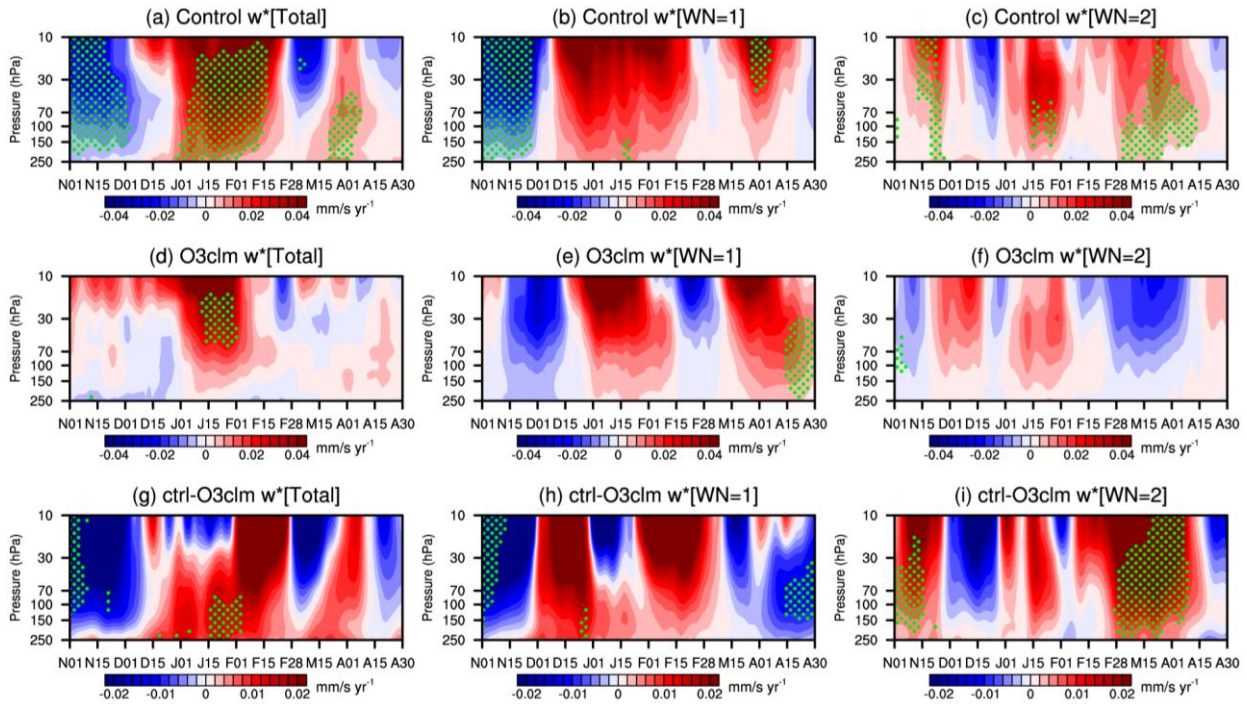
Figure 6 Linear trend of (a, d, and g) the vertical component of the BDC ( \bar{w}^* ) and its contribution (shading) from (b, e and h) the wavenumber 1 and (c, f and i) wavenumber 2 components before 2000 between 10 and 250 hPa averaged in the polar regions (65°–90°N) during winter and spring, derived from (a, b and c) the ensemble control experiments, (d, e and f) ensemble O3clm experiments and (g, h and i) the differences between the ensemble control experiments and ensemble O3clm experiments during the period 1980–2000. The green
