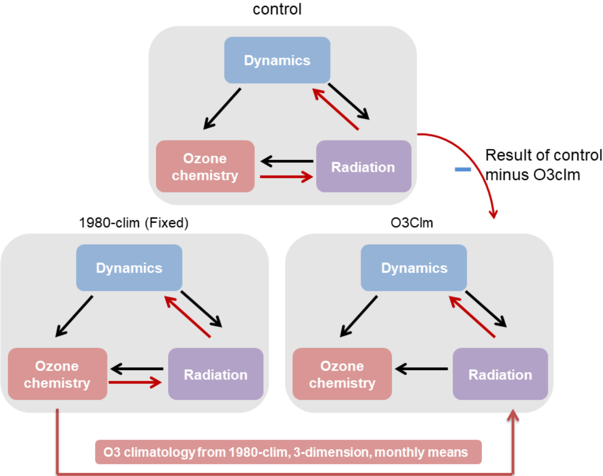
175 Figure 1 Simulation setup of the ensemble control and O3clm experiments. The control experiment treats ozone chemistry fully interactively. That is, the calculated ozone field has direct feedback on the atmosphere via the model radiation scheme. In contrast, the ensemble O3clm experiments do not use interactively calculated ozone in the radiation module. Instead, the radiation module uses an ozone climatology, which is derived from the 1980-clim experiment (see Section2.3) (This figure adapted from Fig. 3a in Friedel et al., 2022a and Fig.1 in Friedel et al., 2022b).
