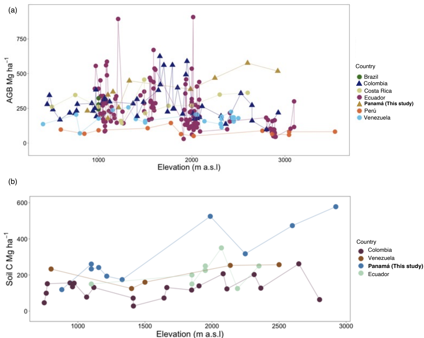
Figure 7. Comparison of above-ground biomass (a) and soil C (b) stocks among countries in the Neotropics from reports > 400 elevation. (a) Points represent AGB \text{Mg ha}^{-1} in values for six countries plus the current study in Panamá; symbols indicate sites with reported EM dominated forests (triangle) or low tree EM presence (less than 10 % or absence) (circles). Studies were performed in Brazil (Alves et al., 2011), Colombia (González-Caro et al., 2020), Costa Rica (Clark et al., 2002, Hofhansl et al., 2020, Lieberman et al., 1996, Tanner et al., 2016), Ecuador (Homeier & Leuschner et al., 2021; Moser et al., 2008), Peru (Malhi et al., 2017), Venezuela (Delaney et al., 1997; Vilanova et al, 2018) (b) Points represent soil C \text{Mg ha}^{-1} at 1 m depth for four countries. Studies were performed in Colombia (Phillips et al., 2019), Venezuela (Delaney et al., 1997) and Ecuador (Schrumph et al., 2001).
