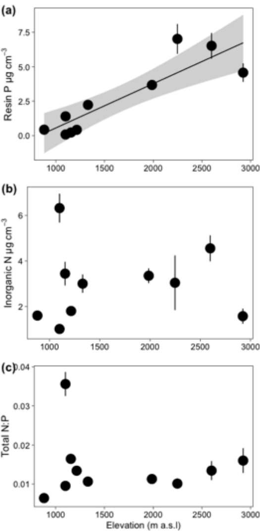
Figure 4. Relationship between elevation and soil parameters for ten 1-ha plots. Each point represents the plot mean ( \pm 1 SE) of a) resin P, b) inorganic N and c) total N:P. The solid line indicates a significant relationship and the shaded area represents the 95% confidence interval.
