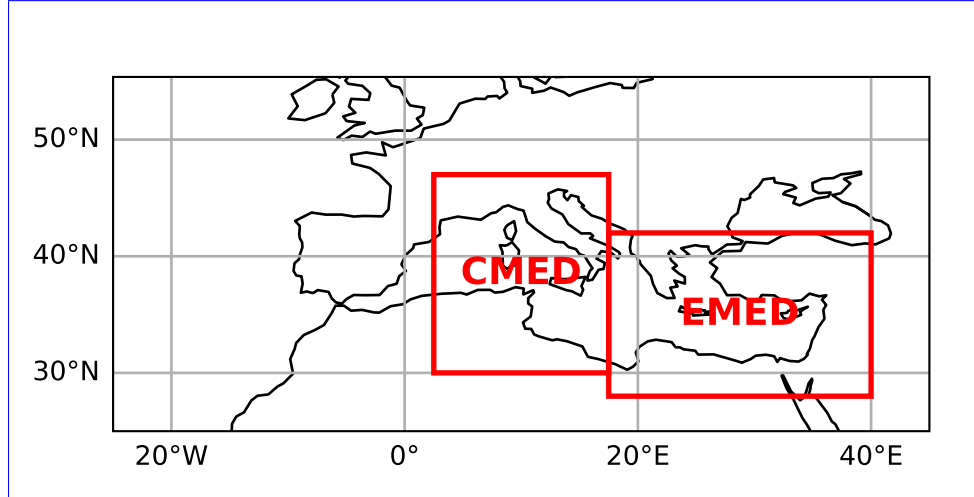
Figure 1. (a) Overview of stratospheric sulphur injections into the stratosphere as a result of volcanic eruptions. The arrows indicate when the 20 eruptions with the highest sulphur injections occurred. (b) The two regions of interest that are shown: “CMED” indicates the region defined as the central Mediterranean (between 2.5° E - 17.5° E and 30° N - 47° N), “EMED” indicates the region defined as the eastern Mediterranean (between 17.5° E - 40° E and 28° N - 42° N).
