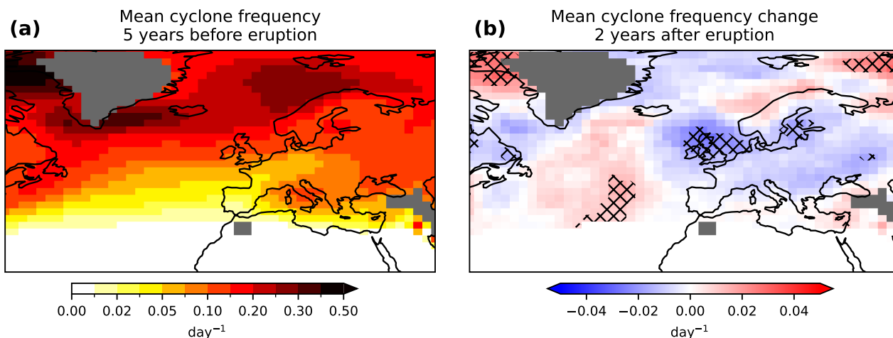
Figure 5. The mean cyclone frequency over northern Europe and the North Atlantic 5 years before the 20 strongest eruptions (a), and the changes in mean cyclone frequency that occur two years after the strongest eruptions (b). The stippling indicates where the changes are statistically significant ( p=0.05 ) at the 5% level . All results are for DJF. The grey shading indicates areas excluded from the analysis (the model elevation is above 1000 m asl).
