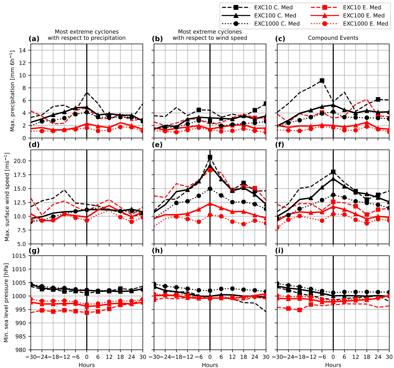
Figure S4. Same as Fig. 8, but now for JJA.
