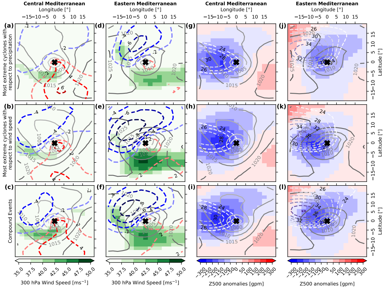
Figure 9. Same as Fig. 7 but now for 300 hPa wind speed in \text{ms}^{-1} (green shading), and 850 hPa temperature anomalies in ^{\circ}\text{C} (red and blue contour lines) in panels a–f. In panels g–l, red-blue shadings show the 500 hPa geopotential height anomalies in gpm and the dashed white contour lines show the Rossby wave packet amplitude in \text{ms}^{-1} . The grey contour lines indicate the SLP in all panels.
