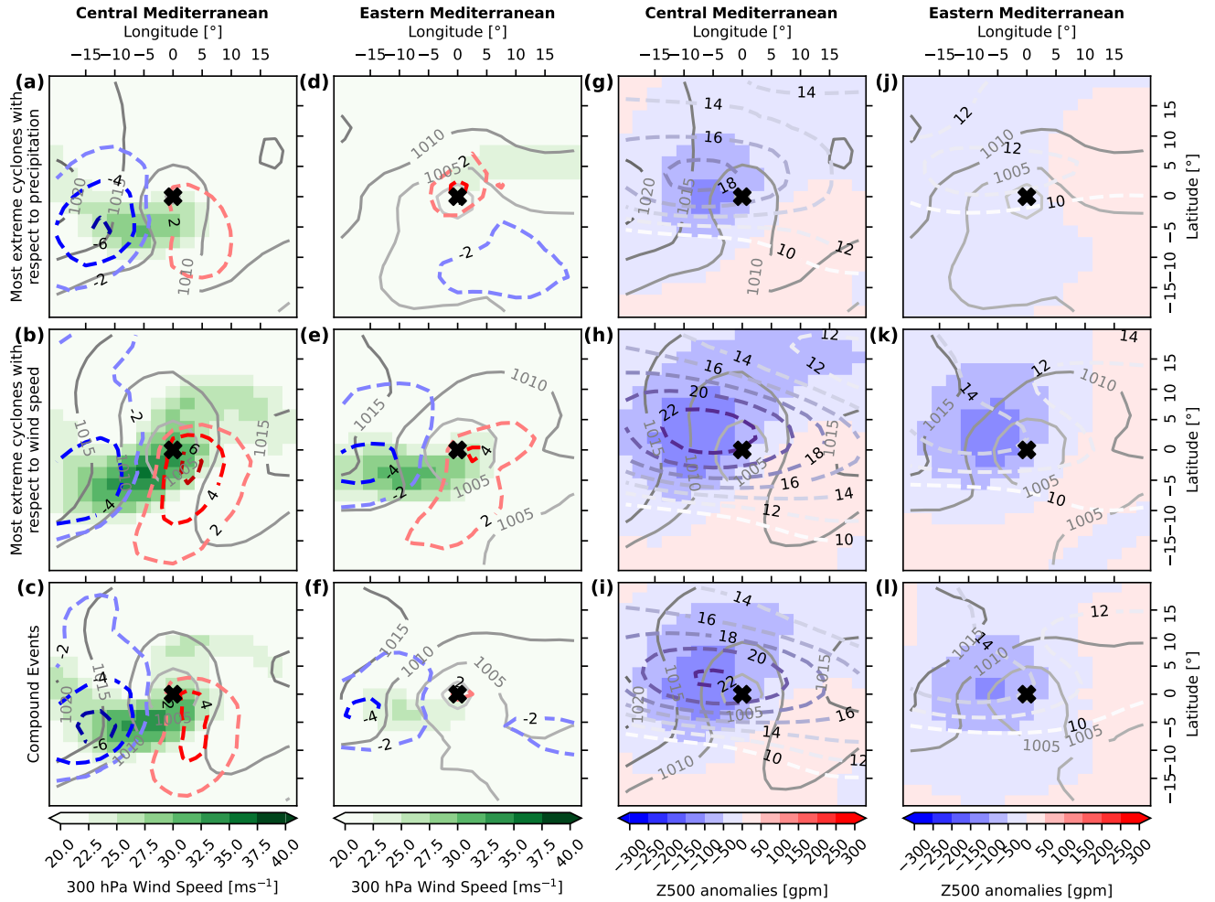
Figure S5. Same as Fig. 9, but now for JJA. Please note Note that the colorbar for the 300 hPa wind speed is different here compared to Fig.
