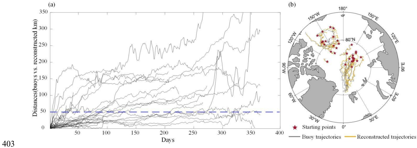
403 404 Figure 8. Comparison of reconstructed ice trajectories with buoy trajectories: (a) misalignment distances over time for trajectory pairs; (b) 405 trajectory pairs from the deployment site of buoys.
