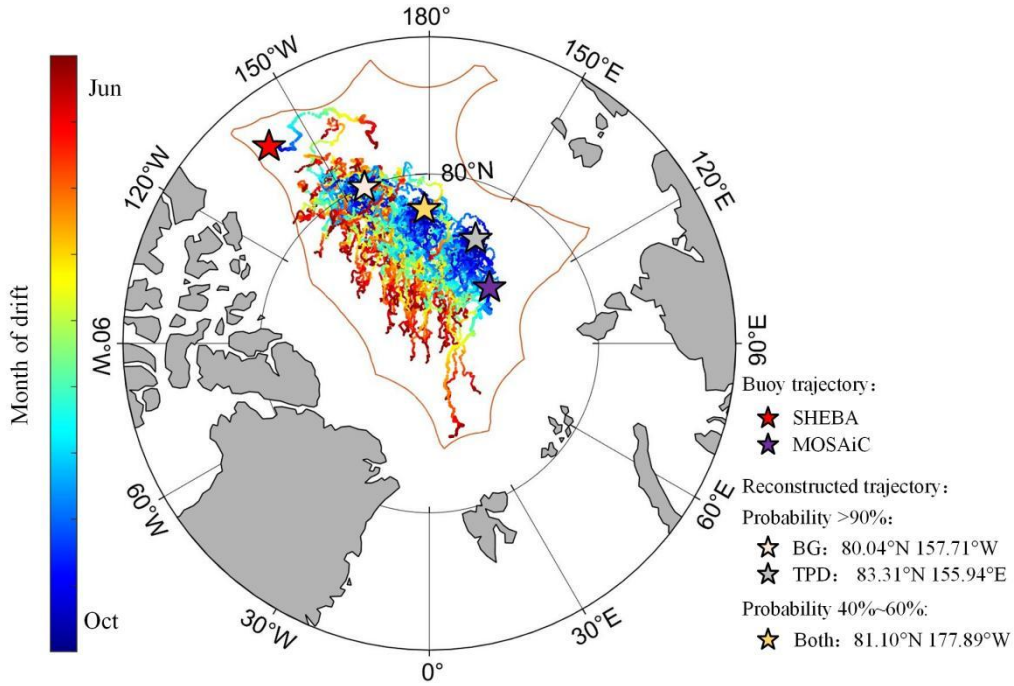
241 Figure 3. Reconstructed 9-month sea ice trajectories in 1979–2022, starting from three geometric centers of grid points with a probability 242 of reaching the BG or TPD region greater than 90% and that having ambiguous destination with a probability of reaching both regions 243 between 40% and 60%. For comparison, the partial drifting trajectories of SHEBA and MOSAiC ice camps started from October 3 of 1997 244 and 2019 to the time of 9 months after deployment are also shown.
