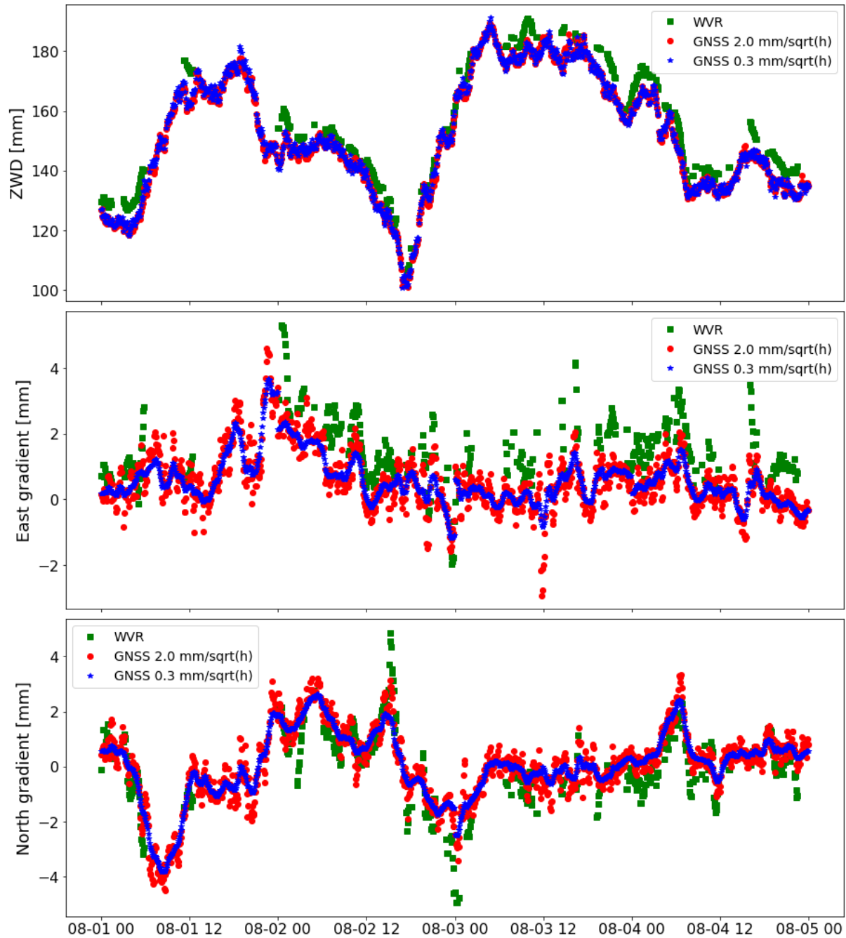
Figure 5. An example of gradient time series from the WVR and from two GNSS solutions for the ONSA station, using different constraints, 0.3 and 2.0 \text{ mm}\sqrt{\text{h}}^{-1} .
