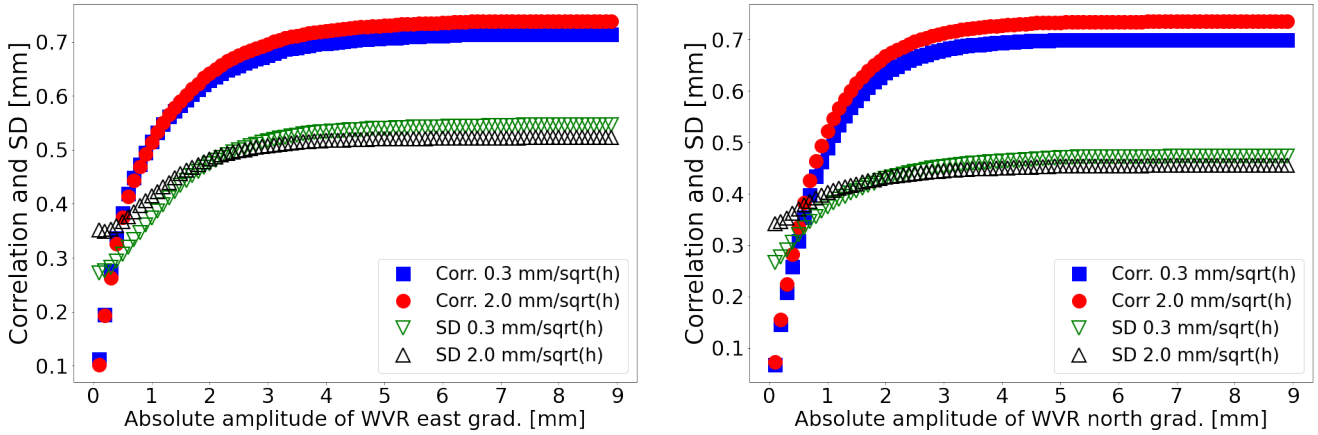
Figure 9. Illustration of how the correlation and the standard deviation (SD) depends on the range of observed gradients. Here correlation and SD are shown as a function of the maximum amplitude of the east (left) and north (right) gradient from the WVR.
