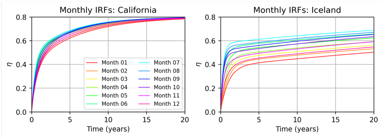
Figure 7. Using the month-long alkalinity release simulations conducted in January, April, July, and October by Zhou et al. (2024), we construct a library of IRFs for each location corresponding to each month by linearly interpolating between months 1, 4, 7, and 10. The left panel shows the resulting monthly IRFs for California (Polygon 214, Figure 12), and the right panel is Iceland (Polygon 36).
