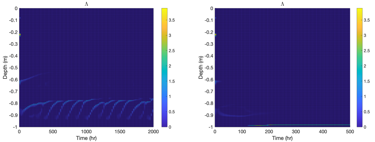
Figure 5. The ratio \Lambda = \alpha \max(0, \text{Ra} - \text{Ra}_{\text{crit}}) / P for the two computations shown in Figures 3 and 4. In both cases, flow is caused by thin regions, where \Lambda \approx 1 , that drive Rayleigh-Taylor convection, suggesting that microbes can control convective transport rate through osmolyte production P .
