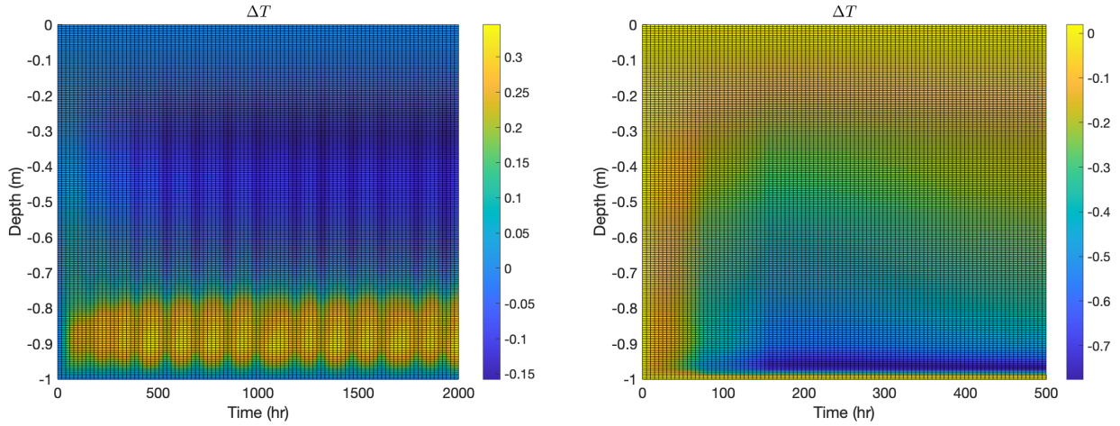
Figure 4. Temperature change T(z,t) - T(z,0) after addition of microbes for the same computations as in Fig. 3, again with biofilm population for 2000 h (left) and planktonic population for 500 h (right) microbial populations . Vertical axes indicate depth from the ice-air interface at z = 0 . In the biofilm case, (1) temperature increases in the convective region because of inflow of relatively warm seawater and (2) temperature decreases in the mid-ice region likely because of smaller diffusivity (due to increased brine volume fraction). In the planktonic case, temperature decreases throughout the ice sheet, although the decrement is relatively small in the thin convective region at the bottom of the sheet.
