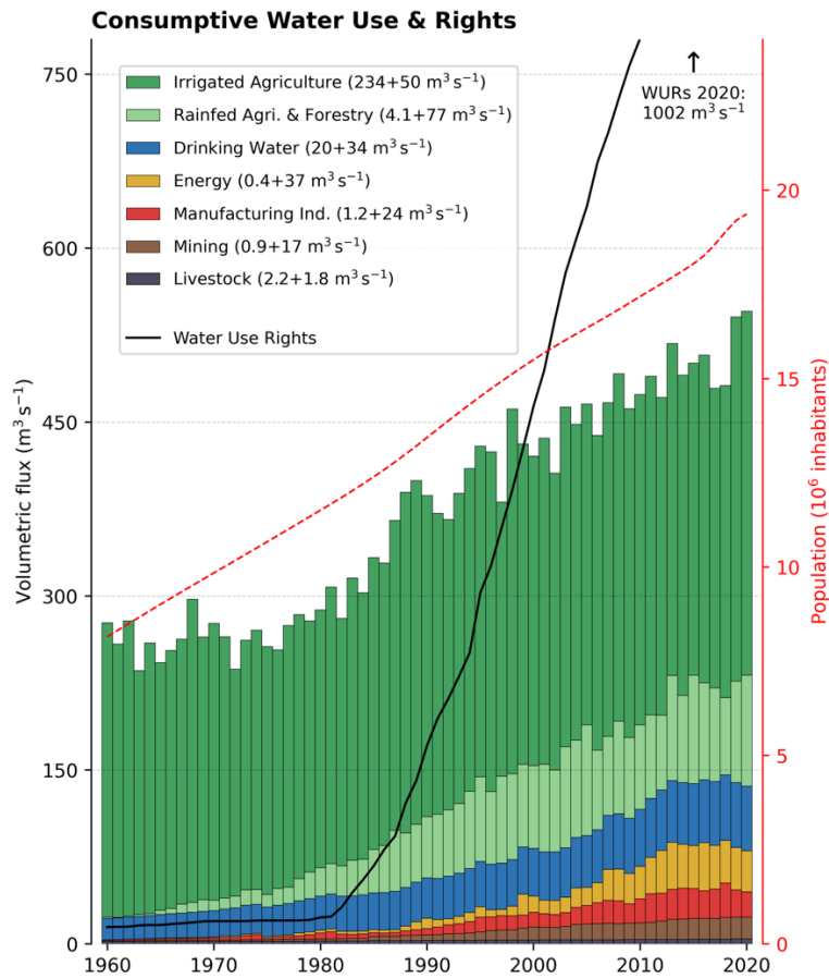
470 Figure 5: Historical evolution (annual means) of consumptive water use and allocated rights (WURs, black curve) in Chile. The values in the legend indicate the average water use during the 1960s and the increase towards the 2010s for each sector. Dashed curve (red axis) show the country's population (source: World Population Prospects, UN, 2024).
