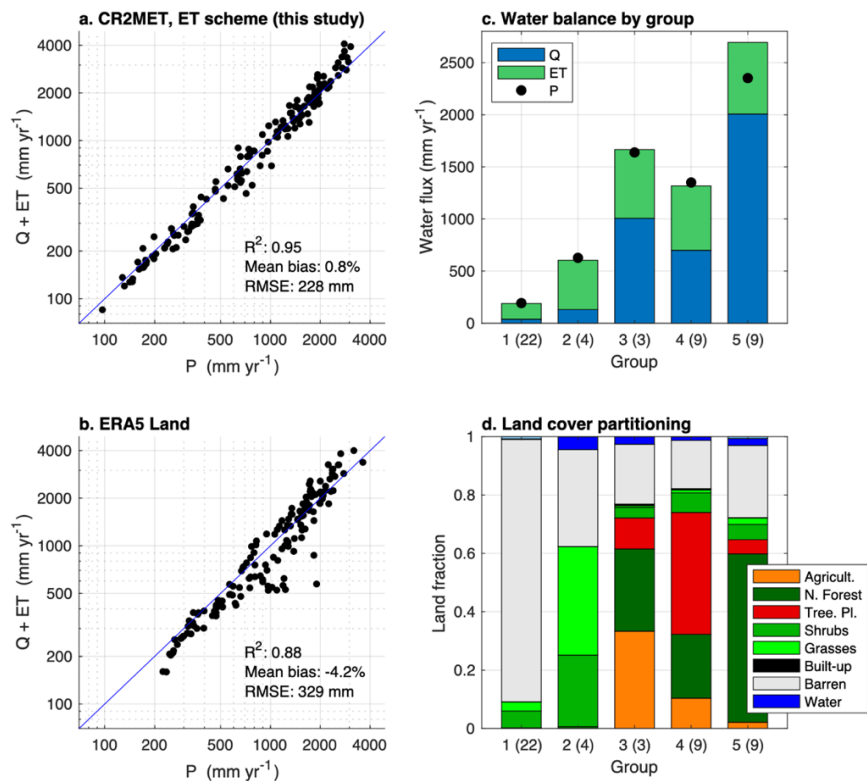
785 Figure A1: Comparison of mean annual precipitation (P) in 147 watersheds in Chile with observed river streamflow (Q) and modeled evapotranspiration (ET). The estimates of P and ET in panels a and b correspond to those assessed in this study (CR2MET-driven) and from ERA5-Land, respectively. Panel c shows the CR2MET-based flux comparison for groups of watersheds with dominant fractions of barren land (>85%, group 1), shrubland and grasses (>40%, group 2), agriculture (>30%, group 3), tree plantations (>30%, group 4), and native forest (>50%, group 5). The number of basins and mean land cover partitioning of each group is shown in panel d.
