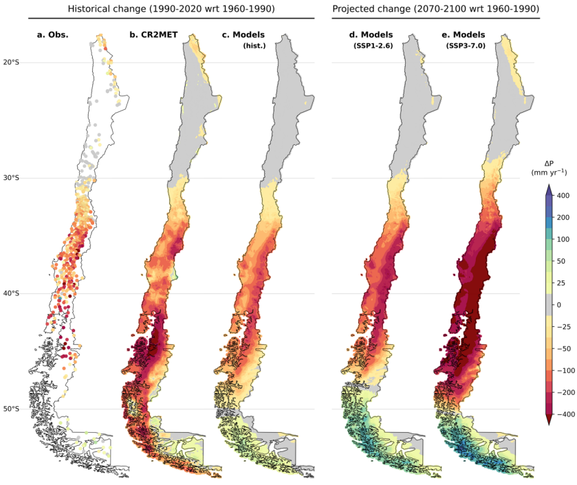
Figure 2: Changes in mean annual precipitation in Chile between the periods 1960-1990 and 1990-2020 (a-c), and projected towards the end of the 21st century (2070-2100) under global scenarios SSP1-RCP2.6 (d) and SSP3-RCP7.0 (e). Historical changes are based on local observations (a), the CR2MET dataset (b), and CMIP6 model simulations (historical scenario and SSP3 for 2015-2020). The three modeled changes (c-e) are based on downscaled simulations from 17 CMIP6 ESMs (showing the multi-model mean).
