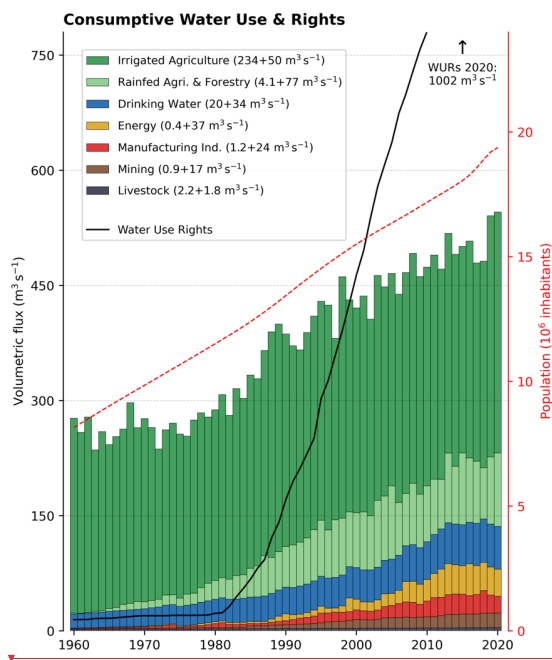
Figure 5: Historical evolution (annual means) of consumptive water use and allocated rights (WURs, black curve ) in Chile. The values in the legend indicate the average water use during the 1960s and the increase towards the 2010s for each sector. Dashed curve (red axis) show the country's population (source: World Population Prospects, UN, 2024).
