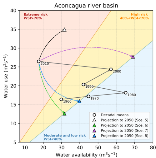
820 Figure 9: The decadal evolution of consumptive water use, water availability, and the corresponding WSI category (background) in the Aconcagua River basin for the period 1960-2020 (circles). Triangle markers indicate different scenarios for the mid-21st century under a global climate scenario with low greenhouse gas emission mitigation (SSP3-7.0, scenarios 5 to 8 in Table 2).
