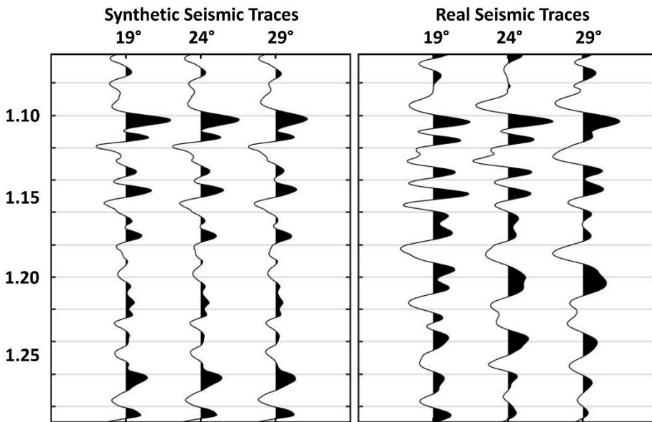
345 Figure 5: Seismic well tie for real data used.
