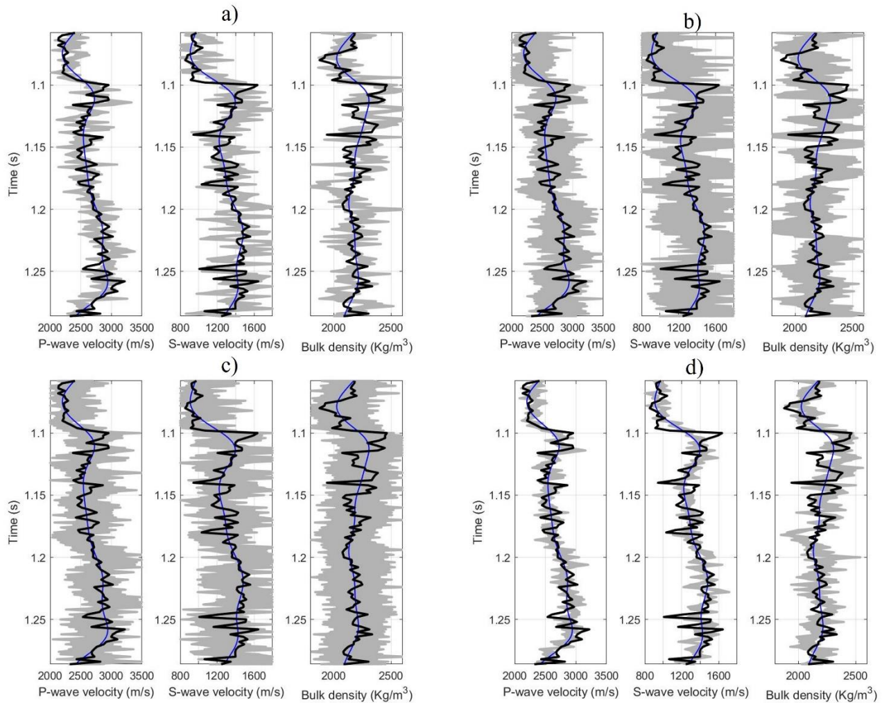
425 Figure 7: True data (black line), prior model (red blue line), and accepted realizations of the model (gray) for real data where a) MH, b) HMC, c) MALA, and d) Lip-MALA.
