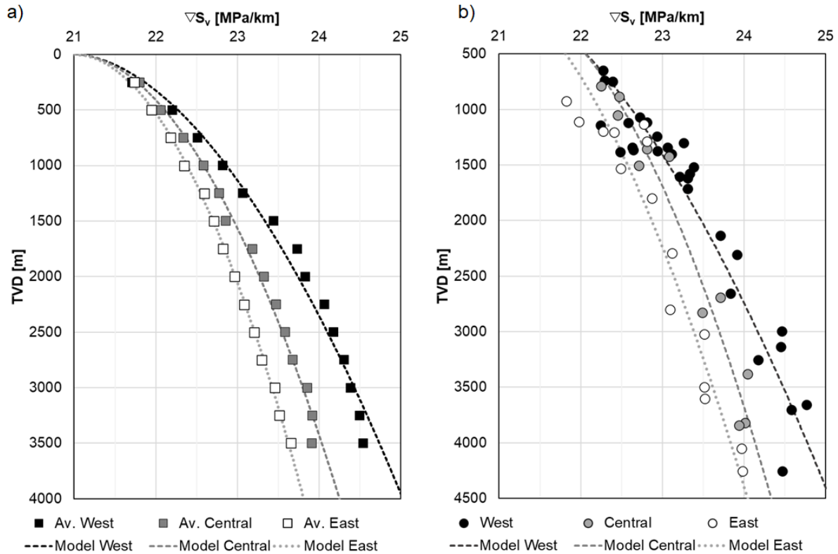
Figure 7: Vertical stress gradients from Dataset II as a function of true vertical depth below ground level TVD . a) Average and modelled vertical stress gradients in the western, central and eastern part of the study area (cf. Fig. 6). Average vertical stress gradients reflect the arithmetic mean from all wells in the western, central and eastern part of the study area at 14 depths and with a step size of 500 \pm 2 m. b) Well-based and modelled vertical stress gradients in the western, central and eastern part of the study area at the top of the Upper Jurassic.
