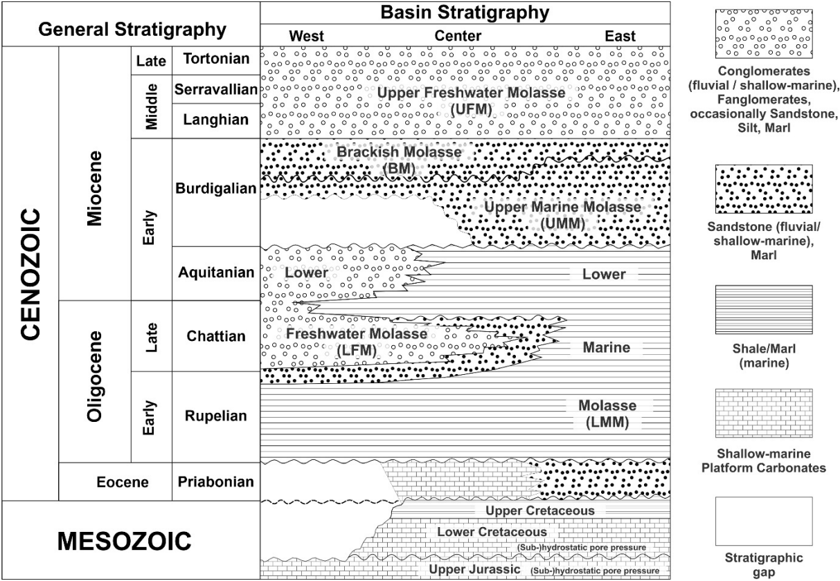
Figure 2: Chronostratigraphic chart of the North Alpine Foreland Basin in SE Germany modified from Drews et al. (2018) after Kuhlemann and Kempf (2002) and Bachmann and Müller (1992).
