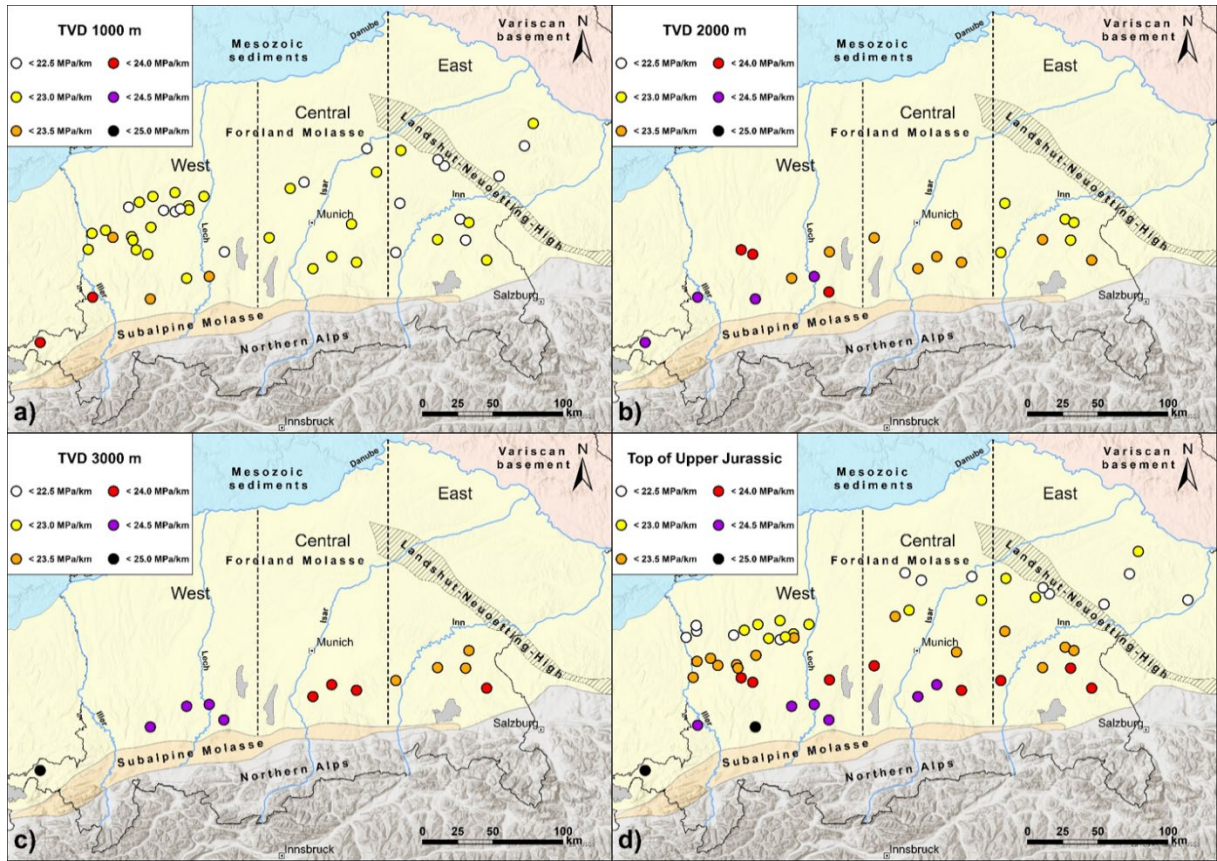
Figure 6: Distribution of vertical stress gradients in MPa/km in the North Alpine Foreland Basin. Vertical stress gradient distribution at a true vertical depth below ground level a) TVD = 1000 m, b) TVD = 2000 m, c) TVD = 3000 m d) Vertical stress gradient distribution at the top of Upper Jurassic carbonates. The N-S trending dashed black lines divide the study area in a western, central and eastern part.
