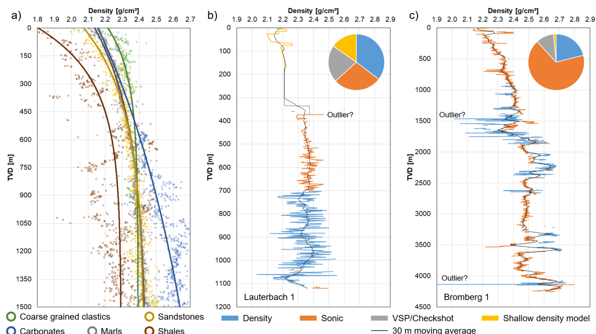
Figure 5: Bulk density profiles. a) Shallow bulk density profiles for each main lithological unit (lines) fitted to quality-controlled and transformed bulk density data from all wells with available data. R^2 values for the bulk density models of coarse grained clastics, sandstones, carbonates, marls and shales are 0.56, 0.82, 0.54, 0.87 and 0.50, respectively. b) Example of a spliced and averaged bulk density profile for the shallow Lauterbach 1 well in the north-western part of the study area (LAU in Fig. 1a). c) Example of a spliced and averaged bulk density profile for the deep Bromberg 1 well in the south-eastern part of the study area (BRO in Fig. 1a). The pie chart insets of b) and c) indicate the coverage by quality-controlled bulk density data (blue), transformed density from sonic velocity (orange) and seismic interval velocity from vertical seismic profiles (VSP) or checkshots (gray) and the shallow bulk density model (yellow) (Tab. 1).
