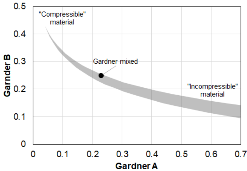
Figure 3: Theoretically possible range for Gardner A and B (grey area) for natural occurring bulk rock densities (1.5-3.0 g/cm 3 ) and velocities (1500-6000 m/s). The black dot “Gardner mixed” marks the A-B combination (A=0.23, B=0.25) for mixed lithologies after Gardner et al. (1974).
