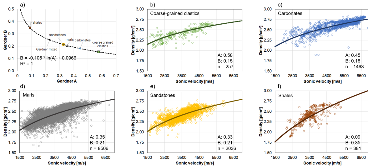
Figure 4: Lithologically calibrated velocity-bulk density relationships based on Gardner et al. (1974). a) Relationship between A-B-parameters for the main lithological units. A-B-parameters were fitted to quality-controlled velocity-bulk density-relations for b) coarse-grained clastics, c) carbonates, d) marls, e) sandstones and f) shales.
