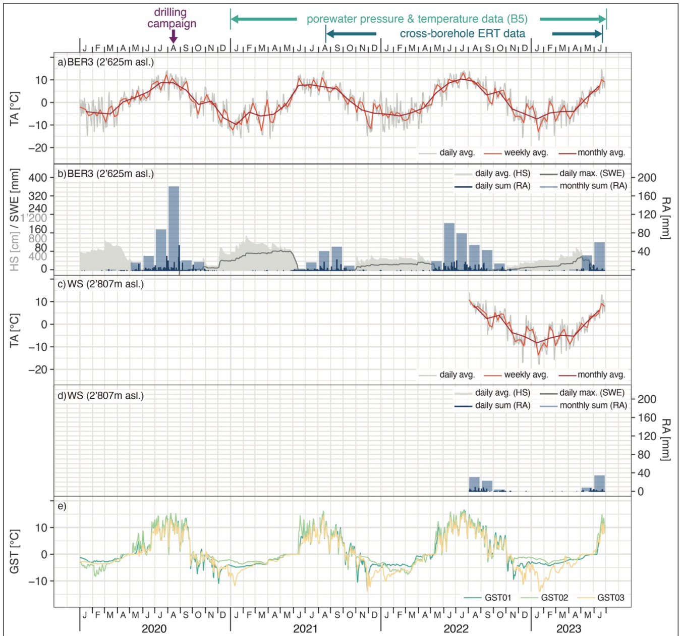
220 Figure 3: Air temperature (TA), snow height (HS), modelled snow water equivalent (SWE), and rainfall (RA) at the IMIS station Puoz Bass (BER3) (a and b), air temperature (TA) and rainfall (RA) from the Schafberg weather station (WS) (c and d), and ground surface temperature (GST) for the three miniature temperature data loggers GST01, GST02, and GST03 (e), for the observation period January 2020 to June 2023. Legends are embedded in each individual diagram. Boreholes B3, B4 and B5 were drilled in August 2020 (purple arrow above). The observation periods for pore water pressure, temperature records, and electrical resistivity tomography (ERT) time steps are marked with mint green and light blue arrows, respectively. WS has recorded data since 05 August 2022. Note the data gap for SWE between 01 January 2020 and 31 August 2020 (b). See Fig. 1d and Tab. S1 for location and detailed station information, Tab. S2 for quarterly and yearly metrics, and Fig. S1 for the IMIS station BER2.
