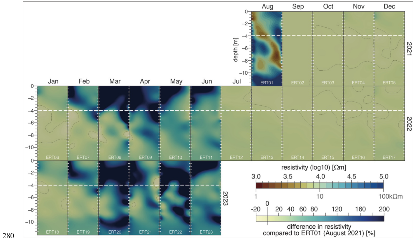
Figure 7: Relative changes in inverted electrical resistivity based on the first ERT dataset on 20 August 2021 (ERT01) between September 2021 and June 2023. The data behind each tomogram were recorded on the 20th of each month (except 29 March 2023). Years are shown on the right of the figure, months on the top. The naming of the tomograms follows the date in ascending order and is indicated at the bottom of the tomogram in white light letters (ERT01 to ERT23). Electrode positions are indicated by the light grey short lines. Borehole B4 is located to the right of each tomogram, B3 to its left. The thin solid lines denote the 0 % isoline. The white dashed lines indicate the maximum depth of the active layer.
