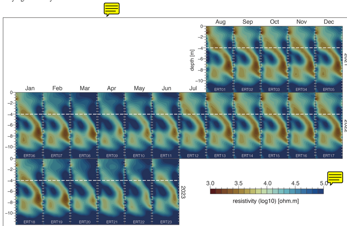
255 Figure 6: Inverted resistivity tomograms of the 23 selected cross-borehole electrical resistivity tomography (ERT) datasets between August 2021 and June 2023. The data behind each tomogram were recorded on the 20th of each month (except 29 March 2023). Years are shown on the right of the figure, months on the top. The naming of the tomograms follows the date in ascending order and is indicated at the bottom of the tomogram in white light letters (ERT01 to ERT23). The ERT multi-core cables with 24 electrodes per borehole (indicated by the light grey short lines) and a vertical spacing of 0.5m are installed the boreholes B3 and B4. Borehole B4 is located to the right of each tomogram, B3 to its left. The white dashed lines indicate the maximum depth of the active layer. See Fig. 1 for borehole locations, Fig. 2 for further details and stratigraphy, and Fig. 7 for relative electrical resistivity changes. 260
