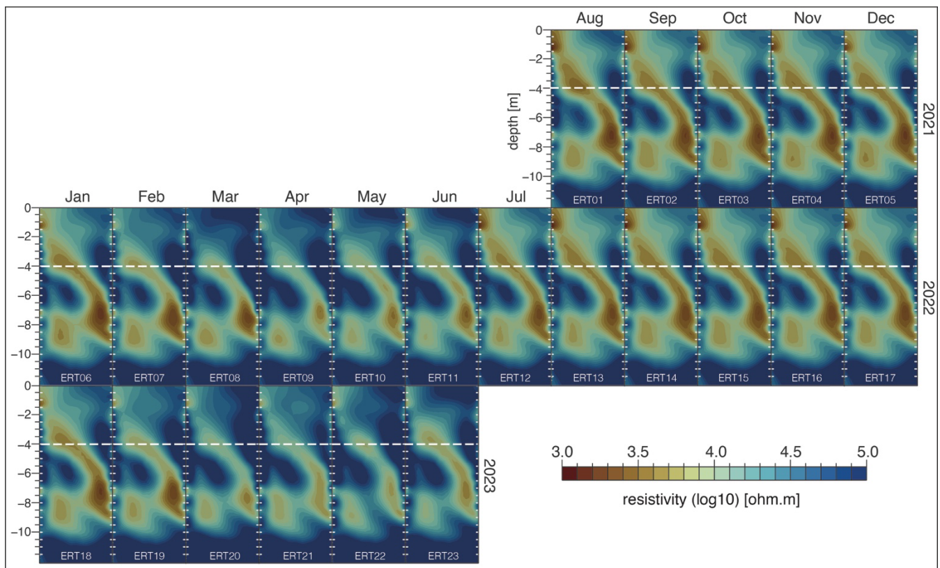
Figure 6: Inverted resistivity tomograms of the 23 selected cross-borehole electrical resistivity tomography (ERT) datasets between August 2021 and June 2023. The data behind each tomogram were recorded on the 20th of each month (except 29 March 2023). Years are shown on the right of the figure, months on the top. The naming of the tomograms follows the date in ascending order and is indicated at the bottom of the tomogram in white light letters (ERT01 to ERT23). The ERT multi-cables with 24 electrodes per borehole (indicated by the light grey short lines) and a vertical spacing of 0.5m are installed the boreholes B3 and B4. Borehole B4 is located to the right of each tomogram, B3 to its left. The white dashed lines indicate the maximum depth of the active layer. See Fig. 1 for borehole locations, Fig. 2 for further details and stratigraphy, and Fig. 7 for relative electrical resistivity changes.
