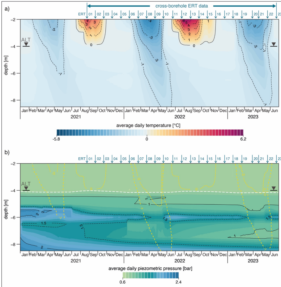
330 Figure 5: Time-depth-temperature (a) and time-depth-piezometric pressure (b) plots for borehole B5 from January 2021 to June 2023. Hourly data were aggregated to daily values before plotting (arithmetic average). In addition to the colouring, integer isotherms and selected isobars are highlighted with solid (0 °C, 1 and 2 bar, respectively) and dashed black lines. Thermistors and piezometers are located at depths of 2, 3, 4, 4.5, 5, 5.5, 6, 6.5, 7.5, and 8.5 m. The black triangle indicates the maximum thickness of the active layer (ALT). Fig. 5b additionally highlights the varying piezometric pressure at the ALT (white dashed line shows the depth of thaw), and shows 0 °C, -1 °C and -2 °C isotherms (yellow dashed lines). See Fig. 1 for borehole location, and Fig. 2 for stratigraphy. The
