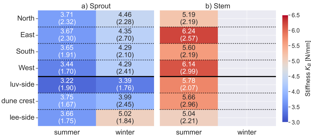
Figure E1. Heatmap showing stiffness K_B for (a) sprout and (b) stem in different zones and seasons. The values within the heatmap cells represent the mean stiffness (in N/mm) with the standard deviation in parentheses.
