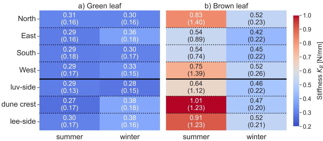
Figure E2. Heatmap showing stiffness K_B for (a) green leaf and (b) brown leaf in different zones and seasons. The values within the heatmap cells represent the mean stiffness (in N/mm) with the standard deviation in parentheses.
