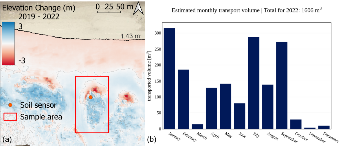
Figure C1. Morphological changes 2019 - 2022 for the Cusp Dune (a) based on DEM data with a 1\text{ m} \times 1\text{ m} raster resolution provided by the Lower Saxony Water Management, Coastal and Nature Protection Agency (NLWKN). Aeolian transport volume calculation for 2022 based on wind speed and direction data sourced from the German Weather Service (DWD) station on Spiekeroog situated between the two field sites.
