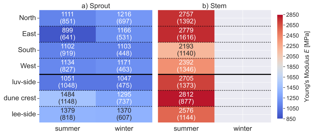
Figure E3. Heatmap showing Young's modulus E for (a) sprout and (b) stem in different zones and seasons. The values within the heatmap cells represent the mean Young's modulus (in MPa) with the standard deviation in parentheses.
