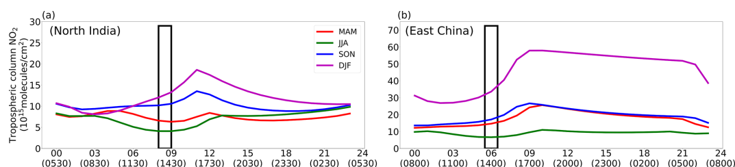
Figure 2. Diurnal cycles of tropospheric column NO 2 (10 15 molec. cm -2 ) simulated by UKCA over (a) north India and (b) east China for the four seasons (averaged over 2005–2015). The time axis displays UTC times, with local time shown in parentheses. The box highlights the OMI overpass time, representing the period used for UKCA-OMI comparisons.
