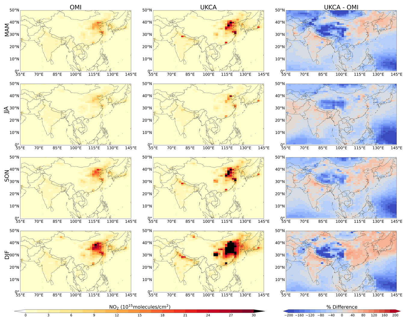
Figure 6. Seasonal tropospheric column NO 2 ( 10^{15} molec. \text{cm}^{-2} ) distributions from OMI (left), simulated by UKCA (middle), and the percentage difference ( 100\% \times (\text{UKCA} - \text{OMI}) / \text{UKCA} ) between UKCA and OMI (right).
