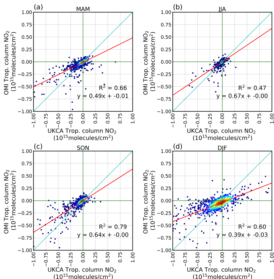
Figure 12. Scatter plots of UKCA and OMI tropospheric column NO 2 trends ( 10^{15} molec. \text{cm}^{-2} \text{yr}^{-1} ) from 2011 to 2015 by season. The 1 : 1 line is shown in cyan colour and the best fit line in red colour. Data points shown as a heat map, where red corresponds to more data. The equations of the best fit and the coefficient of determination ( R^2 ) are also shown. Note that N = 2050 data points are used for the fit, though some points fall outside the scales shown.
