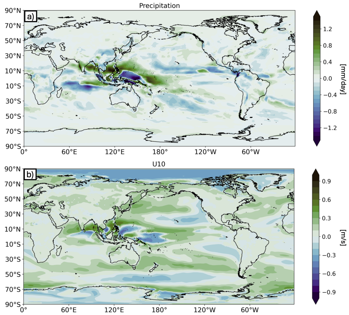
Figure 9. The annual absolute bias difference of NIense and the SUPERense ( ((\text{NIense-Observations}) - (\text{SUPERense-Observations})) ) for precipitation (a) and 10-meter windspeed (b). Positive values indicate SUPERense is more skillful and vise-versa.
