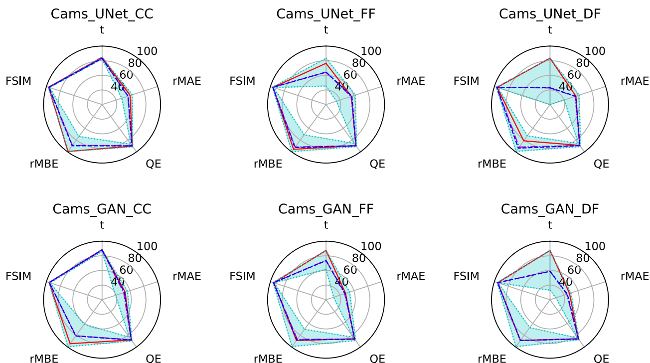
Figure 9. Overview of each couple model - fusion strategy. The charts names shows information about the chosen dataset, the model, and the fusion type. Regarding the fusion type, 'CC' means 'Channel Concatenation' or Data Fusion, 'FF' means Feature Fusion, and 'DF' means Decision Fusion.
