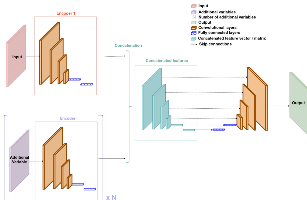
Figure 3. Architecture of the UNet with feature fusion approach. Also corresponds to the architecture of the GAN's generator.
