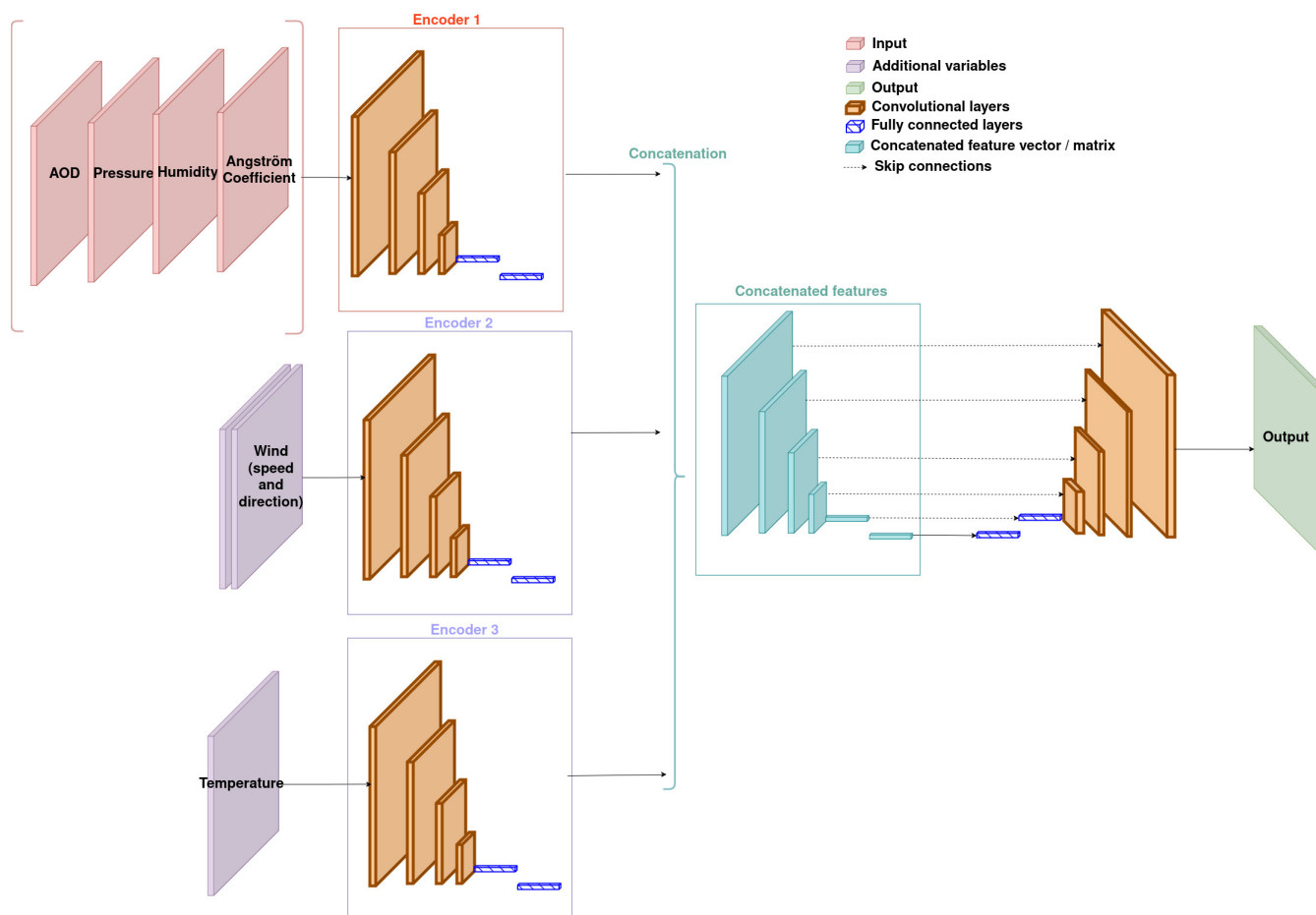
Figure 6. The second proposed hybrid model, using both data fusion and feature fusion.
