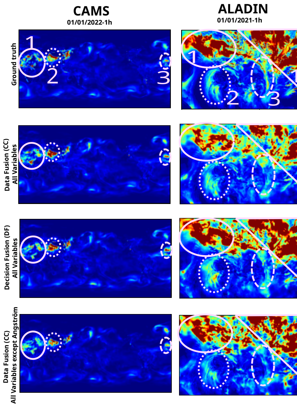
Figure 11. Outputs of the best models on both datasets for one given sample. The pink circles and numbers have been added afterwards to attract the reader's attention on some details of the image.
