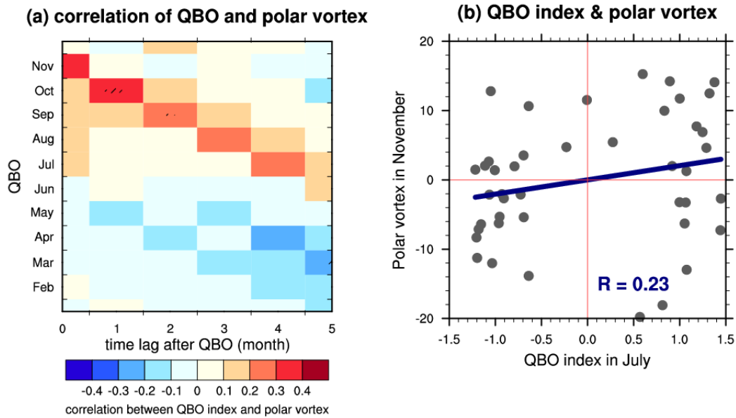
Figure 1: (a) Correlations between the zonal-mean zonal wind at 60°S and 70 hPa and the QBO index at different time lag derived from the MERRA-2 reanalysis dataset. The Y-axis represents the month of the QBO index used in the correlation analysis. The X-axis indicates the time lags. The shadings indicate that the correlations are statistically significant at 90% confidence level. (b) Monthly mean zonal-mean zonal wind at 60°S and 70 hPa in November (with a 5-month lag after the QBO in July) plotted against the July QBO index according to MERRA-2 reanalysis dataset from 1980 to 2022. The solid blue line represents the linear regression of the QBO index and the strength of Antarctic stratospheric polar vortex, with their correlation coefficient shown in the bottom right-hand corner.
