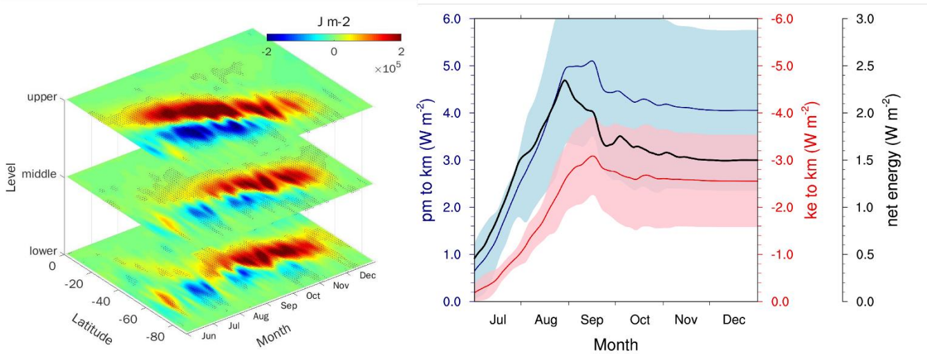
Figure 9: (a) Composite differences in mean kinetic energy (KM) from July to November between the Pos-Exmode and Neg-Exmod according to MERRA-2 reanalysis dataset. The KM at “upper”, “middle”, and “lower” levels are integrated 1–20 hPa, 30–50 hPa, and 70–100 hPa, respectively. The dotted regions mark-indicate that the differences between the Pos-Exmode and Neg-Exmode are statistically significant at the 90% confidence level. (b) Composite differences in time-integrated energy transformations averaged over 1–100 hPa and 40°S–70°S between the Pos-Exmode and Neg-Exmode. The blue and red shadings indicate significant intervals. If these shadings do not cross the X-axis, the difference is significant at the 90% confidence level. The blue line, corresponding to the left Y-axis, represents the energy transformed from the mean potential energy (PM) to KM. The red line, corresponding to the first right Y-axis, represents the energy transformed from the eddy kinetic energy (KE) to KM. The black line, corresponding to the second right Y-axis, represents the net energy transformed to KM.
