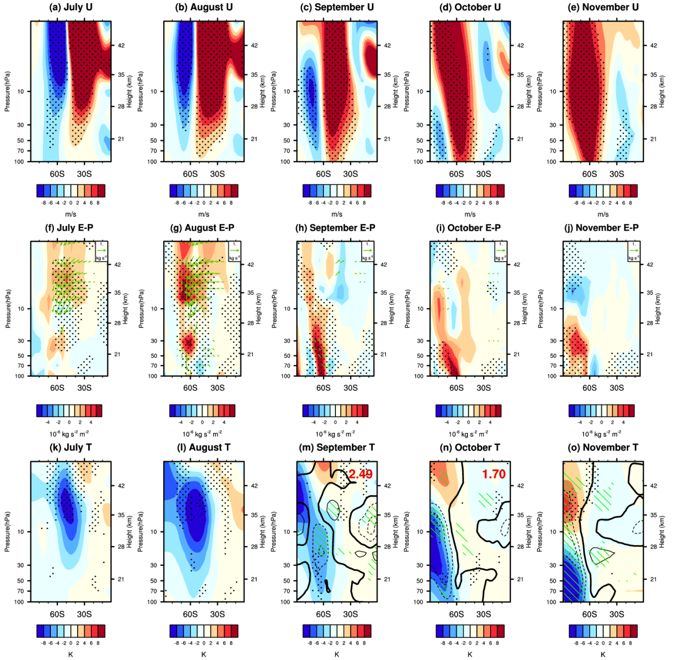
Figure 4: Composite differences in (a)–(e) the zonal-mean zonal wind anomalies, (f)–(j) the scaled E-P flux anomalies (green vectors; horizontal component unit: 10^7 \text{ kg s}^{-2} ; vertical component unit: 10^5 \text{ kg s}^{-2} ) and the E-P flux divergence anomalies (shadings), (k)–(o) the zonal-mean temperature anomalies (shadings) and the zonal-mean ozone volume mixing ratio anomalies (contours; dashed lines are negative, and thick lines are zero contours). The contour intervals are 200 ppbv from July to November between the Pos-Exmode and Neg-Exmode according to MERRA-2 reanalysis dataset. Composite differences in PSC areas between the Pos-Exmode and Neg-Exmode, based on the NASA ozone watch dataset from September to October, are shown at the top of Panels (m) and (n). The E-P flux and its divergence are calculated from wave 1 to 3. E-P flux vectors are scaled by the factor \cos\phi and multiplied by the square
