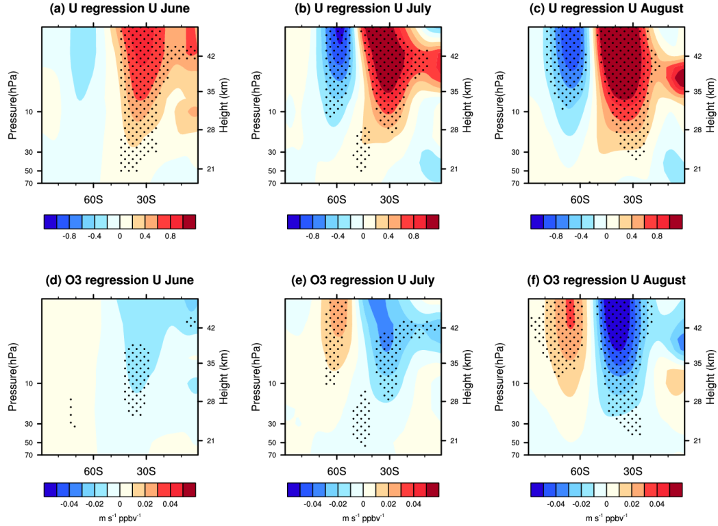
Figure 2: (a)–(c) Regression patterns of the zonal-mean zonal wind in (a) June, (b) July, and (c) August against the zonal-mean zonal wind at 60°S and 70 hPa in November during WQBO years , derived from the MERRA-2 reanalysis dataset. (d)–(f) Regression patterns of the zonal-mean zonal wind in (d) June, (e) July, and (f) August against the ozone concentration averaged over the south of 60°S at 70 hPa in November during WQBO years , derived from the MERRA-2 reanalysis dataset. The shadings indicate that the regression coefficients are statistically significant at 95% confidence level.
