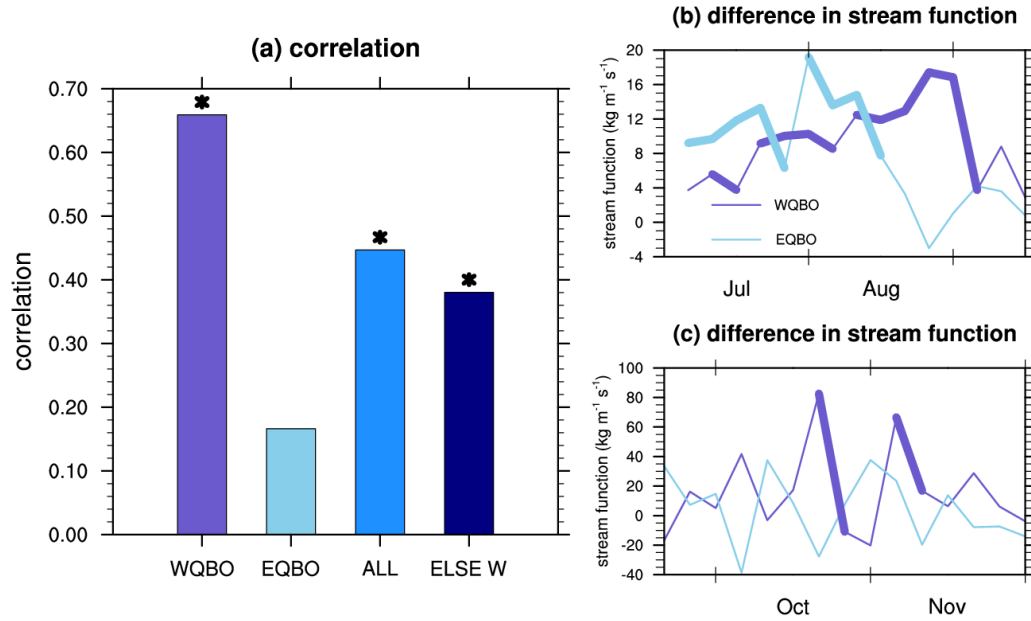
Figure 10: (a) The correlations between zonal-mean zonal wind in extratropical and polar regions under during WQBO years (WQBO) , EQBO years (EQBO) , all years ( ALL ), and years except WQBO ( ELSE W ) derived from MERRA-2 reanalysis dataset from 1980 to 2022 . The asterisks indicate that the correlations are statistically significant at the 95% confidence level. (b) Composite differences in stream function averaged over 0–60°S and 1–30 hPa between the strong and weak polar vortex during the WQBO (purple lines) and EQBO (blue lines) from July to September. The thick lines indicate that the differences between the strong and weak polar vortex are statistically significant at the 90% confidence level. (c) Same as panel (b), but the stream function averaged over 30°S–60°S and 50–100 hPa from September to November.
