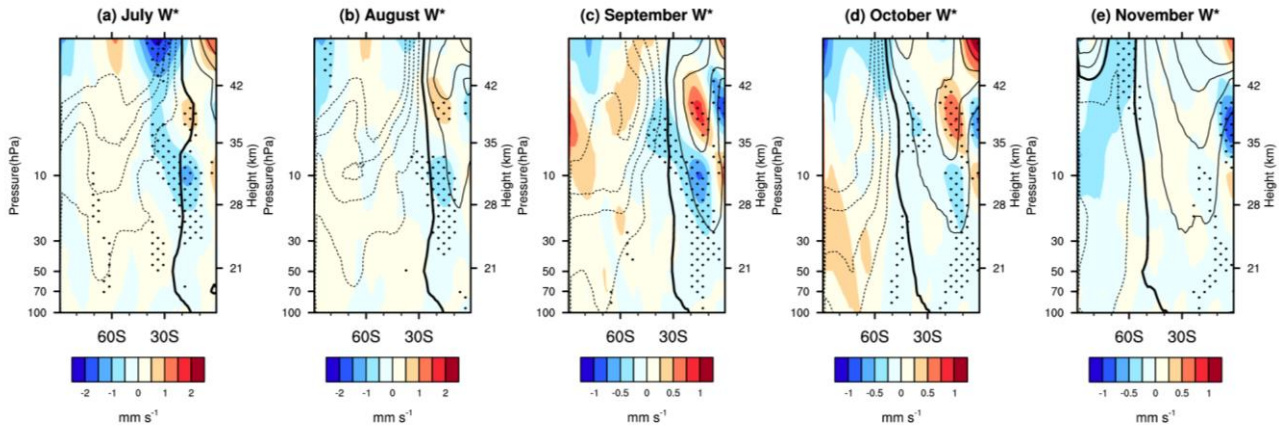
Figure 11: Composite differences (color shadings) in \bar{w}^* between WQBO and EQBO from July and November according to the MERRA-2 reanalysis dataset. The dotted regions mark-indicate that the differences in \bar{w}^* between the WQBO and EQBO are statistically significant at the 90% confidence level. The contours indicate the climatological \bar{w}^* from 1980 to 2022. The dashed lines are negative. Thick lines are zero contours, and the contour intervals are 0.5 mm/s.
