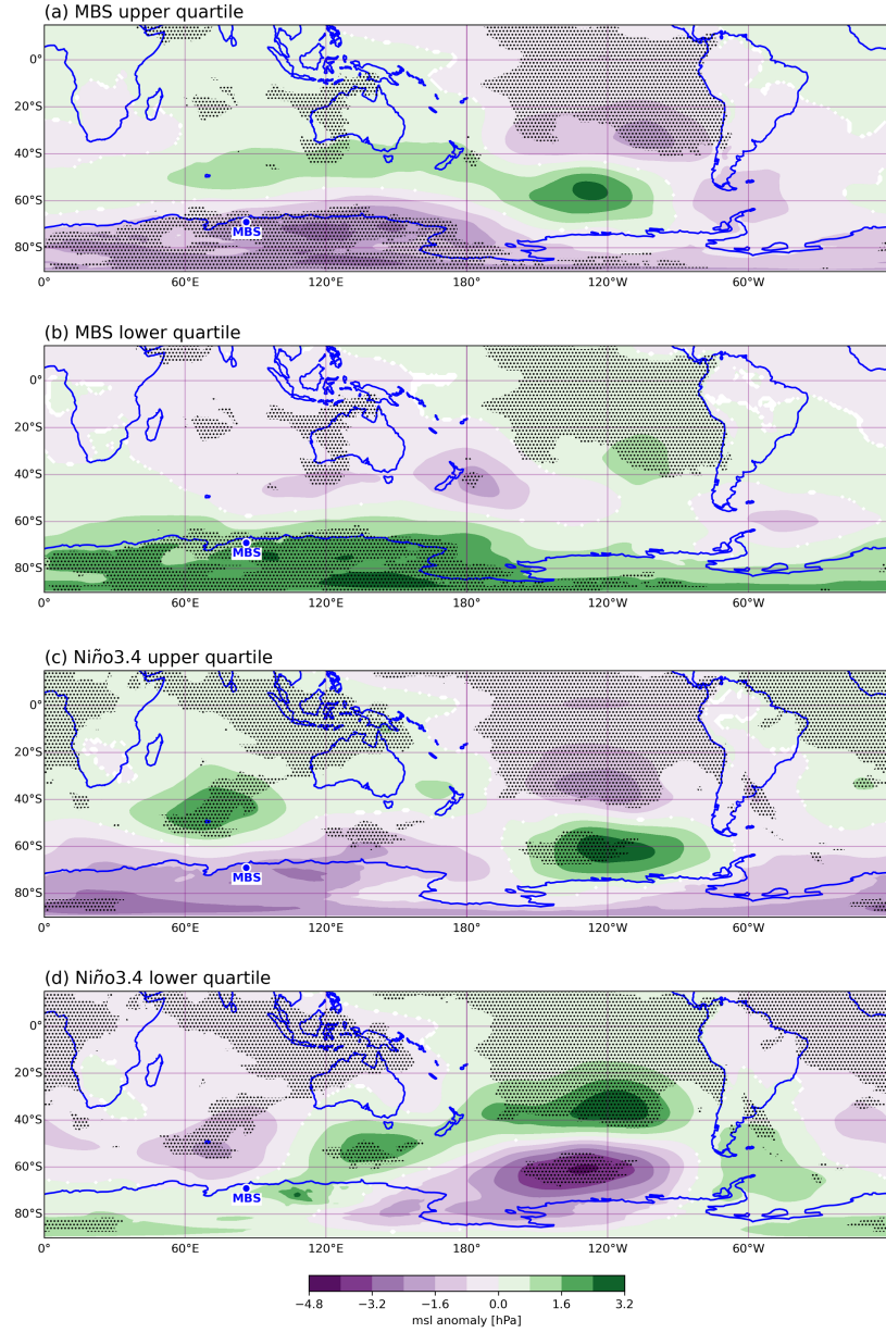
Figure A1. Composite maps of the winter ERA5 mean sea level pressure anomaly for the Mount Brown South site average (MBS CI^- ) (a) upper [1982, 1986, 1987, 1993, 1996, 1997, 2009, 2012, 2014, 2015] and (b) lower quartile [1980, 1981, 1983, 1990, 1991, 1995, 1999, 2001, 2010, 2011] and for the Niño3.4 (c) upper [1982, 1987, 1991, 1993, 1997, 2002, 2004, 2009, 2012, 2015] and (d) lower quartile [1984, 1985, 1988, 1989, 1998, 1999, 2000, 2007, 2010, 2011]. The stippling indicates points where the mean sea level pressure anomaly K-S test p value is < 0.1 . The blue dot indicates MBS.
