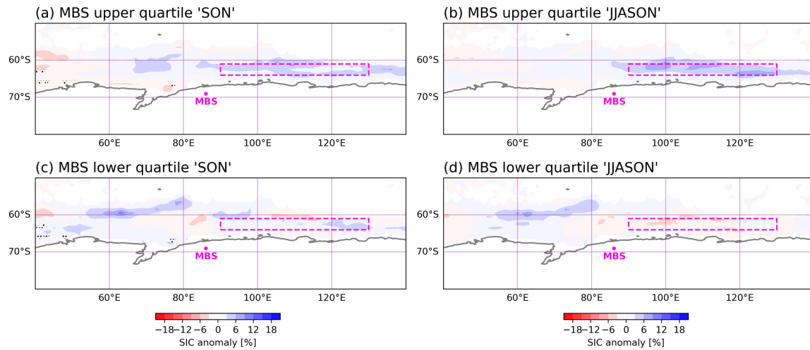
Figure A6. Composite maps of the (a, c) September–November (b, d) July–November sea ice concentration for the Mount Brown South site average (MBS CI^- ) (a, b) upper [1982, 1986, 1987, 1993, 1996, 1997, 2009, 2012, 2014, 2015] and (c, d) lower quartile [1980, 1981, 1983, 1990, 1991, 1995, 1999, 2001, 2010, 2011]. The stippling indicates points where the K-S test p value is < 0.1. The MBS northeast coast box (61–64° S, 90–130° E) highlighted by the fuchsia dashed line while the fuchsia dot indicates MBS.
