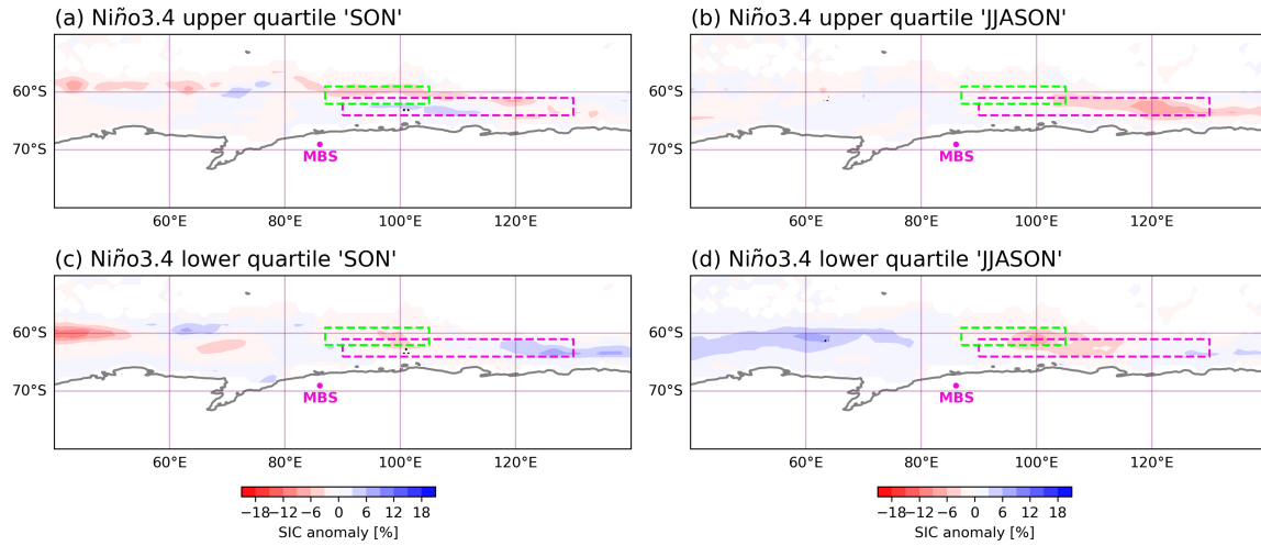
Figure A9. Composite maps of the (a, c) September–November (SON) (b, d) July–November (JJASON) sea ice concentration for the Niño3.4 (a) SON (b) JJASON upper and (c) SON (d) JJASON lower quartile. The stippling indicates points where the K-S test p value is < 0.1. The MBS northeast coast box (61–64° S, 90–130° E) highlighted by the fuchsia dashed line while the fuchsia dot indicates MBS.
