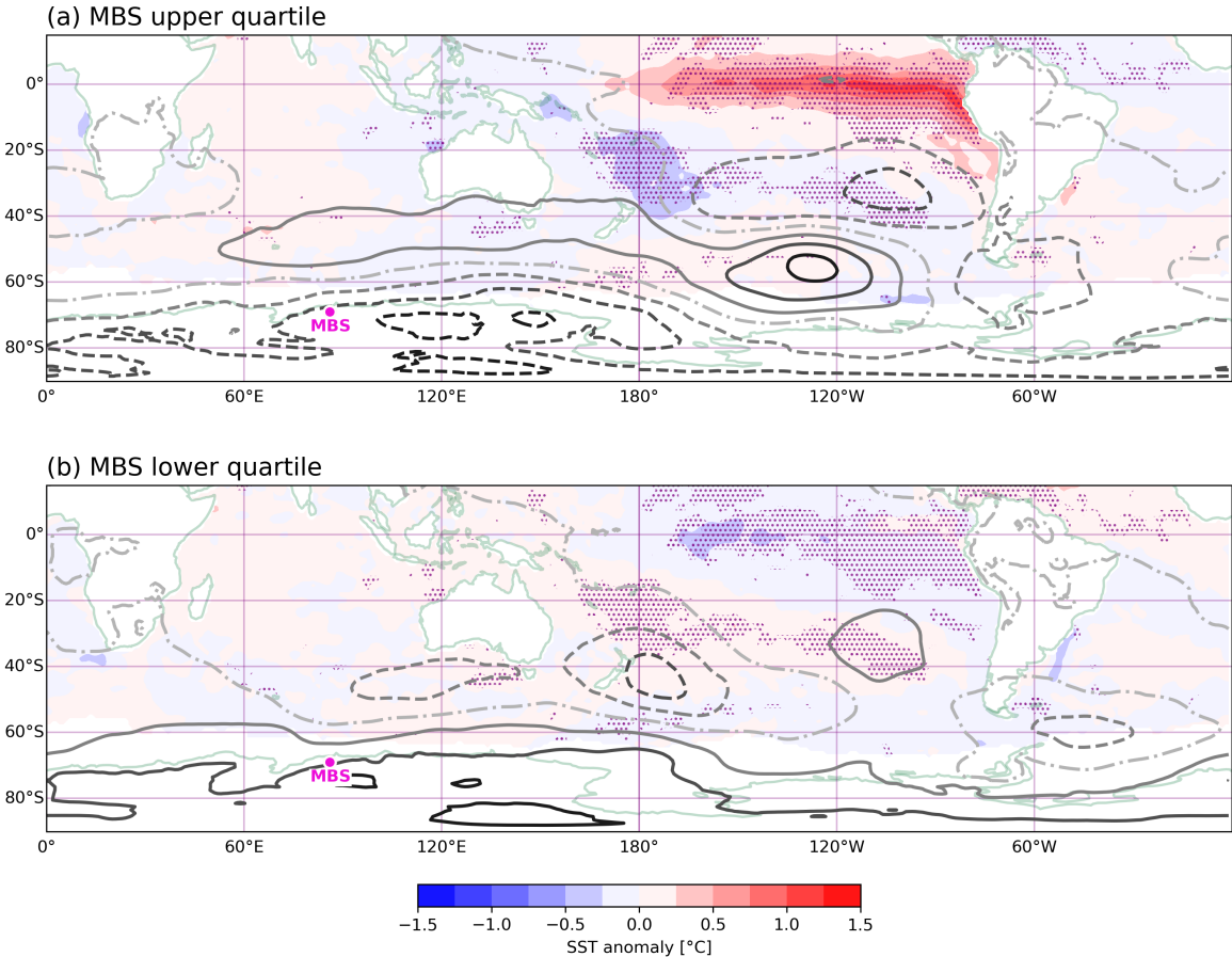
Figure 1. Composite maps of the winter (JJA) sea surface temperature anomaly (shading) and ERA5 mean sea level pressure anomaly (contours) for the Mount Brown South site average (MBS Cl - ) (a) upper [1982, 1986, 1987, 1993, 1996, 1997, 2009, 2012, 2014, 2015] and (b) lower quartile [1980, 1981, 1983, 1990, 1991, 1995, 1999, 2001, 2010, 2011]. High (low) MSLP anomalies shown by solid (dashed) contours, with darker shades of grey indicating stronger anomalies. The contour line graduations indicate 0.8 hPa. The stippling indicates points where the K-S test p value is < 0.1 for the sea surface temperature anomaly (shading). The fuchsia dot indicates MBS. Wind anomalies near the MBS region are next analysed to investigate whether there is variance in the source of sea salt (potentially due to sea ice or other changes in sea salt aerosol production) or changes in regional circulation patterns associated with the transport of salts. Z scores of the meridional and zonal wind anomalies are considered, since they are standardized and provide context as to how strong or weak wind anomalies are with respect to the mean.
