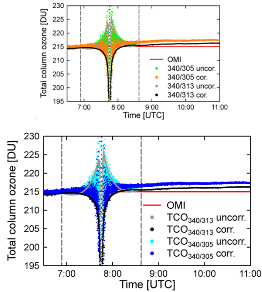
Figure 17: GUV measurements of TCO at Union Glacier on 4 December 2021. Uncorrected and LD-corrected \text{TCO}_{340/305} data are shown in green-cyan and orangeblue , respectively. Similar data calculated for \text{TCO}_{340/313} are shown in grey and black. The average of OMI measurement for this day is indicated by a horizontal red line. Long-dashed lines indicate the 1 st and 4 th contact. The 3 rd and 4 th contact are indicated by dashed-dotted lines.
