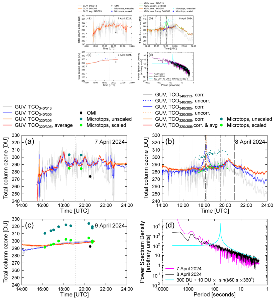
Figure 9: Measurements of TCO at Mazatlán on (a) 7 April 2024, (b) 8 April 2024, (c) and 9 April 2024. TCO_{340/313} , TCO_{340/305} , and TCO_{320/305} measurements at 1 Hz are shown in gray, blue, and orange, respectively. The red line shows 90-second moving averages of TCO_{320/305} calculated from the 90-second global spectral irradiance segments, which are separated by the shadow banding segments. TCO derived from TCO_{340/305} —Microtops measurements are biased high (cyan-dark green circles). Data scaled down by 6.5 % are also shown (light green) for ease of comparison with GUV data. OMI measurements are only available on 7 and 9 April 2024. All data were filtered for SZAs smaller than 75^\circ . The vertical “very long-dashed” vertical lines (before 16:00 and at about 21:00) indicate the times when the shadow of the Moon either first hit-touched the Earth (over the Pacific) or leaves-ft the Earth (over Greenland). 1 st and 4 th contact at Mazatlán are indicated by dashed lines, and the 2 nd and 3 rd contact are indicated by dashed-dotted lines. Panel (d) shows the power
