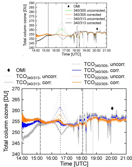
Figure 13: Measurements of TCO at Fort Collins on 14 October 2024 with the GU. Uncorrected and LD-corrected \text{TCO}_{340/305,13} , \text{TCO}_{340/305} , \text{TCO}_{320/305} data are shown in grey, blue, and green and orange, respectively. Uncorrected and LD-corrected data Similar data for \text{TCO}_{340/313} are shown in grey and black . are indicated by broken and solid lines, respectively. The The OMI measurement of this day is also indicated by a black diamond. Long-dashed lines indicate the 1 st and 4 th contact. The time of the eclipse maximum is indicated by a short-dashed line and the local solar noon is indicated by a gray line.
