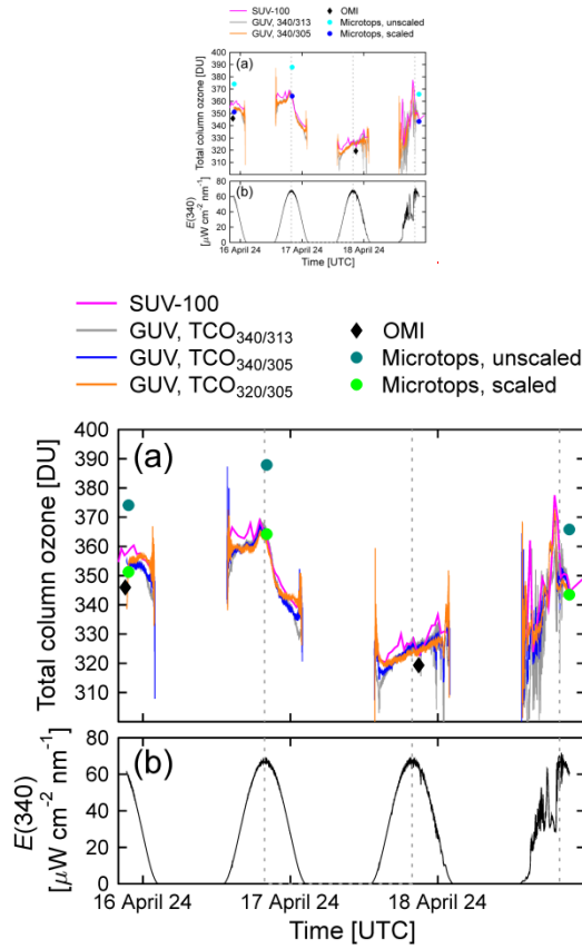
Figure 5: (a) Total column ozone at San Diego calculated from Version 2 spectra of the SUV-100 spectroradiometer (pink line), derived from GUUV measurements for the 340/313 (gray line), and 340/305 (orange-blue line), and 320/305 (orange line) wavelength pairs, provided by OMI (black diamond), and measured by the Microtops (cyan-dark green circle). Microtops measurements scaled by 1/1.065 are also shown. Only data up to SZAs of 85° are included. (b) Spectral irradiance at 340 nm measured by the GUUV radiometer. Vertical broken lines indicate the times of local solar noon.
