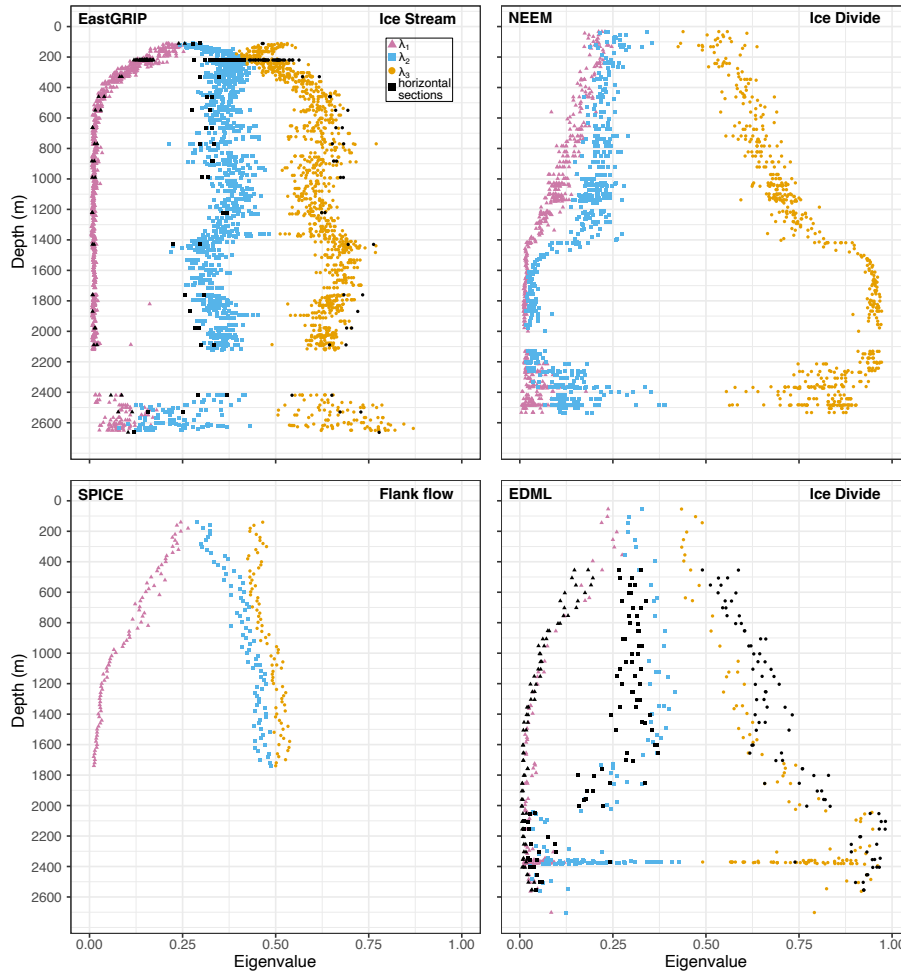
Figure 12. Comparison of the anisotropy between EastGRIP, NEEM, EDML and SPICE via their eigenvalue pattern with depth (Montagnat et al., 2014a; Weikusat et al., 2017; Voigt, 2017). Note the differences between maximum values of \lambda_3 of EastGRIP and SPICE compared to NEEM and EDML. Annotations as in Fig-Figure 7; all axes are formatted the same for better comparison.
