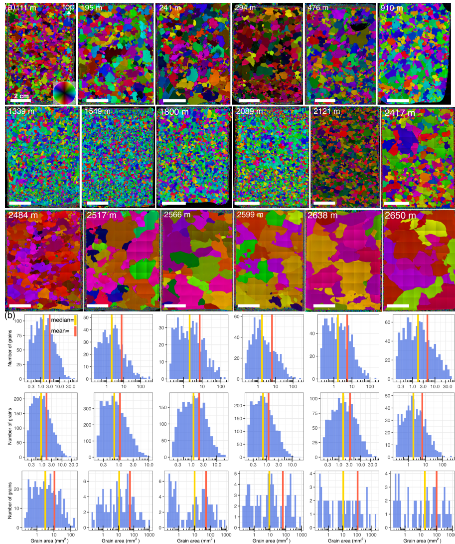
Figure 9. Representative selection displaying the a) microstructure and b) respective grain size distributions (note the varying axes) at similar depths as the CPOs in Fig. Figure 3 . Top indicates the surface of the ice sheet. The c-axis orientation is indicated by the colour wheel.
