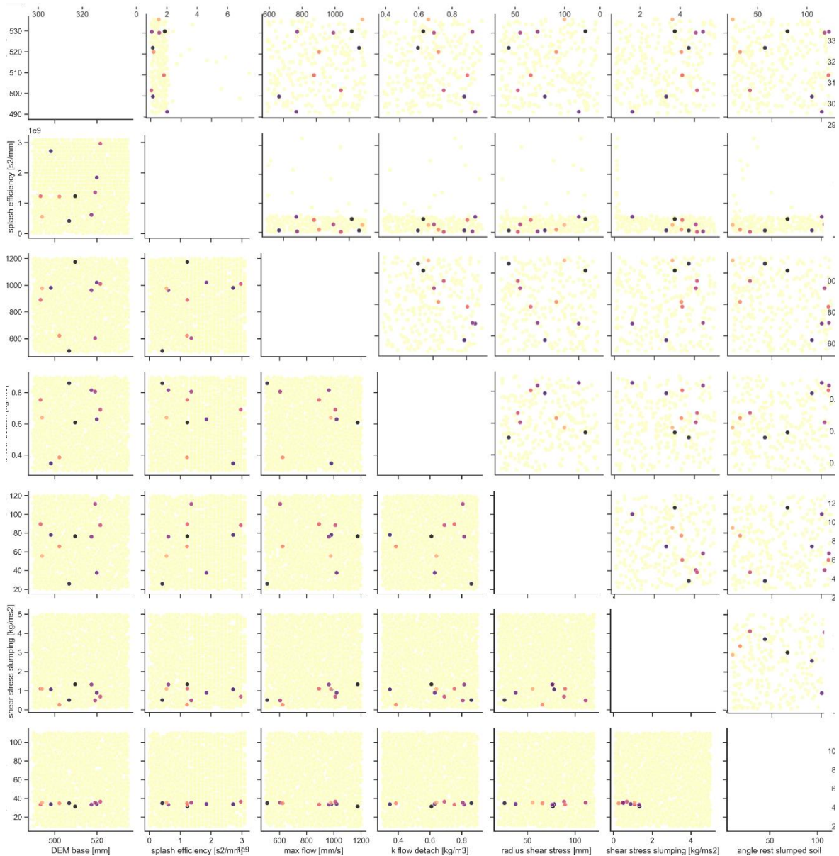
Figure 9: Parameter values of best 10 models considering all objective functions – lower triangle corresponds to the laboratory experiment and upper triangle to the field experiment. The colours help to identify points belonging to the same model run.
