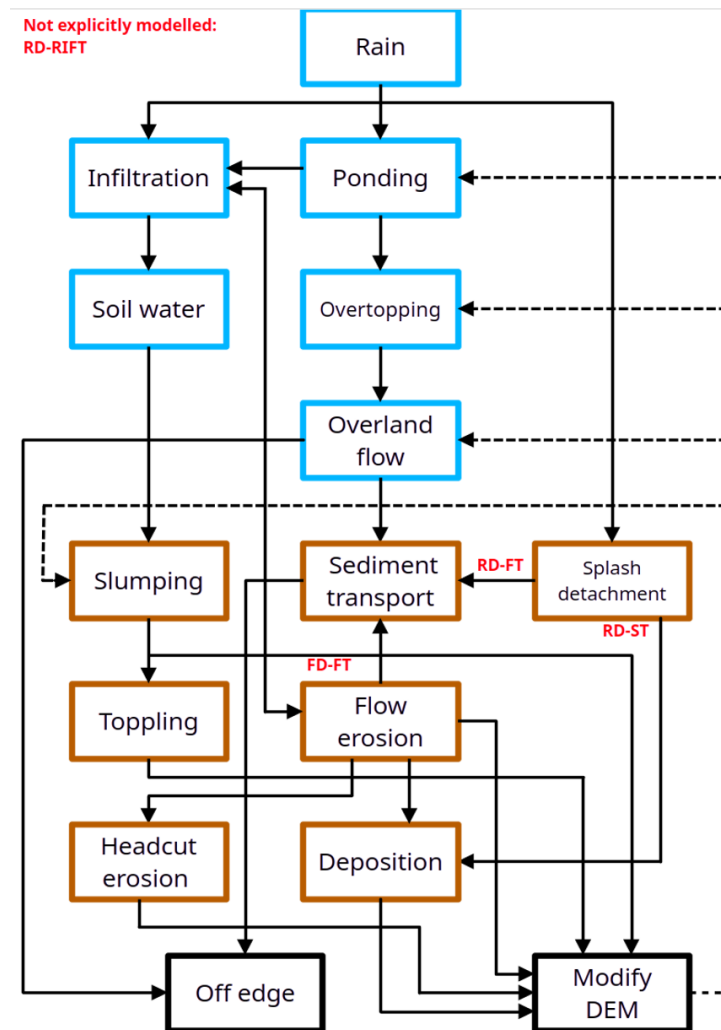
Figure 3: Flow chart of RillGrow. Blue-edged boxes indicate hydrological processes or stores, brown-edged boxes indicate erosional processes, black-edged boxes are model specific. The codes (RD-ST, FD-FT etc.) describe erosional subprocesses, see Kinnell (2001). Plain black lines represent process linkages, dashed black lines represent feedback.
