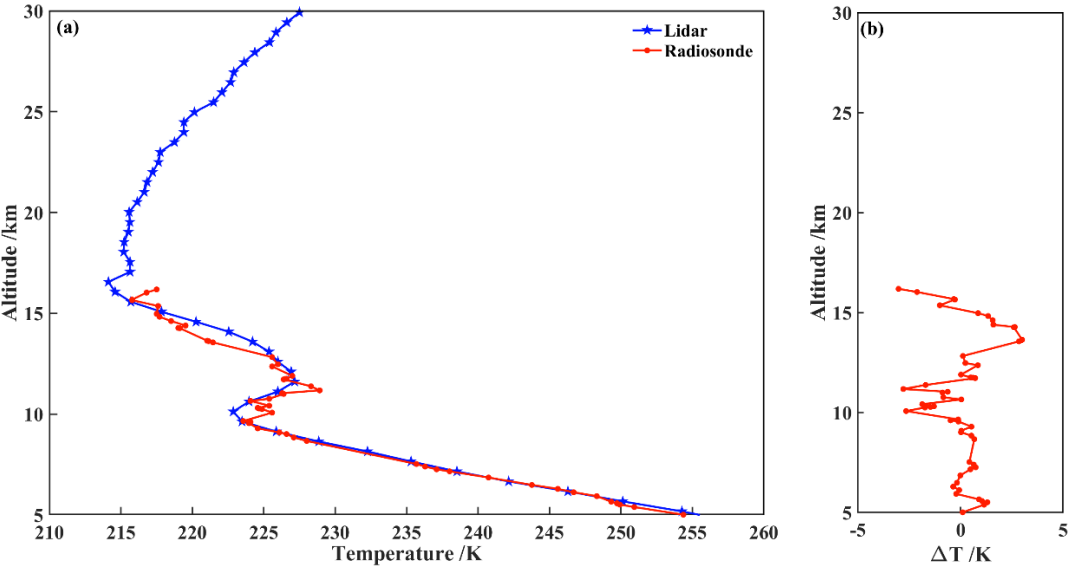
Figure 5: The results of atmospheric temperature measurements from 5 km to 30 km altitude (2024.03.10 0:30~1:00). (a) Comparison between lidar and radiosonde; (b) Deviation profile.
