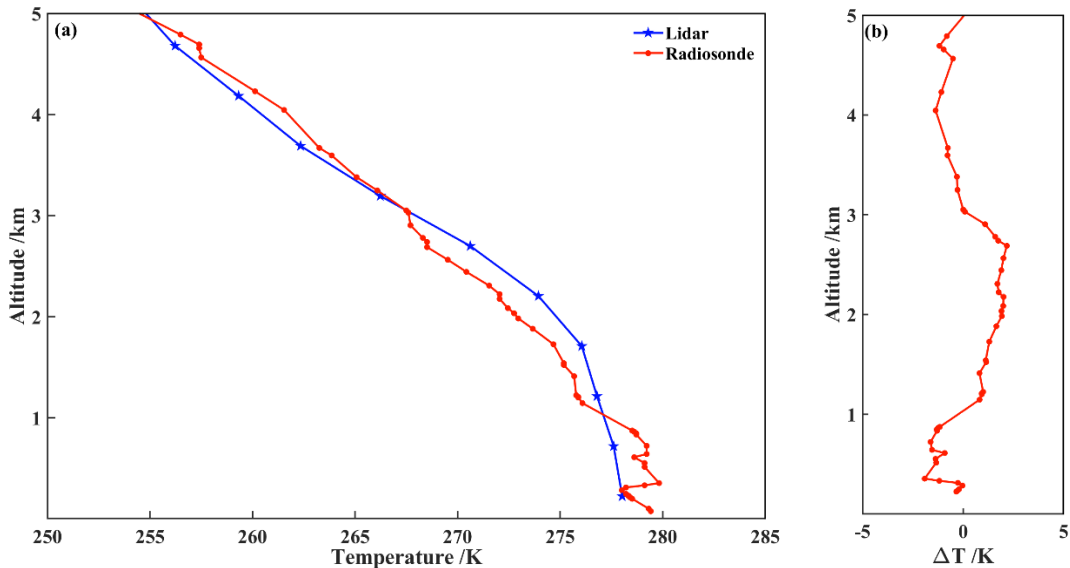
Figure 4: The atmospheric temperature measurements result from the surface to 5 km altitude. (a) Comparison between lidar and radiosonde; (b) Deviation profile.
