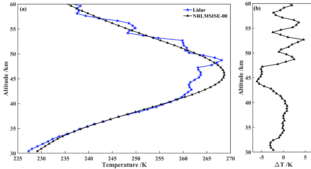
Figure 6: The results of atmospheric temperature measurements from 30 km to 60 km altitude (2024.03.10 0:30-1:00 LT). (a) Comparison between lidar and model; (b) Deviation profile.
