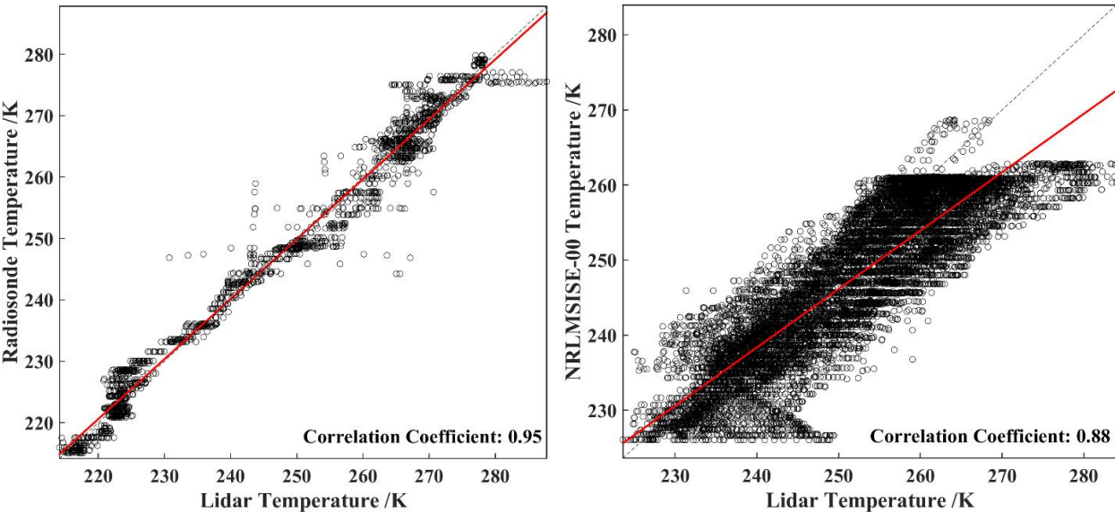
195 Figure 7: Correlation analysis results. (a) Correlation of atmospheric temperature between lidar and radiosonde from the surface to 16 km altitude. (b) Correlation of atmospheric temperature between lidar and NRLMSISE-00 atmospheric model from 30 km to 60 km altitude.
