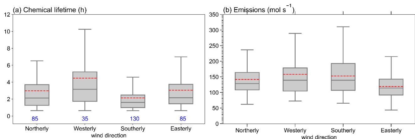
340 Figure 7: Boxplots of estimated NO x (a) chemical lifetimes and (b) emissions over Wuhan are categorized into four groups based on wind direction. For each box, the middle line indicates the median; the box top and bottom indicate the upper and lower quartiles, respectively; the whiskers indicate the farthest nonoutlier values; and the means are presented with red dashed lines. The number of days in each category is listed in blue.
