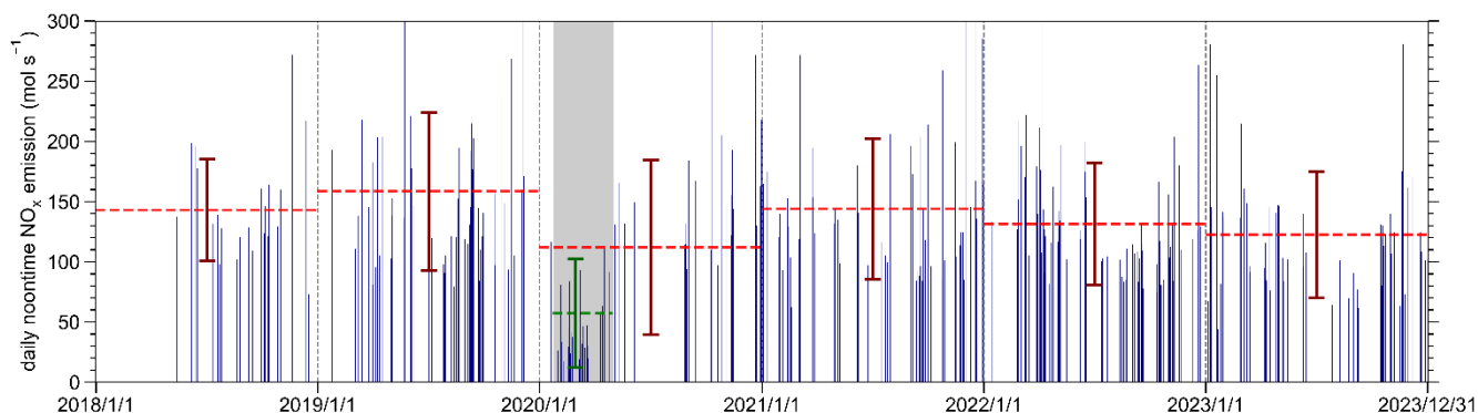
320 Figure 6: Daily noontime \text{NO}_x emissions over Wuhan on the days with valid estimation from 13 May 2018 through 31 December 2023. The annual mean emissions for each year are marked as red dashed lines. The green dashed line represents the mean \text{NO}_x emission during the COVID-19 lockdown-influenced period. The error bars denote the emission standard deviation for each time frame. The COVID-19 lockdown-influenced period is shaded in grey.
