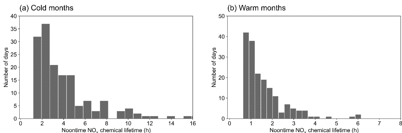
235 Figure 3: Distribution of estimated NO x chemical lifetimes over Wuhan in (a) cold months and (b) warm months.
