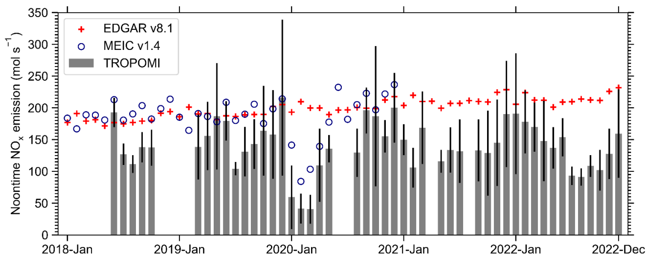
215 Figure 2: Monthly NO x emissions estimated with the TROPOMI data (grey columns), reported by EDGAR v8.1 (red pluses) and MEIC v1.4 (blue circles) from 2018 to 2022 (from 2018 to 2020 for MEIC v1.4). The emissions of EDGAR v8.1 and MEIC v1.4 are scaled to the noontime emission intensities to keep in consistent with TROPOMI. The TROPOMI monthly mean is calculated only when three or more days are available. Thus, the comparison is unavailable for several months. The error bars on the TROPOMI estimations represent the standard deviation of the daily NO x emissions in each month.
