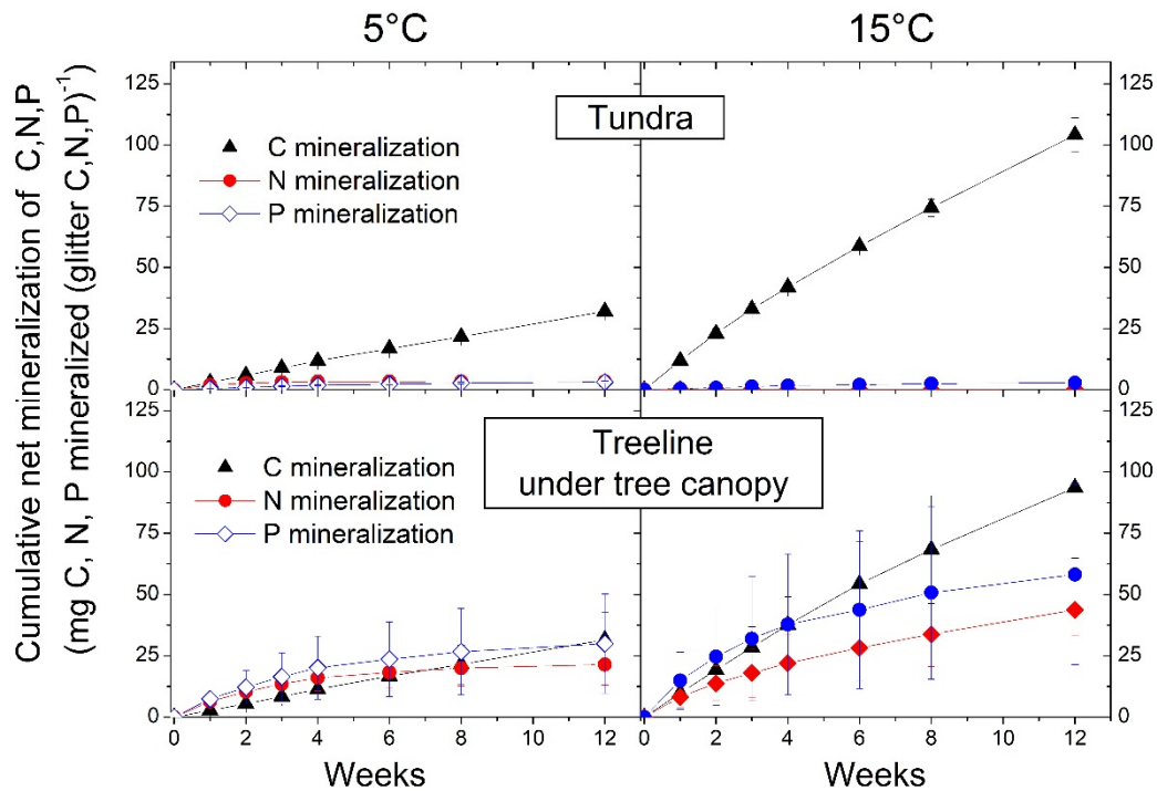
Figure 1: Cumulative potential net C, N, and P mineralization from the litter layer of the treeline ecotone in the South Urals at 5°C and 15°C during 12 weeks following a 3-week long preincubation at 15°C. Means and standard errors of three replicates. Cumulative values after 12 weeks of all vegetations types along the elevation gradient in the Khibiny mountains and South-Urals are shown in Figure 2.
