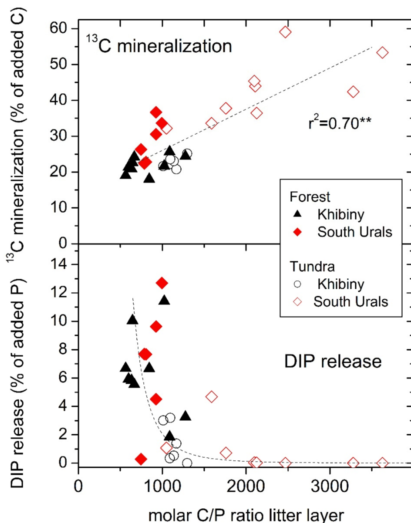
Figure 8: Relationship between the molar C:P ratio in the litter layer and the mineralization of ^{13}\text{C} from added ^{13}\text{C} labelled glucose-6-phosphate (G6P) and and additional the net release of dissolved inorganic P (DIP) following the G6P addition in the tundra and forest of the Khibiny Mountains and the South Urals. DIP-release is fitted to an threshold-type function ( y=x/1000)^5 ; r^2=0.38^{**} ).
