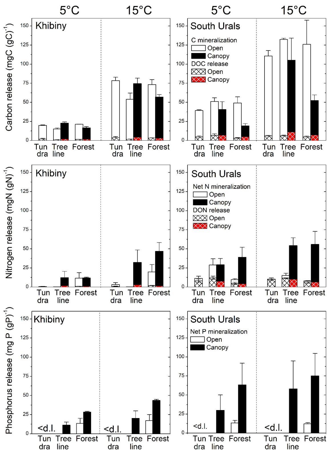
Figure 2: Cumulative net mineralization of carbon, nitrogen and phosphorus and release of organic carbon and nitrogen (DOC and DON) from the litter layer along elevation gradients across the treeline ecotone in the Khibiny mountains (left panels) and South-Urals (right panels) at 5°C and 15°C during 12 weeks of incubation. Means and standard errors of three replicates. Open land are areas without tree canopy consisting of a tundra vegetation in the tundra and at treeline, but forbs in the forest.
