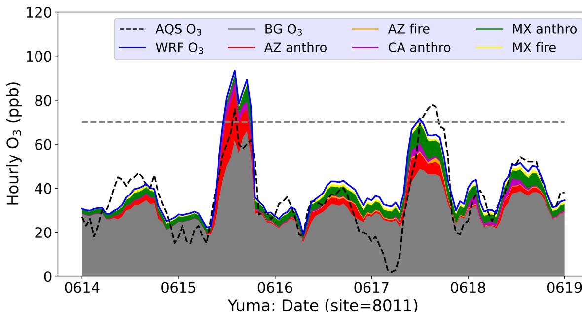
Figure 9. Hourly O 3 concentrations (in ppb) at the Yuma monitoring site (site number: 04-027-8011) between 14-19 June 2021, at local time. The dashed black line represents observed O 3 levels from the AQS, while the solid blue line shows WRF-Chem simulated O 3 concentrations. Shaded areas indicate contributions from various sources: background O 3 (gray), Arizona wildfires (orange), anthropogenic emissions from Mexico (green), anthropogenic emissions from Arizona (red), anthropogenic emissions from California (purple), and Mexico wildfires (yellow).
