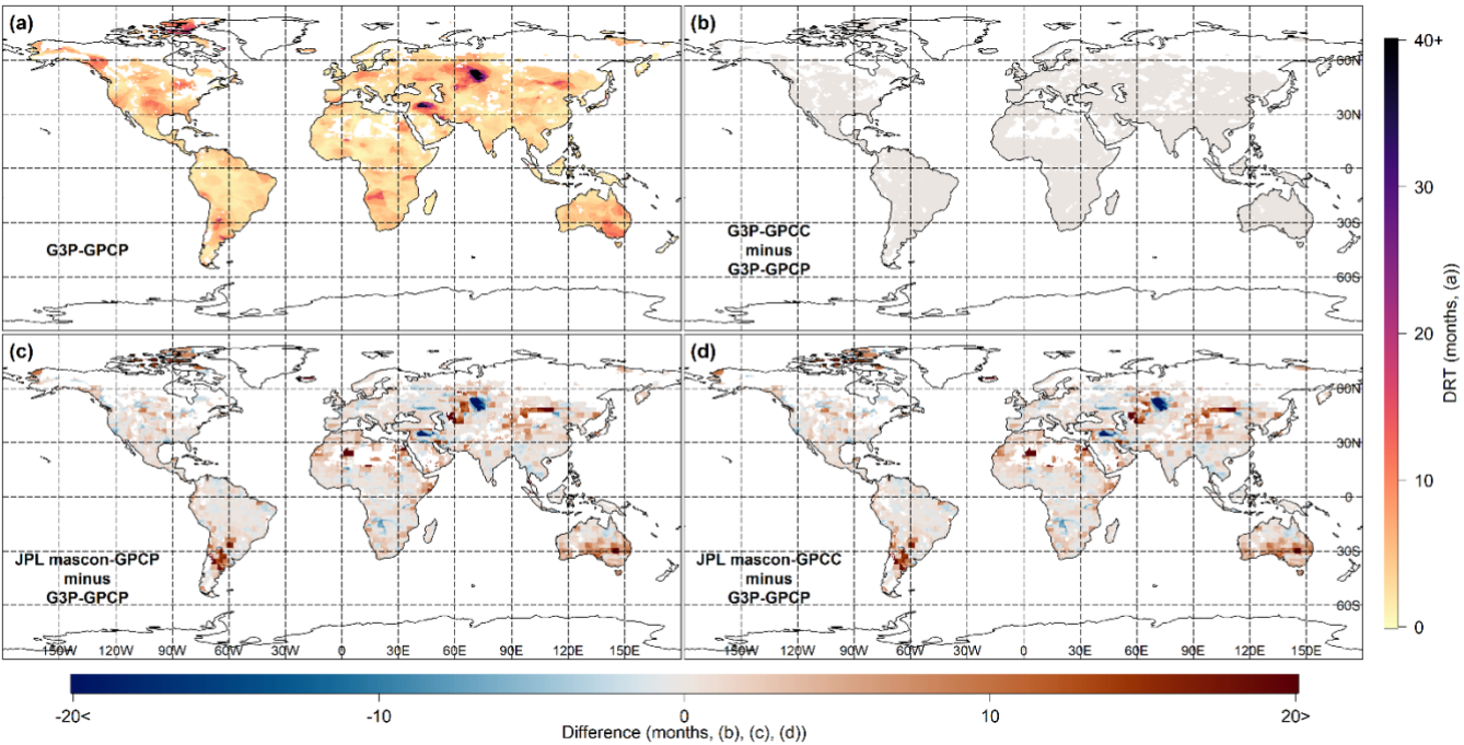
530 Figure A1. Display of the standard error of DRT estimates based on the storage deficit obtained from different dTWSA (i.e., G3P, JPL mascon) and cdPA (i.e., GPCP, GPCC) datasets. (a) Standard error for dTWSA from G3P and cdPA from GPCP (G3P–GPCP). Differences in standard error relative to G3P–GPCP for (b) G3P–GPCC, (c) JPL mascon–GPCP, and (d) JPL mascon–GPCC.
