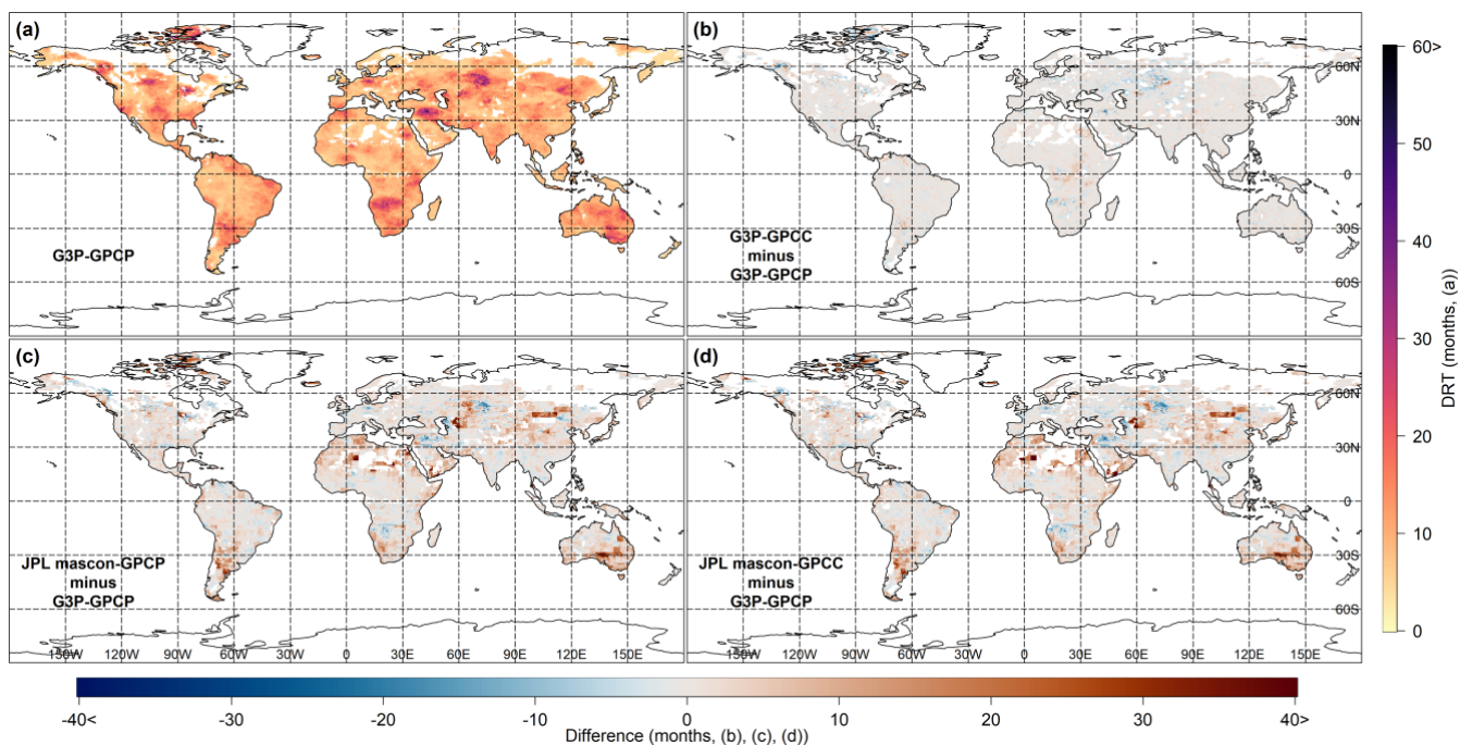
Figure 5. Representation of mean drought recovery time (DRT) estimates based on storage deficit method, obtained from different dTWSA (i.e., G3P, JPL mascon) and cdPA (i.e., GPCP, GPCC) datasets. (a) DRT estimated using dTWSA from G3P and cdPA from GPCP (G3P-GPCP). Differences in DRT relative to G3P-GPCP for (b) G3P-GPCC, (c) JPL mascon-GPCP, and (d) JPL mascon-GPCC.
