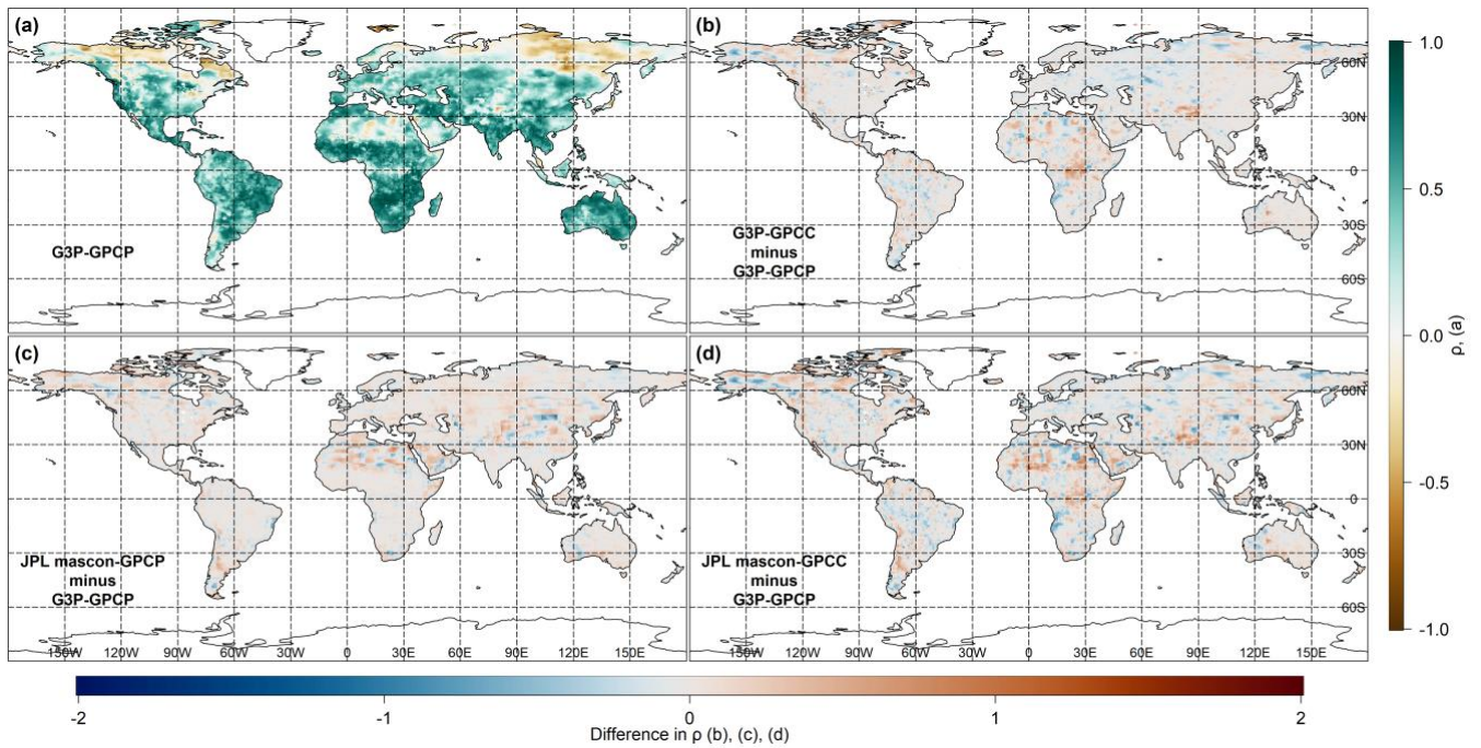
315 Figure 2. Representation of correlation coefficients between different dTWSA (i.e., G3P, JPL mascon) and cdPA (i.e., GPCP, GPCC) datasets. (a) Correlation coefficients obtained for dTWSA from G3P and cdPA from GPCP (G3P–GPCP). Differences in correlation coefficients relative to G3P–GPCP for (b) G3P–GPCC; (c) JPL mascon–GPCP; and (d) JPL mascon–GPCC. Please note that regions with negative correlations were removed from subsequent analyses.
