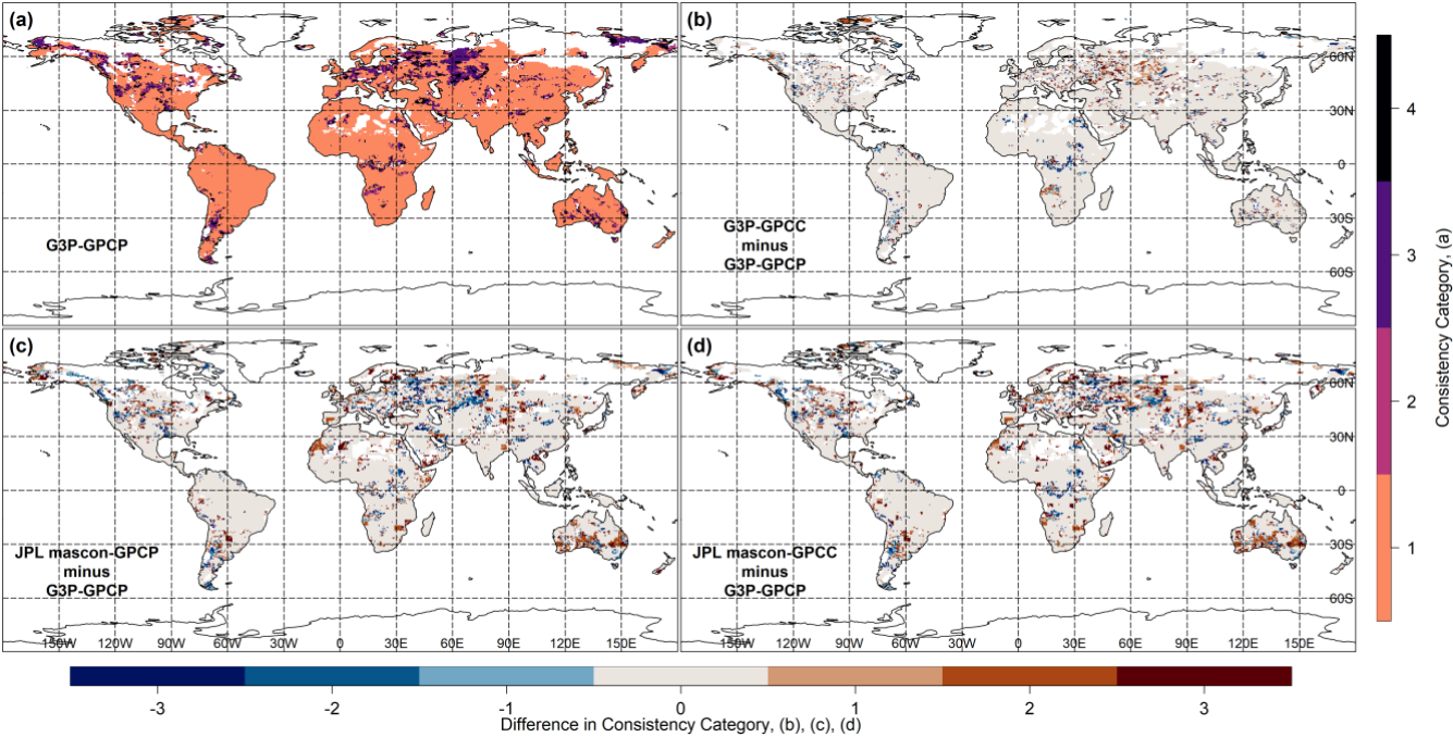
445 Figure 8. Representation of the consistency in DRT estimates (the class of the time difference in DRT values between two methods, see Table 1), obtained from the different dTWSA (i.e., G3P, JPL mascon) and cdPA (i.e., GPCP, GPCC) datasets. (a) consistency using dTWSA from G3P and cdPA from GPCP (G3P–GPCP), and differences in consistency class relative to G3P–GPCP for (b) G3P–GPCC, (c) JPL mascon–GPCP, and (d) JPL mascon–GPCC.
