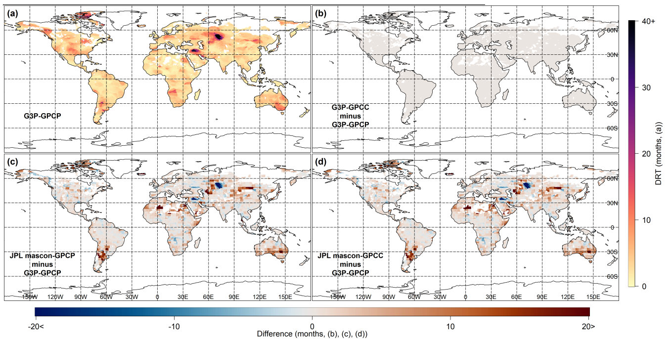
Figure A1. Display of the standard error of DRT estimates based on the storage deficit obtained from different dTWSA (i.e., G3P, JPL mascon) and cdPA (i.e., GPCP, GPCC) datasets. (a) Standard error for dTWSA from G3P and cdPA from GPCP (G3P–GPCP). Differences in standard error relative to G3P–GPCP for (b) G3P–GPCC, (c) JPL mascon–GPCP, and (d) JPL mascon–GPCC.
