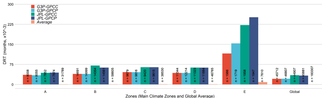
Figure A3. Standard error for average DRT estimates based on (a) storage deficit and (b) required precipitation amount for various climate zones from two different dTWSA (i.e., G3P and JPL mascon) and two different cdPA (i.e., GPCP and GPCC) products calculated for Equatorial (A); Arid (B); Warm Temperate (C); Snow (D); and Polar (E) as given by the Köppen-Geiger classification.
