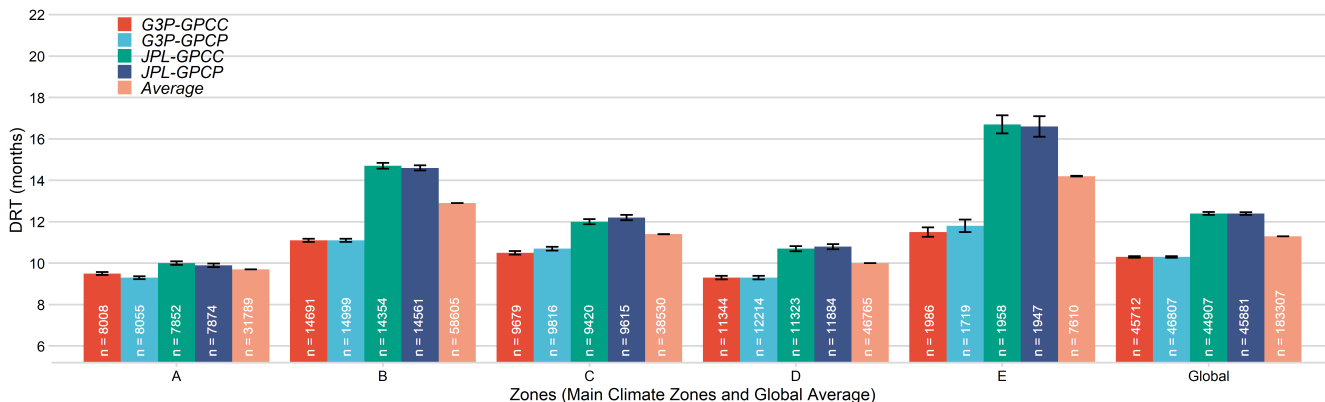
Figure 7. Average DRT estimates based on (a) storage deficit and (b) required precipitation amount for various climate zones from two different dTWSA (i.e., G3P and JPL mascon) and two different cdPA (i.e., GPCP and GPCC) products calculated for Equatorial (A); Arid (B); Warm Temperate (C); Snow (D); and Polar (E) as given by the Köppen–Geiger classification.
