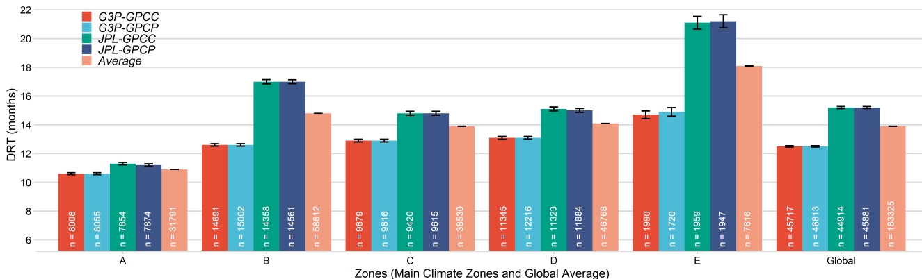
(b) DRT Based on Required Precipitation Amount
