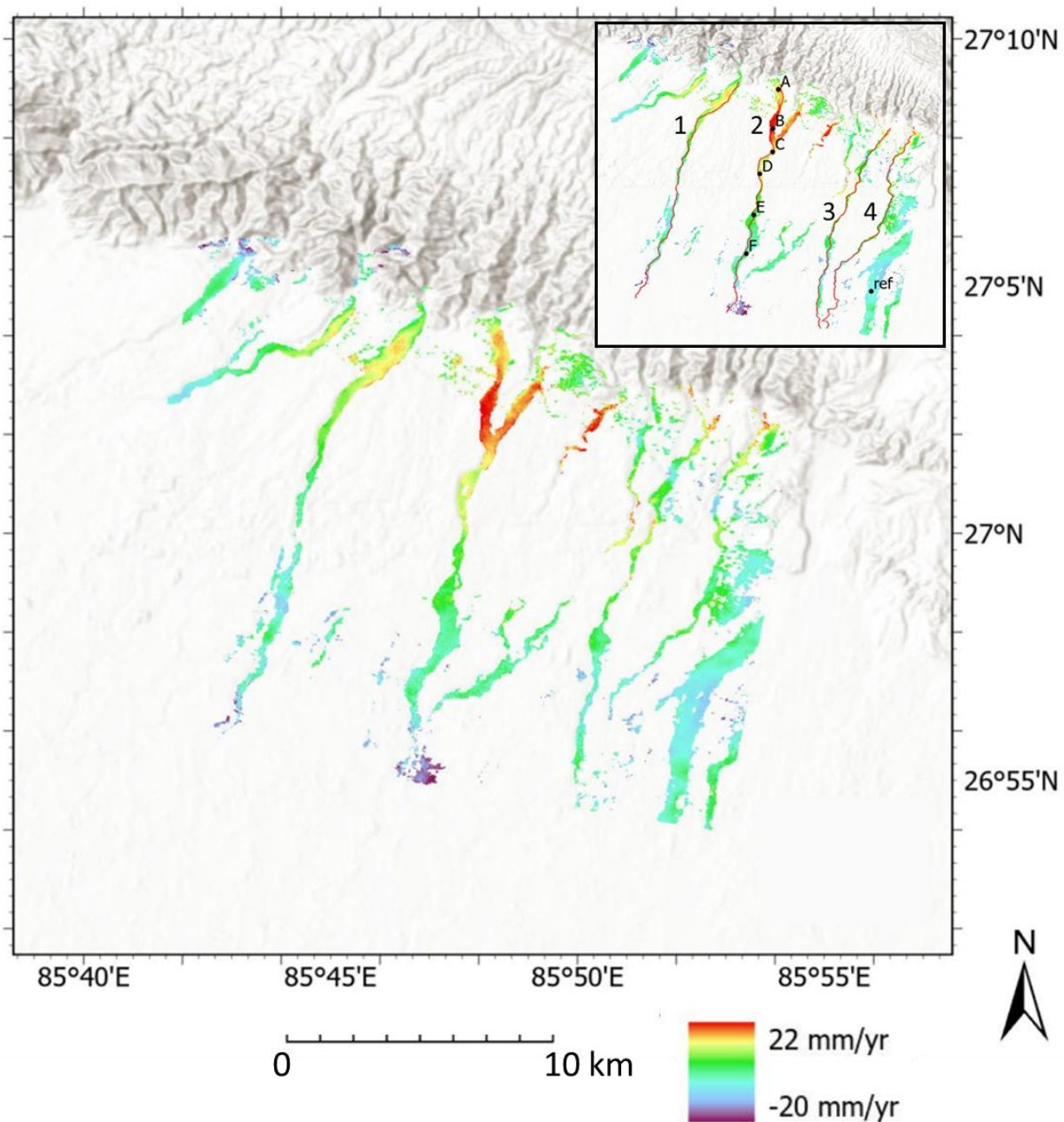
355 Figure 11: Spatial distribution of elevation change (2016 – 2021) at 20 m resolution for dry gravel riverbeds. An inset within the figure provides a detailed annotations. The results show the positive elevation change broadly decreasing with distance from the mountain front. The 20 m resolution SAR dataset focuses solely on mapping the rate of elevation change of dry river channels based on the residual topographic phase. Basemap data sources: ESRI World Topographic Basemap with hillshade illumination.
