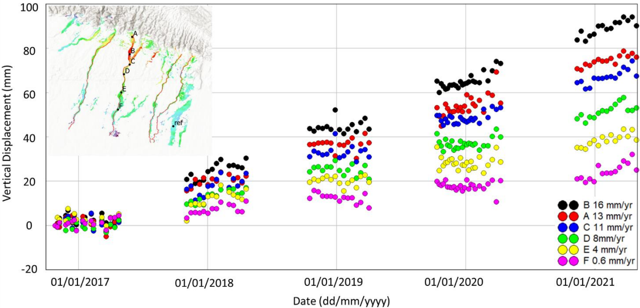
445 Figure 16: The SBAS-InSAR (20 m resolution) time-series along river 2 shows positive elevation changes. The June to September gap corresponds to the monsoon season. The inter-seasonal displacements shown in the time series are predominantly due to sediment aggradation. The fluctuations in the measurement points during the dry period could be due to a combination of noise and varying perpendicular baselines, which cause variations in topographic phase ambiguity. Basemap data sources: ESRI World 450 Topographic Basemap with hillshade illumination.
