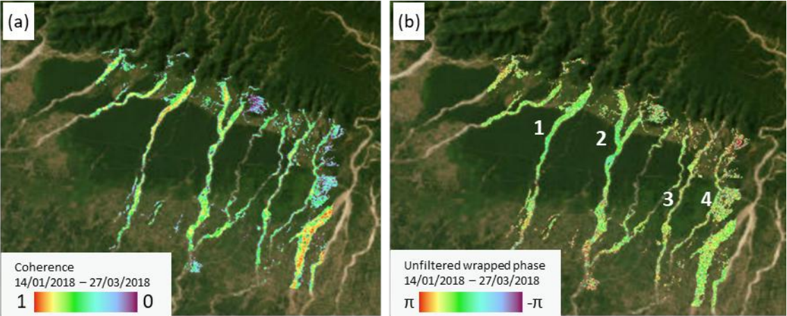
245 Figure 6: Short timespan interferograms' (acquired on dates 14/01/2018 and 27/03/2018, 72 days) (a) coherence and (b) unfiltered wrapped phase (20 m resolution, 0.2 coherence masked). Phase changes between adjacent pixels is relatively small and continuous. The continuous shifts in colour along the river shows a smooth, low phase gradient feature that contributes to a more accurate phase unwrapped interferogram. © Google Earth
