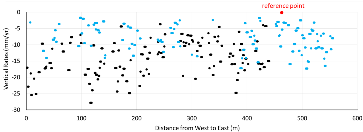
425 Figure 15: Basin transects of the InSAR analysis (northern black and southern blue lines in Fig. 12) indicate high heterogeneity in the distribution of subsidence across the basin, potentially caused by water extraction. Values from cropland and villages are shown in the transect plot, while elevation changes along the riverbeds, affected by monsoon season interferograms are excluded. The reference point for InSAR processing, located near the blue transect, is projected onto the plot and marked with a red dot.
