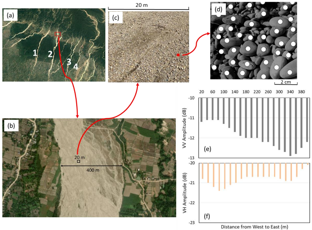
Figure 2: Illustration of the SAR diffuse backscatter from a dry gravel riverbeds. The returned SAR backscatter energy intensity is usually very small because the radar signal loses strength as it travels to the target and back. This illustration demonstrates that each 20 m 2 InSAR mapping pixel contains tens of thousands of distributed scatterers. The intensity of the SAR signal represents the sum of the distributed scatterers (white dots in (d)) in that pixel. Some areas may be covered by sand bars, which exhibit lower backscatter numbers compared to areas with larger pebbles, potentially resulting in lower backscatter intensity. Histogram (e) and (f) show the distribution of VV and VH amplitude value across the 400 m wide section of the river (b) from each 20m 2 pixel. The darker gravel bars in the east have relatively lower VV amplitude compared to the western gravel beds, and relatively higher VH amplitude, interpreted as due to minor vegetation. The decibel (dB) scale is logarithmic, and the logarithm of a small number (less than 1) is negative. The SAR amplitude values in decibels typically range from about -25 dB to 0 dB for most cases. For more detailed SAR polarimetric amplitude background theory, please refer to the supplementary section. © Microsoft
