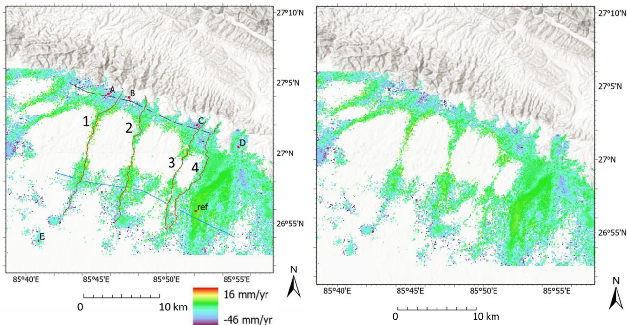
370 Figure 12: Spatial distribution of LOS displacement at 100 m resolution from 2016 – 2021 is shown as a background basin elevation change map, with and without annotations. This figure shows the negative elevation change in the basin. Due to the vegetation decorrelation effects, the results are sparse. The villages have denser pixels, attributable to the strong double bounce backscattering caused by houses. The 100 m resolution data are used only for mapping the basin based on the LOS displacement phase. For detailed 375 LiCSBAS processing implementation based on LOS displacement phase, please see the supplementary material. At the river, the data are considered unreliable due to contamination from monsoon season river water. Basemap data sources: ESRI World Topographic Basemap with hillshade illumination.
