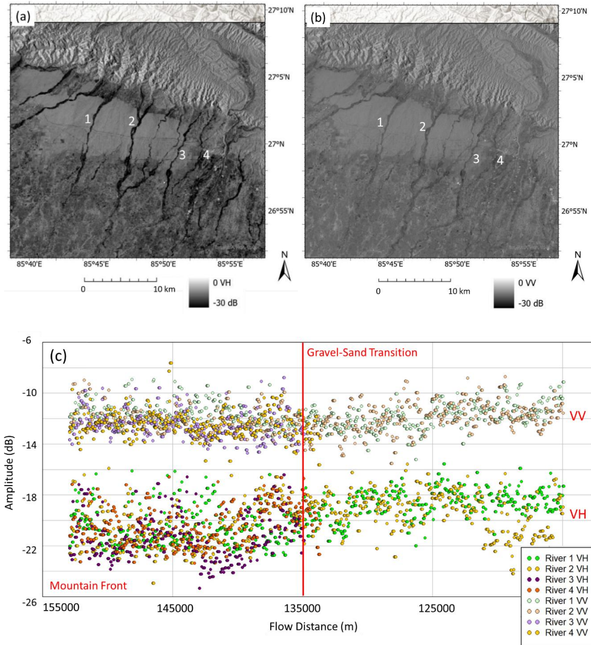
Figure 3: (a) Sentinel-1 SAR amplitude in decibels (dB) with VH (a) and VV (b) polarization, sourced from Google Earth Engine ( https://developers.google.com/earth-engine/datasets/catalog/COPERNICUS_S1_GRD ). Sentinel-1 is dual-polarized, providing only VV and VH polarized data. The mountain regions show strong backscatter amplitude mainly due to slope orientation. Slopes that face the radar look direction can return more backscatter energy back to the satellite sensor. The forest area has higher amplitude due to strong volume backscattering, but the forest and vegetation cover areas have low coherence due to the seasonal growth change. Along the river channel VV has a higher amplitude than VH. (c) Amplitude values were plotted along river channels and all aligned to start from the mountain front, indicating that the VV polarization has double the amplitude value compared to the VH polarization. The river mountain front is the point of exit of the river from the mountains where the channel abruptly widens. There is no clear amplitude change response to roughness change at the gravel to sand transition along the rivers. The mean
