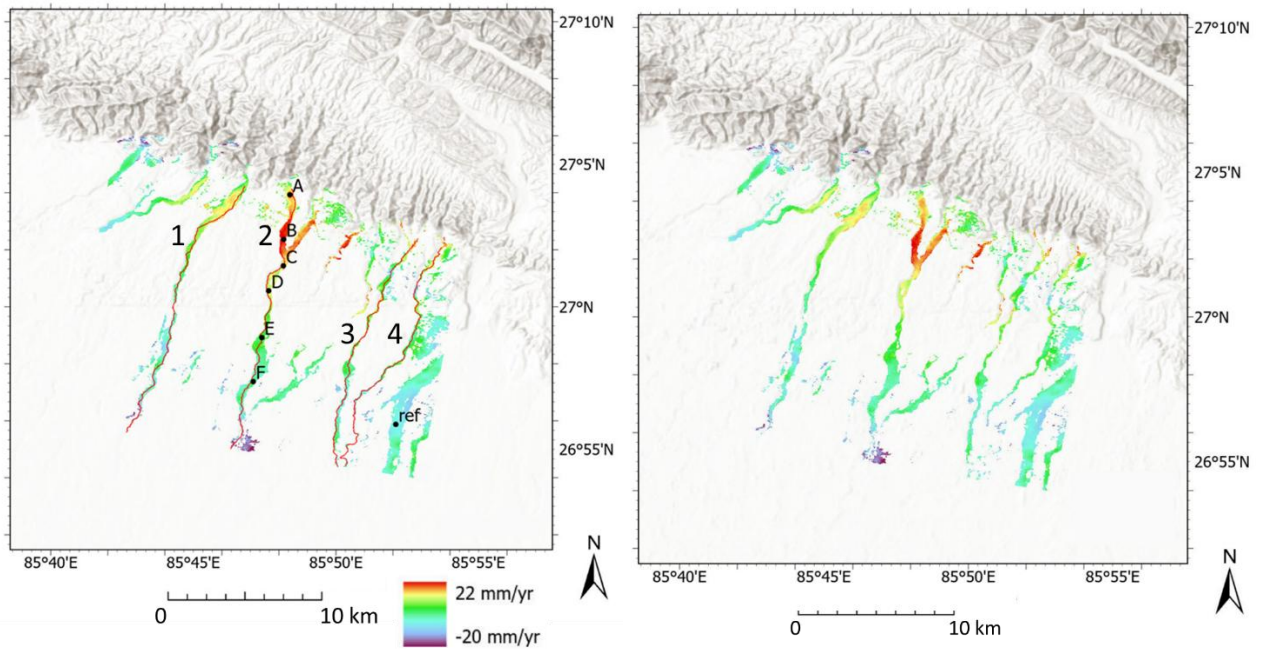
355 Figure 11: Spatial distribution of elevation change at 20 m resolution (2016 – 2021) for dry gravel riverbeds, shown on maps with and without annotations. The results show the positive elevation change broadly decreasing with distance from the mountain front. The 20 m resolution SAR dataset focuses solely on mapping the rate of elevation change of dry river channels based on the residual topographic phase. Basemap data sources: ESRI World Topographic Basemap with hillshade illumination.
