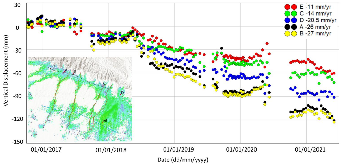
455 Figure 17: The SBAS-InSAR (100 m resolution) time-series in the floodplain shows a consistent pattern of negative elevation change, indicative of subsidence at each observed location. To ensure accuracy, there are no gaps in the network, which is connected by both short and long timespan interferograms. Basemap data sources: ESRI World Topographic Basemap with hillshade illumination.
