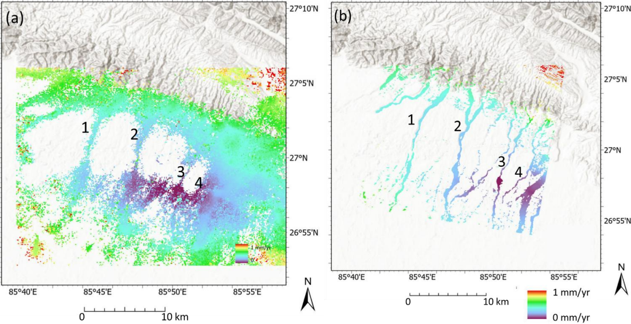
395 Figure 13: Standard deviation of the InSAR LOS velocity for 100 m resolution (a) and 20 m resolution (b). The standard deviation ranges from 0–1 mm/yr. The calculation of the velocity standard deviation assumes that all input pixel values from the InSAR images are reliable. For the 100 m resolution InSAR results at river channels, despite showing a positive elevation trend, the values are considered unreliable due to high noise contamination. This unreliability comes from noise in the InSAR images taken during the monsoon season. Consequently, the 100 m resolution InSAR results are solely employed for mapping basin elevation changes, while the 20 m resolution InSAR results are used to map changes in river channel elevation. Basemap data sources: ESRI World Topographic Basemap with hillshade illumination.
