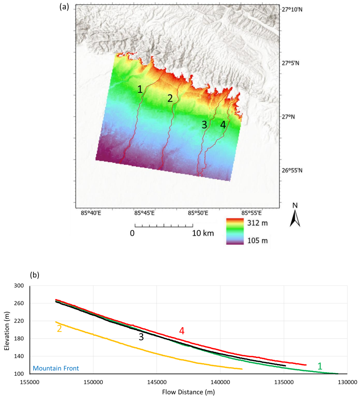
235 Figure 5: (a) The 30 m resolution SRTM DEM (© Esri). The terrain results in a gradient in the topographic phase values. This DEM was used to remove static topography phase during the interferogram calculation process, which is carried out using the GAMMA software as implemented by the LiCSAR (Lazecský et al., 2020). The residual topographic phase is derived by subtracting the topographic phase from the year 2000 SRTM DEM. (b) River long profiles showing no obvious evidence of knick points. From the mountain front to the gravel-sand transition, the elevation of the river channel decreases by around 150 m. The exact season when
