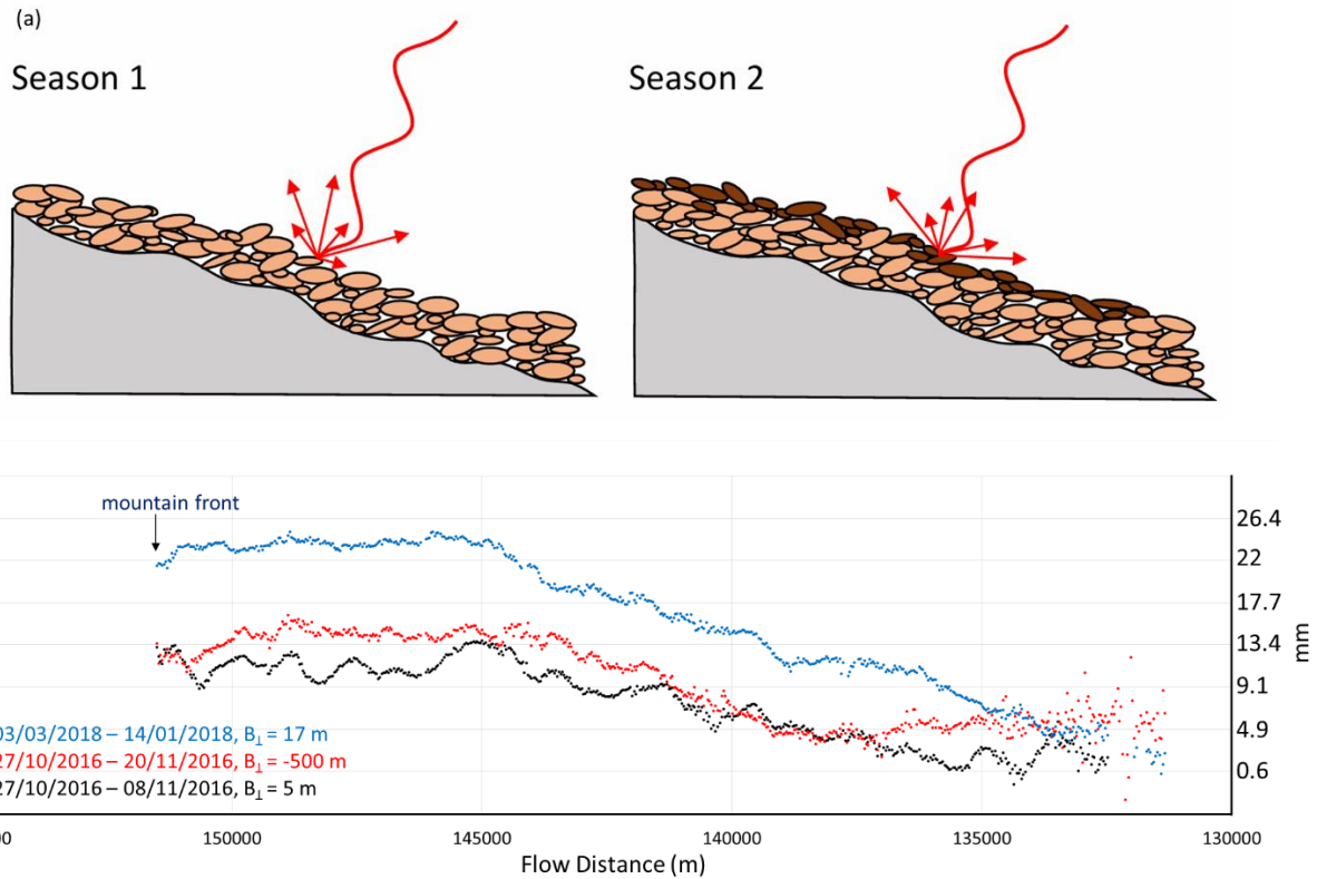
Figure 10: (a) Illustration of the annual increase in dry gravel riverbed topographic elevation due to sediment aggradation. Dark brown pebbles show accumulation in season 2. (b) Changes in the residual topographic phase along river 2, influenced by sediment aggradation and perpendicular baseline variations. The filtered unwrapped phase values are plotted along river 2, comparing residual topographic phase observations with different perpendicular baselines from the same year (black and red curves), and the residual topographic differences between 2016 and 2018 with similar perpendicular baseline (blue and black curves). From the same year, the large baseline (red) measured topographic phases are higher than smaller baseline measurements (black). This indicates that a larger perpendicular baseline increases the sensitivity of the interferometric phase to topographic elevation. Comparing different years, the year 2018 (blue) has higher residual topographic phase values, likely due to sediment aggradation.
