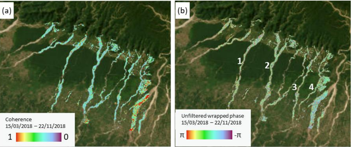
250 Figure 7: Long timespan interferograms' (acquired on dates 15/03/2018 and 22/11/2018, 252 days) (a) coherence and (b) unfiltered wrapped phase (b) (20 m resolution, 0.2 coherence masked). Based on coherence data, the months from November to March are identified as the driest in the study area. Most regions shown in blue on (a) display coherence values below 0.3, indicating that they are insufficient for obtaining reliable interferometric phase. Areas of high coherence on the eastern side are depicted in red on (a) and correspond to an embanked, inactive gravel riverbed. © Google Earth 255
