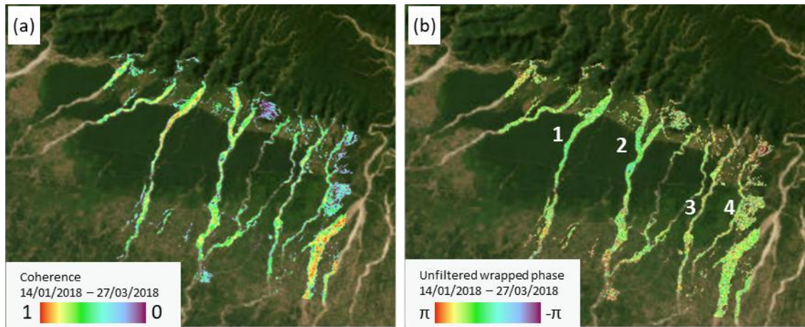
250 Figure 6: Short timespan interferogram coherence (a) and unfiltered wrapped phase (b) (20 m resolution, 0.2 coherence masked, acquired on dates 14/01/2018 and 27/03/2018, 72 days). Phase changes between adjacent pixels is relatively small and continuous. The continuous shifts in colour along the river shows a smooth, low phase gradient feature that contributes to a more accurate phase unwrapped interferogram. © Google Earth
