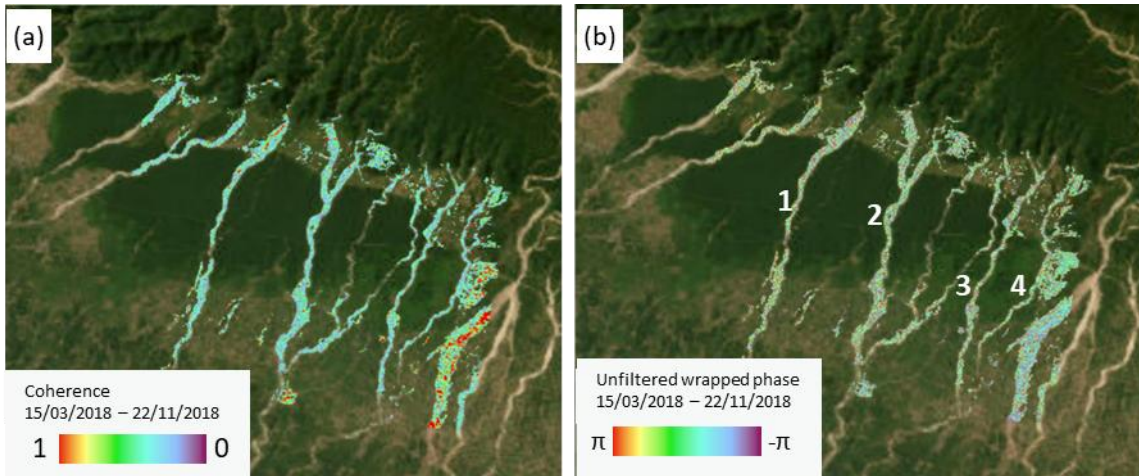
255 260 Figure 7: Long timespan interferogram coherence (a) and unfiltered wrapped phase (b) (20 m resolution, 0.2 coherence masked, acquired on dates 15/03/2018 and 22/11/2018, 252 days). Based on coherence data, the months from November to March are identified as the driest in the study area. Most regions shown in blue on (a) display coherence values below 0.3, indicating that they are insufficient for obtaining reliable interferometric phase. Areas of high coherence on the eastern side are depicted in red on (a) and correspond to an embanked, inactive gravel riverbed. © Google Earth
