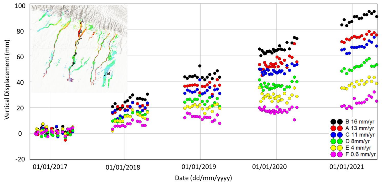
440 Figure 16: The SBAS-InSAR (20 m resolution) time-series along river 2 shows positive elevation changes. The June to September gap corresponds to the monsoon season. The inter-seasonal displacements shown in the time series are predominantly due to sediment aggradation. The fluctuations in the measurement points during the dry period could be due to a combination of noise and varying perpendicular baselines, which cause variations in topographic phase ambiguity. Basemap data sources: ESRI World Topographic Basemap with hillshade illumination. 445
