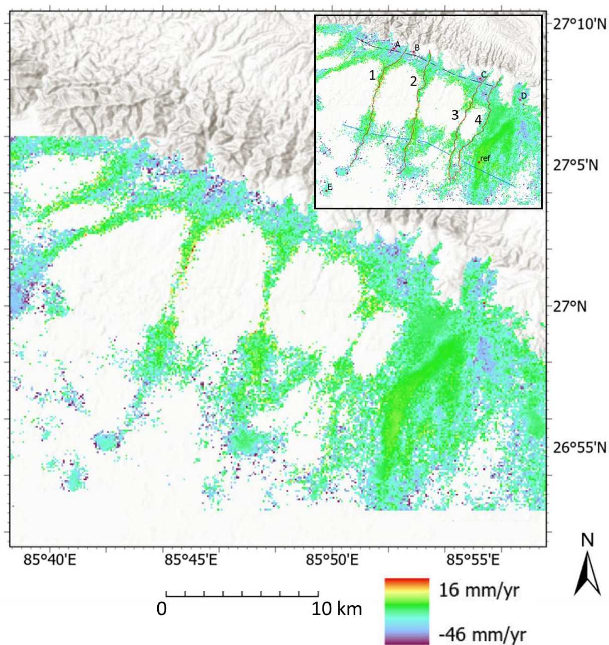
Figure 12: Spatial distribution of LOS displacement (2016 – 2021) at 100 m resolution for the basin. An inset within the figure provides a detailed annotations. This figure shows the negative elevation change in the basin. Due to the vegetation decorrelation effects, the results are sparse. The villages have denser pixels, attributable to the strong double bounce backscattering caused by houses. The 100 m resolution data are used only for mapping the basin based on the LOS displacement phase. For detailed LiCSBAS processing implementation based on LOS displacement phase, please see the supplementary material. At the river, the data are considered unreliable due to contamination from monsoon season river water. Basemap data sources: ESRI World Topographic Basemap with hillshade illumination.
