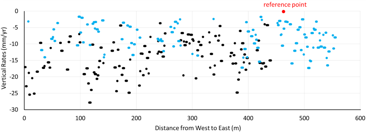
420 Figure 15: Basin transects of the InSAR analysis (northern black and southern blue lines in Fig. 12) indicate high heterogeneity in the distribution of subsidence across the basin, potentially caused by water extraction. Values from cropland and villages are shown in the transect plot, while elevation changes along the riverbeds, affected by monsoon season interferograms are excluded. The reference point for InSAR processing, located near the blue transect, is projected onto the plot and marked with a red dot.
