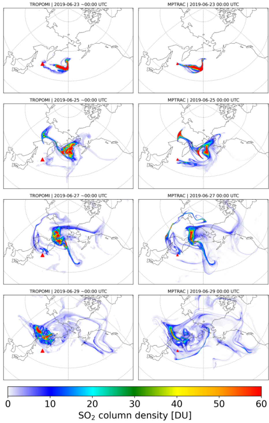
Figure 3. Evolution of \text{SO}_2 total column density distributions from 23 June 2019 to 30 29 June 2019 from the MPTRAC simulation with implicit chemistry scheme (right column) and TROPOMI satellite observations (left column). The red triangle marks the location of the Raikoke volcano.
