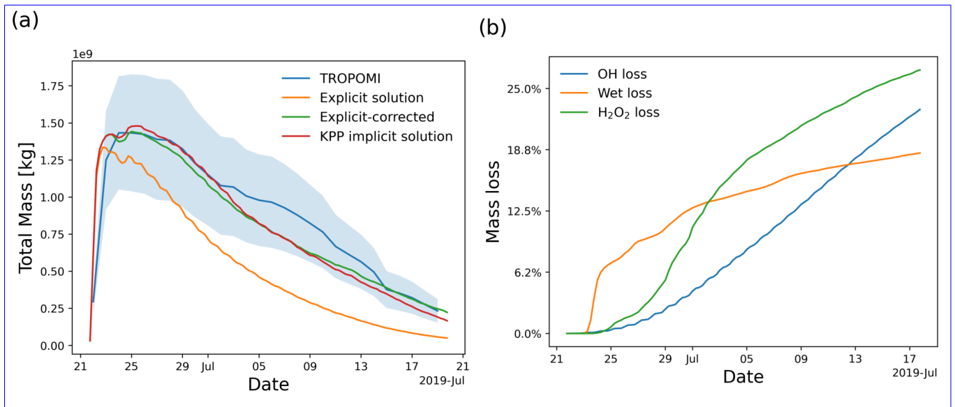
Figure 5. (a) Temporal evolution of the SO 2 total mass burden of the 2019 Raikoke eruption from TROPOMI measurements (blue curve, shading shows uncertainty range) and MPTRAC simulations with explicit solution (orange curve), simplified explicit solution with correction (green curve), and KPP implicit solution (red curve). (b) Estimates of SO 2 total mass loss of the Raikoke eruption due to OH oxidation (blue curve), wet deposition (orange curve), and H 2 O 2 oxidation (green curve) from the simplified explicit solution with correction.
