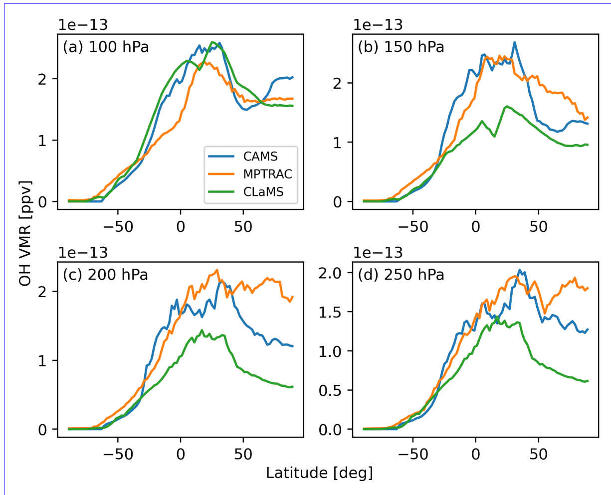
Figure 8. Zonal mean distributions of the OH field obtained from the CAMS reanalysis (blue curves), climatological data from the CLaMS model (green curves) and the MPTRAC simulation (orange curves) at pressure levels of 100 hPa (a), 150 hPa (b), 200 hPa (c) and 250 hPa (d) on 1 July 2019, 00:00 UTC.
