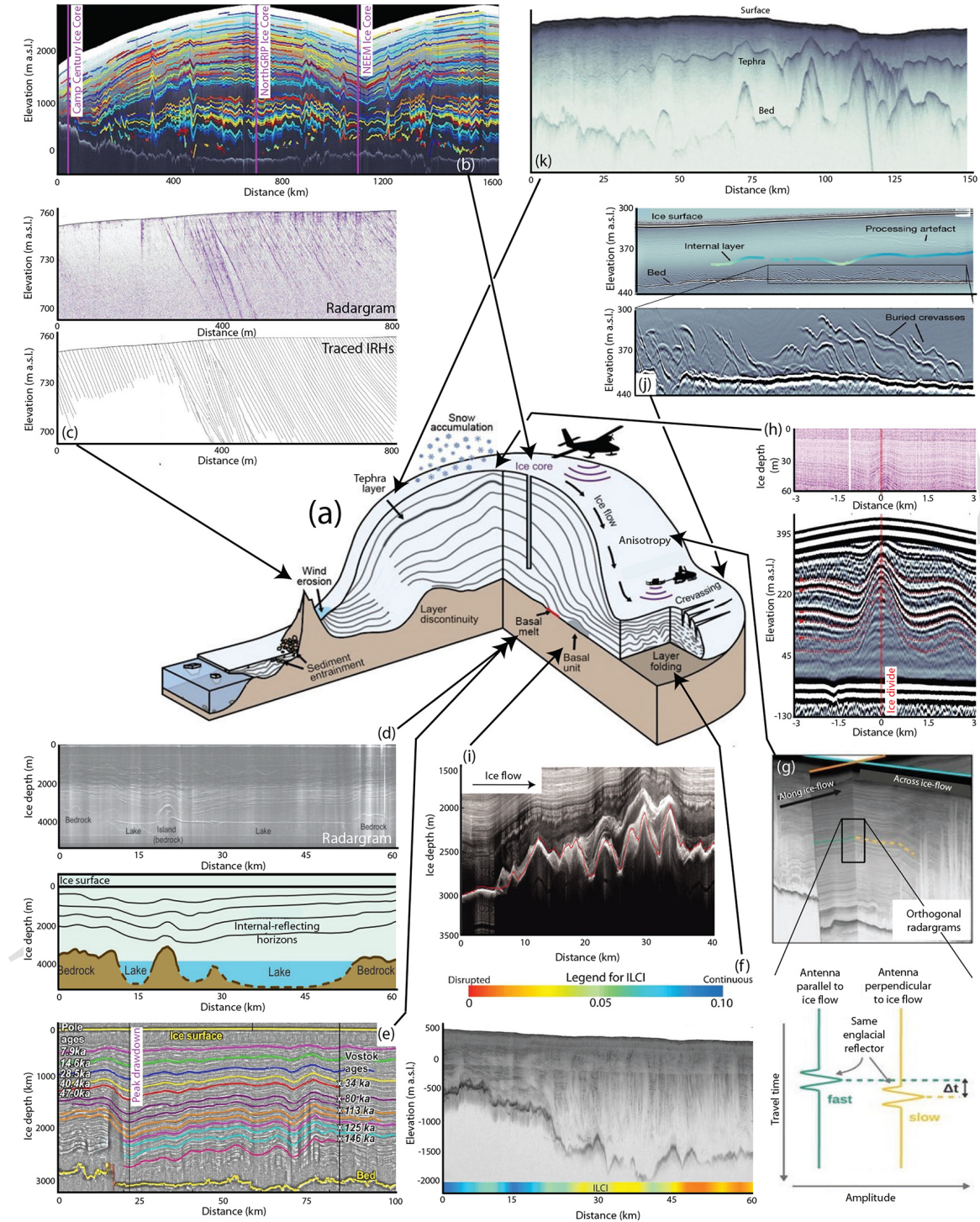
Figure 8. Schematic illustration of radiostratigraphic observations within an ice sheet and their scientific applications; panel (a) in the centre depicts typical ice-sheet locations for the applications shown in subsequent panels. (b) Connecting and validating ice cores in Greenland (after MacGregor et al., 2015a). (c) Imaging intersections of IRHs with ice surface in the region of surface wind scouring (after Winter et al., 2016). (d) Using isochrones to calculate basal melting across Subglacial Lake Vostok (after Siegert et al., 2001). (e) Using isochrone drawdown to locate region of elevated geothermal heat flux near the South Pole (after Jordan et al., 2018). (f) Application of the Internal Layering Continuity Index (ILCI) to quantify disruption (folding or warping) to otherwise continuous isochrones (after Bingham et al., 2015). (g) Using intersecting RES profiles to explore ice anisotropy (after Gerber et al., 2023). (h) Raymond Arch imaged in near-surface (top panel) and deep RES across Derwael Ice Rise, Dronning Maud Land (after Drews et al., 2015). (i) Basal-ice units and suggested accreted basal ice in East Antarctica (after Bell et al., 2011). (j) Basal crevasses imaged in West Antarctica and used to date re-grounding of previously floating ice (after Kingslake et al., 2018). (k) Prominent tephra horizon imaged by RES across Pine Island Glacier, West Antarctica (after Corr and Vaughan, 2008).
