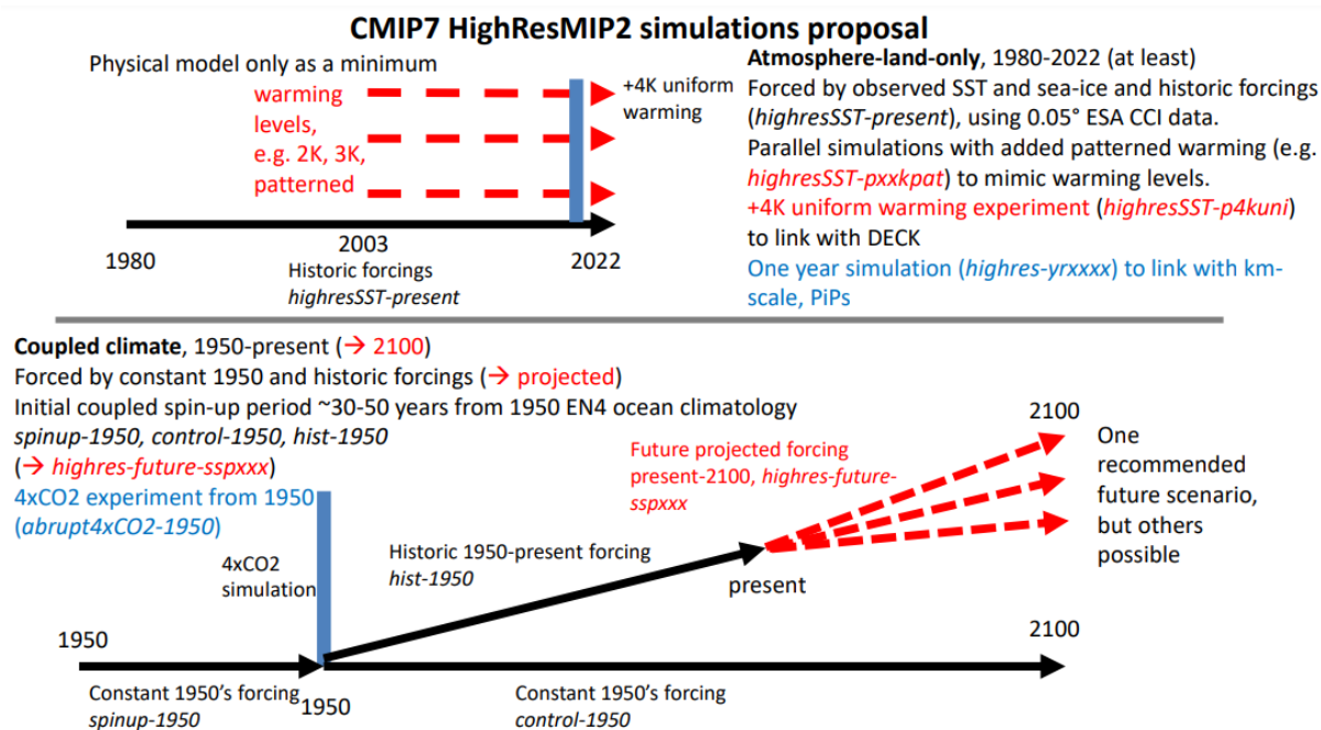
375 Figure 2: Illustration of the HighResMIP2 simulations in Tiers 1-5 for (upper) atmosphere-only and (lower) coupled model experiments.
