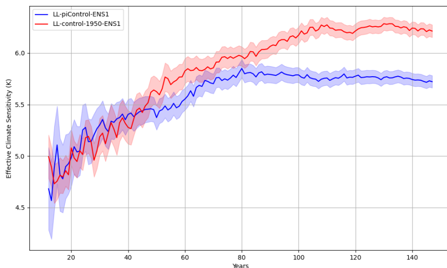
490 Figure 5: An illustrative example of model metrics enabled by new HighResMIP2 simulations: Effective Climate Sensitivity (EffCS) calculated with successively more years of data for two simulations, in this case a ~130-km atmosphere coupled to a ~100-km ocean. Blue uses the standard CMIP6 DECK piControl and abrupt-4xCO2 simulations to calculate EffCS over 150 years; Red uses the standard HighResMIP experimental design, 50 years of spinup-1950, and then control-1950 and abrupt4xCO2-1950 simulations. Using only 30 years of simulation clearly does not define the final (150 year) EffCS, but may at least give a useful lower bound. Any relationship across experimental designs will need more (multi-model) analysis.
