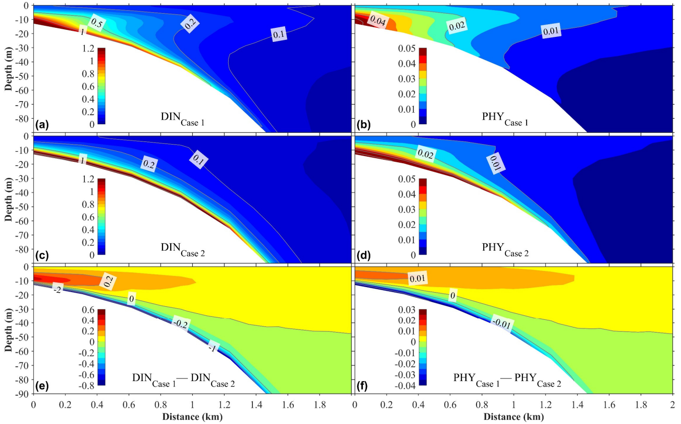
Figure 13: (a)–(d) illustrate the vertical distributions of the annual mean dissolved inorganic nitrogen ( DIN_{SGD} ) originating from submarine groundwater discharge (SGD) and the phytoplankton ( PHY_{SGD} ) it supports under two scenarios. Panels (a) and (b) correspond to Case 1, where the buoyancy effect of SGD is included in the hydrodynamic model, while panels (c) and (d) correspond to Case 2, where the buoyancy effect of SGD is excluded. (e) and (f) show the differences in DIN_{SGD} and PHY_{SGD} between Case 1 and Case 2. The distance on the x-axis is measured from the shore.
