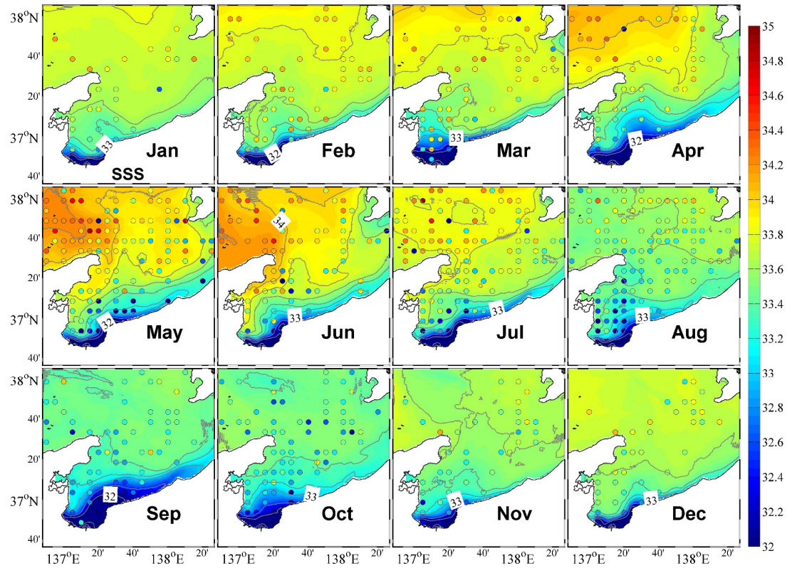
Figure 4: Monthly mean surface salinity. The circles represent observational data, whose color bar is shown on the right.
