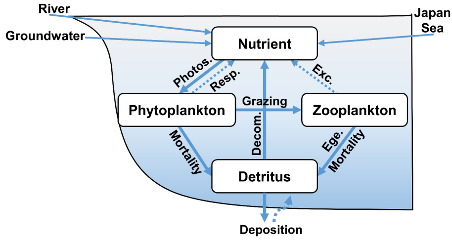
200 Figure 3. Biogeochemical processes in the ecosystem model. In this model, groundwater is released at the bottom of the sea. Photos., Resp., Exc., Ege., and Decom. represent Photosynthesis, Respiration, Excretion, Egestion, and Decomposition, respectively.
