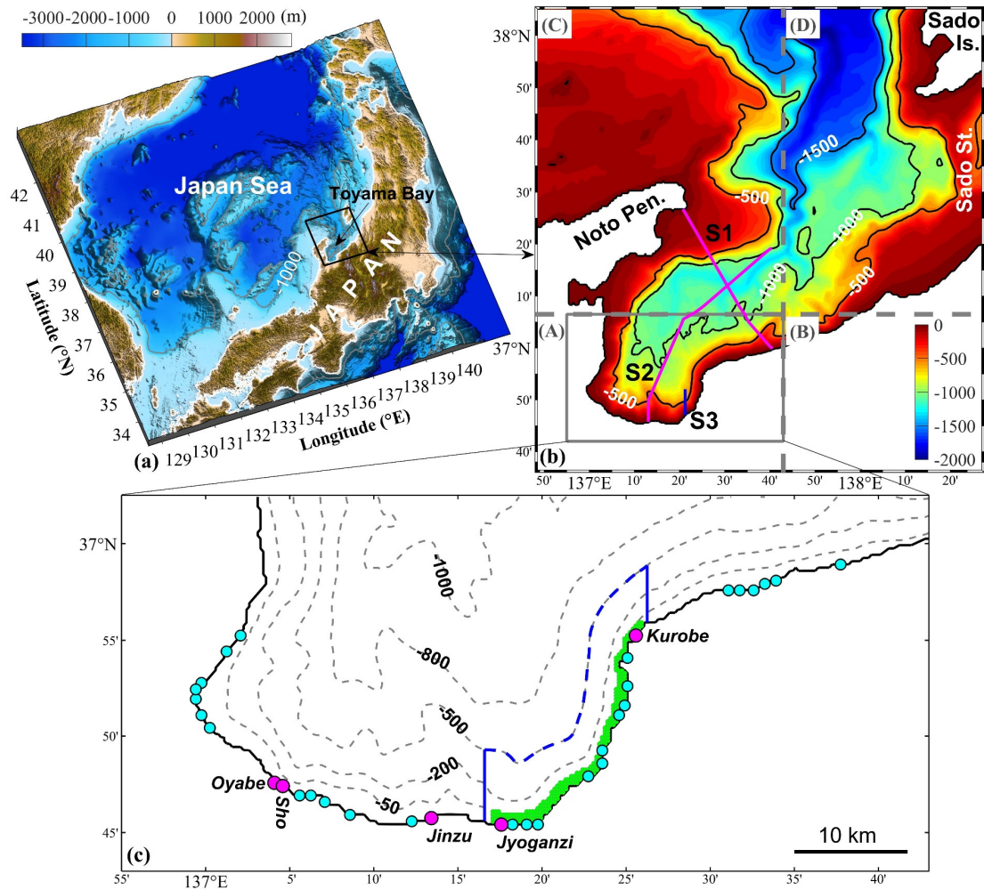
Figure 1: (a) Study area. (b) Model domain for Toyama Bay. Colors and contour lines represent indicate the water depth, with units in meters. The model domain was divided into four areas from (A) to (D) with different horizontal resolutions. The respective horizontal resolutions are (1) 300 m × 300 m, (2) 900 m × 300 m, (3) 300 m × 900 m, and (4) 900 m × 900 m. “Pen.”, “Is.”, and “St.” is the abbreviation of Peninsula, Island, and Strait respectively. The three lines S1, S2, and S3 represent the sections to show vertical distributions of the results. (c) The inner part of the bay. The circles indicate river mouths that supply freshwater and nutrients, with pink for first-class rivers and blue for second-class rivers. The green area means the location of submarine groundwater discharge (SGD). A uniform distribution of SGD over the grid points in this green area is assumed. The area inside the blue lines is used to calculate the inventories and material flows of SGD- and river-derived nutrients.
