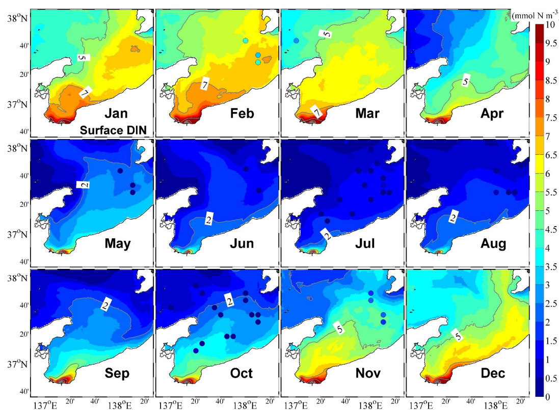
Figure 65: Monthly mean surface dissolved inorganic nitrogen (DIN). The color circles represent observational data.
