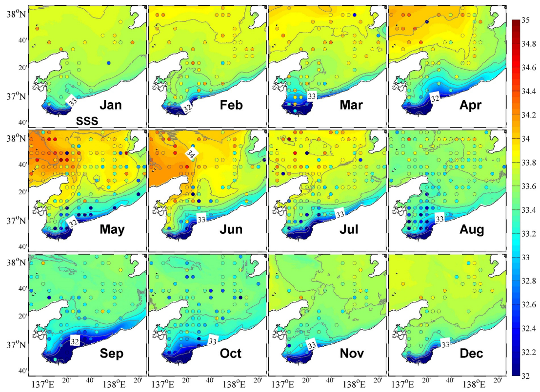
Figure 43: Monthly mean surface salinity. The circles represent observational data, whose color bar is shown on the right.
