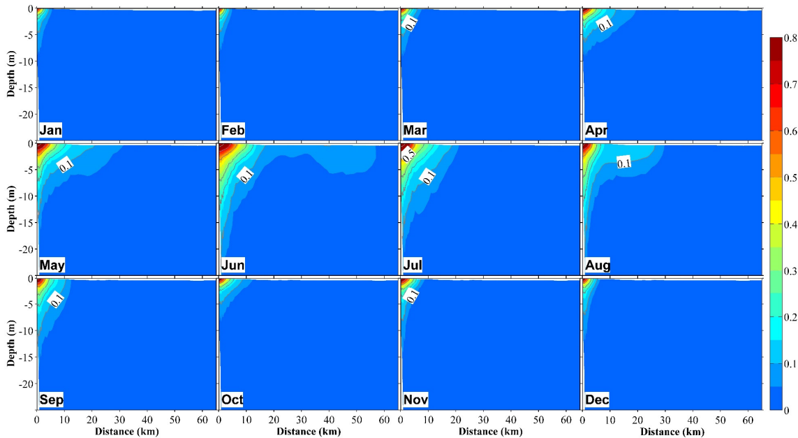
Figure 98: Vertical distribution at section S2 (Figure 1b) of the ratio of dissolved inorganic nitrogen originating from river water (DIN RV ) to the total DIN in 12 months. The distance on the x-axis is measured from the shore.
