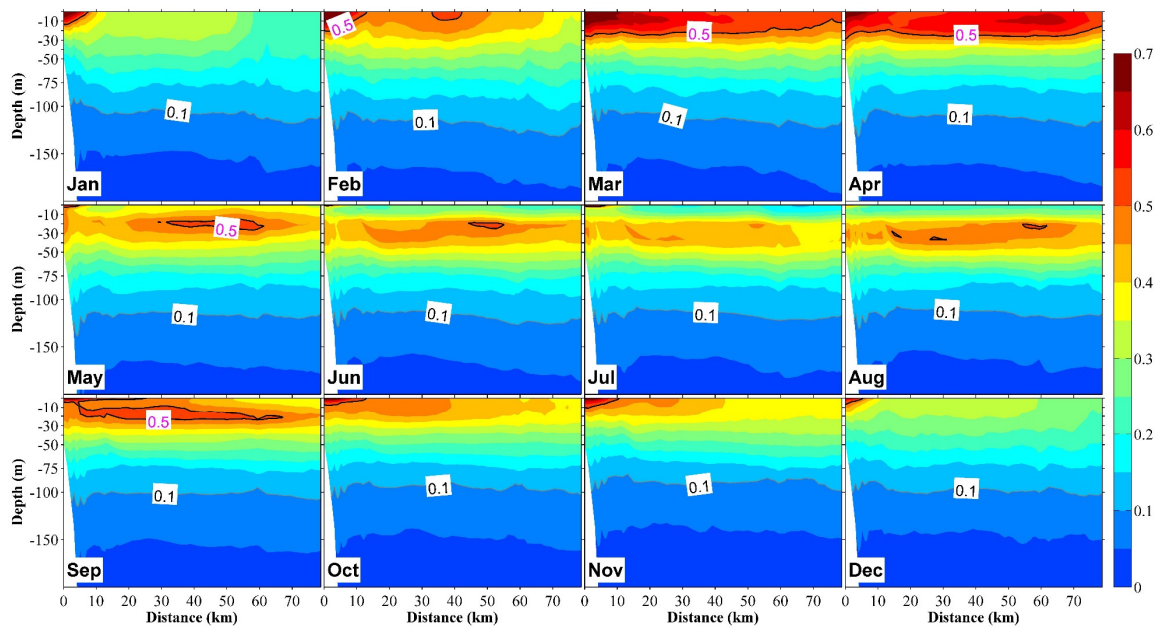
Figure 87: Vertical distribution at section S2 (in Figure 1b) of phytoplankton in 12 months, with the unit in \text{mmolN m}^{-3} . The distance on the x-axis is measured from the shore.
