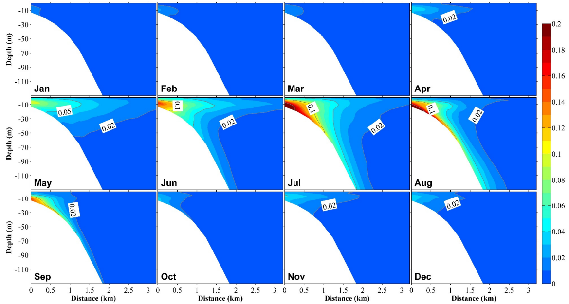
Figure 124: Vertical distributions at section S3 (Figure 1b) of the proportions of phytoplankton supported by nutrients originating from submarine groundwater discharge ( \text{PHY}_{\text{SGD}} ) to the total phytoplankton in 12 months. The distance on the x-axis is measured from the shore.
