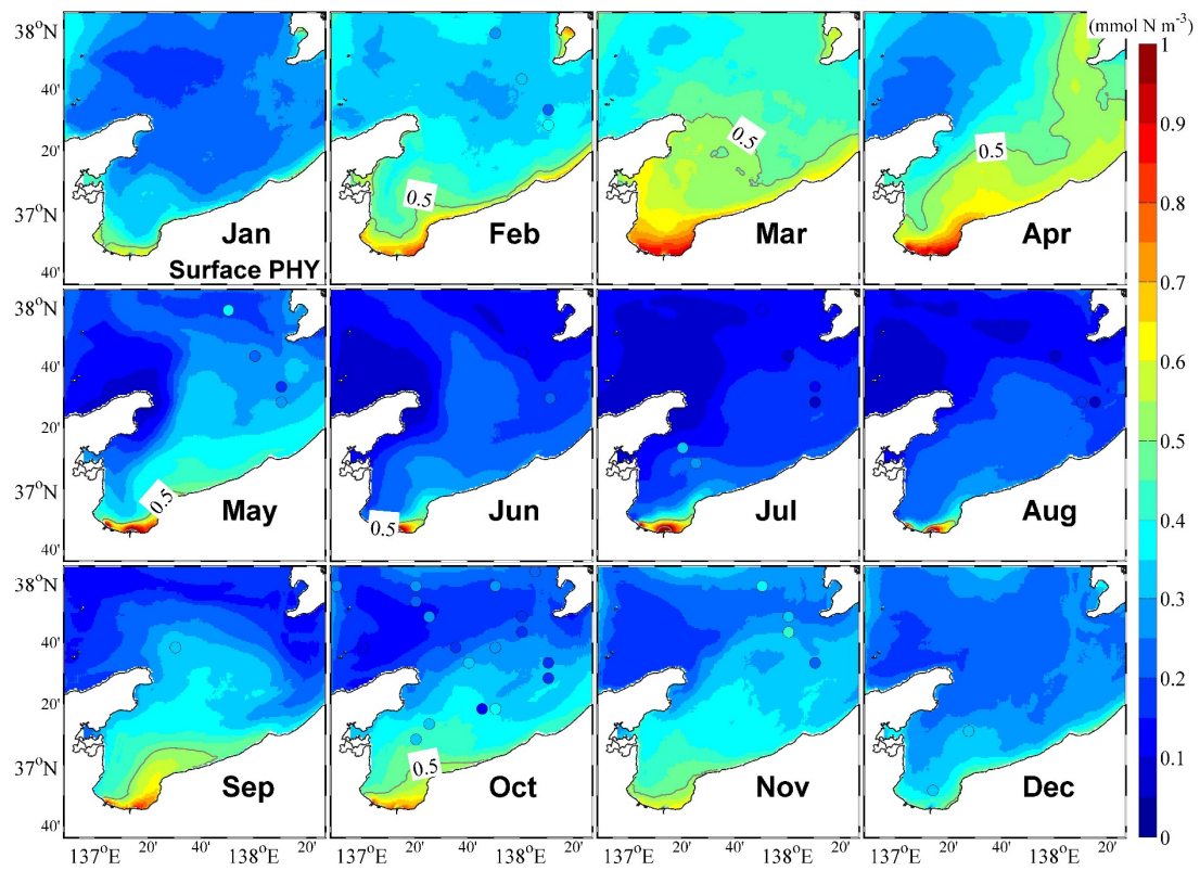
Figure 76: Monthly mean surface phytoplankton concentrations. The color circles represent observational data.
