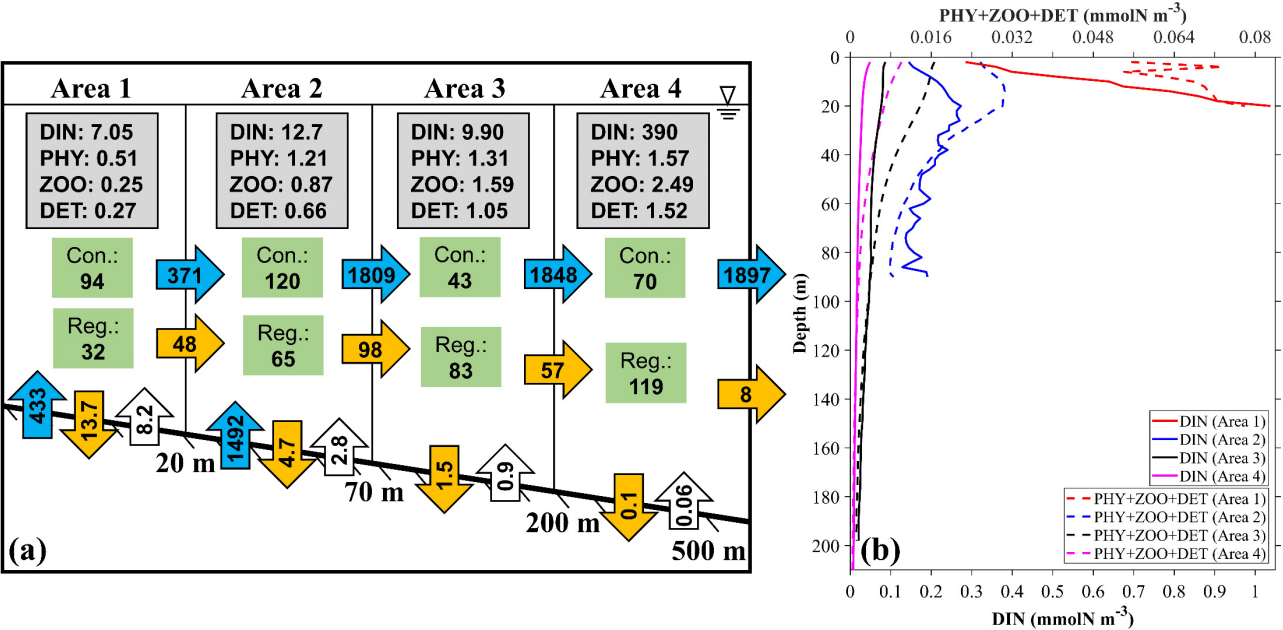
420 Figure 143: (a) The annual mean inventories and material flows of SGD-derived nutrients in 4 different areas near the outlet locations of SGD (Figure 1c). (Area 1) 0–20 m, (Area 2) 20–70 m, (Area 3) 70–200 m, (Area 4) 200–500 m. The values in the grey rectangles represent the inventory (×10 7 mmol) of the ecosystem variables in the area. The values in the green rectangles represent the consumption (Con.) and regeneration (Reg.) rates of DIN GW in the biogeochemical processes (mmol s -1 ). The values in the vertical
