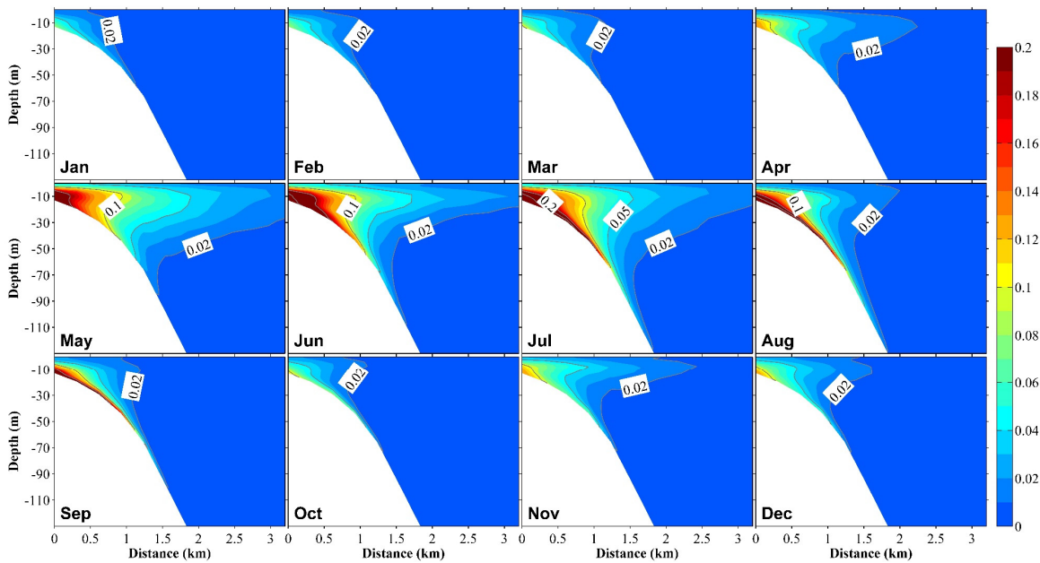
Figure 109: Vertical distributions at section S3 (Figure 1b) of the ratio of dissolved inorganic nitrogen originating from submarine groundwater discharge ((DIN SGD ) to the total DIN in 12 months. The distance on the x-axis is measured from the shore.
