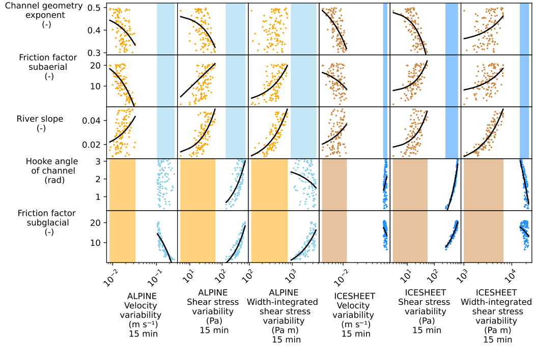
Figure 6. Parameter values compared to variability in model outputs. Plots on the left (orange, light blue) correspond to the ALPINE case. Plots on the right (brown, dark blue) correspond to the ICESHEET case. Outputs are shown using 15 minute smoothing time. Linear trends are denoted in black if they are significant at p \geq 0.01 . To compare the range of model outputs for the subaerial and subglacial cases, shaded areas show the range of model outputs that are independent of the parameter values.
