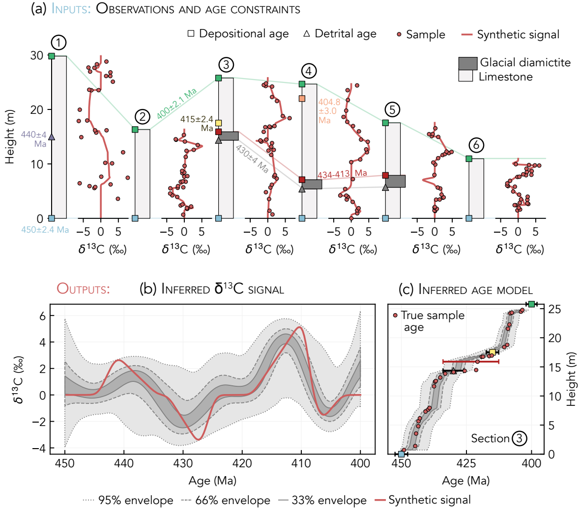
Figure 8. Testing the inference model using synthetic data. (a) Age-constraint-prior-distributions, stratigraphic Stratigraphic sections -with age constraints and \delta^{13}\text{C} observations. (b) \delta^{13}\text{C} signal inference using the age constraints and \delta^{13}\text{C} observations in a, with the synthetic \delta^{13}\text{C} signal plotted for comparison. The 95% envelope marks the 2.5th and 97.5th percentiles of the posterior \delta^{13}\text{C} distribution for each time step, the 66% envelope marks the 17th and 83rd percentiles, and the 33% envelope marks the 33.5th and 66.5th percentiles. (c) Posterior age model for section 3, with samples plotted by their true age.
